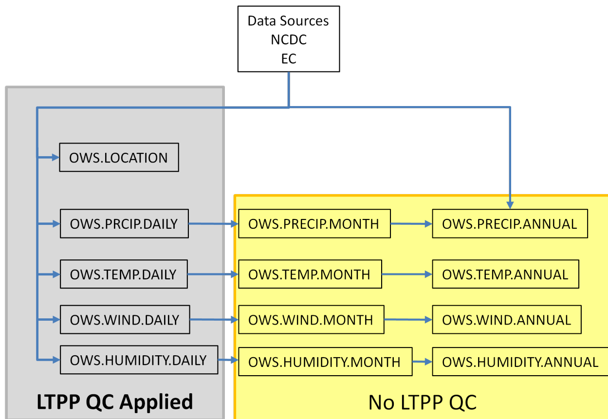
Figure 5. Structure and relationship between the CLM_OWS_* tables.
