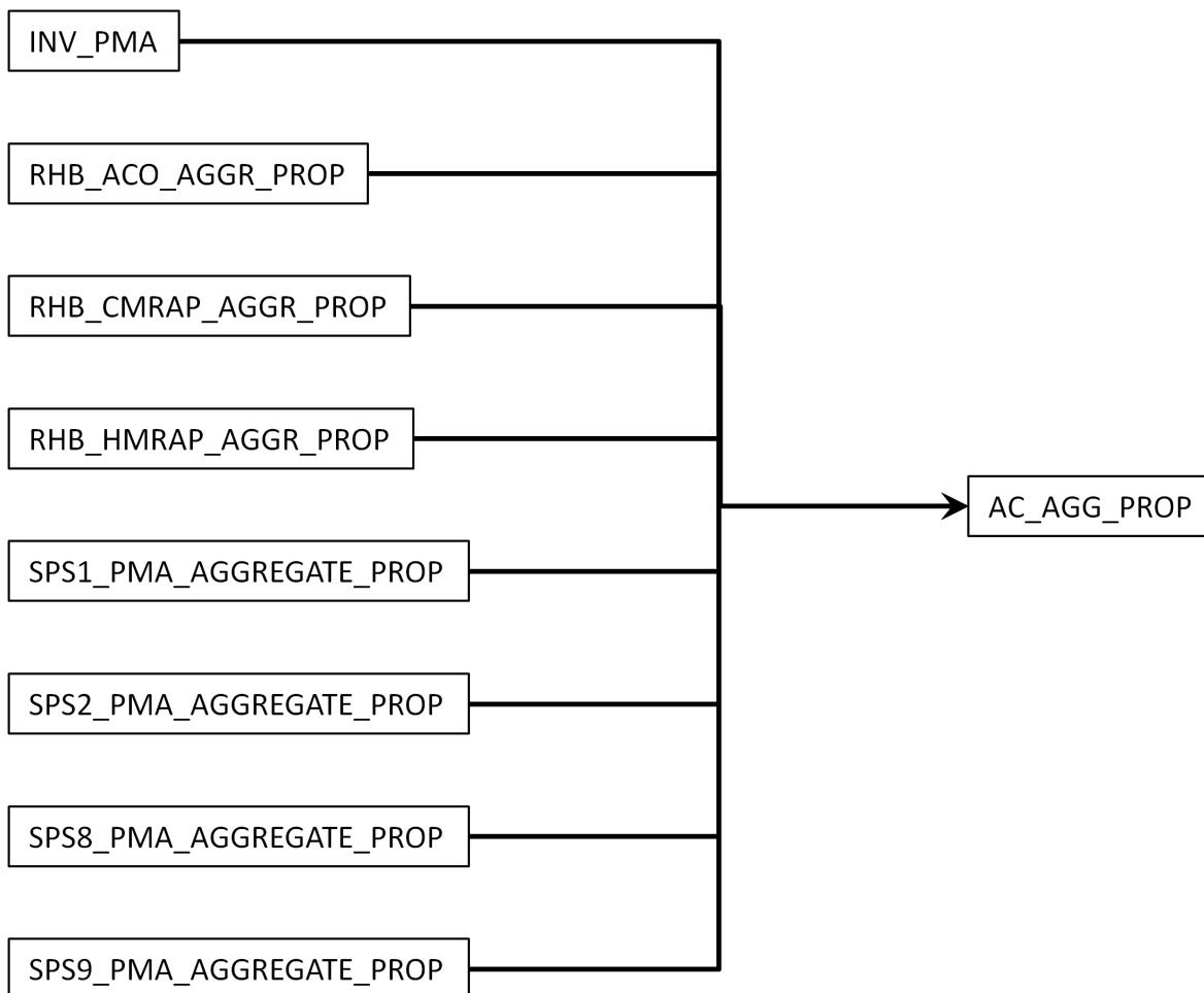
Figure 20. Source tables for the AC_AGG_PROP table included in the DCV module.
