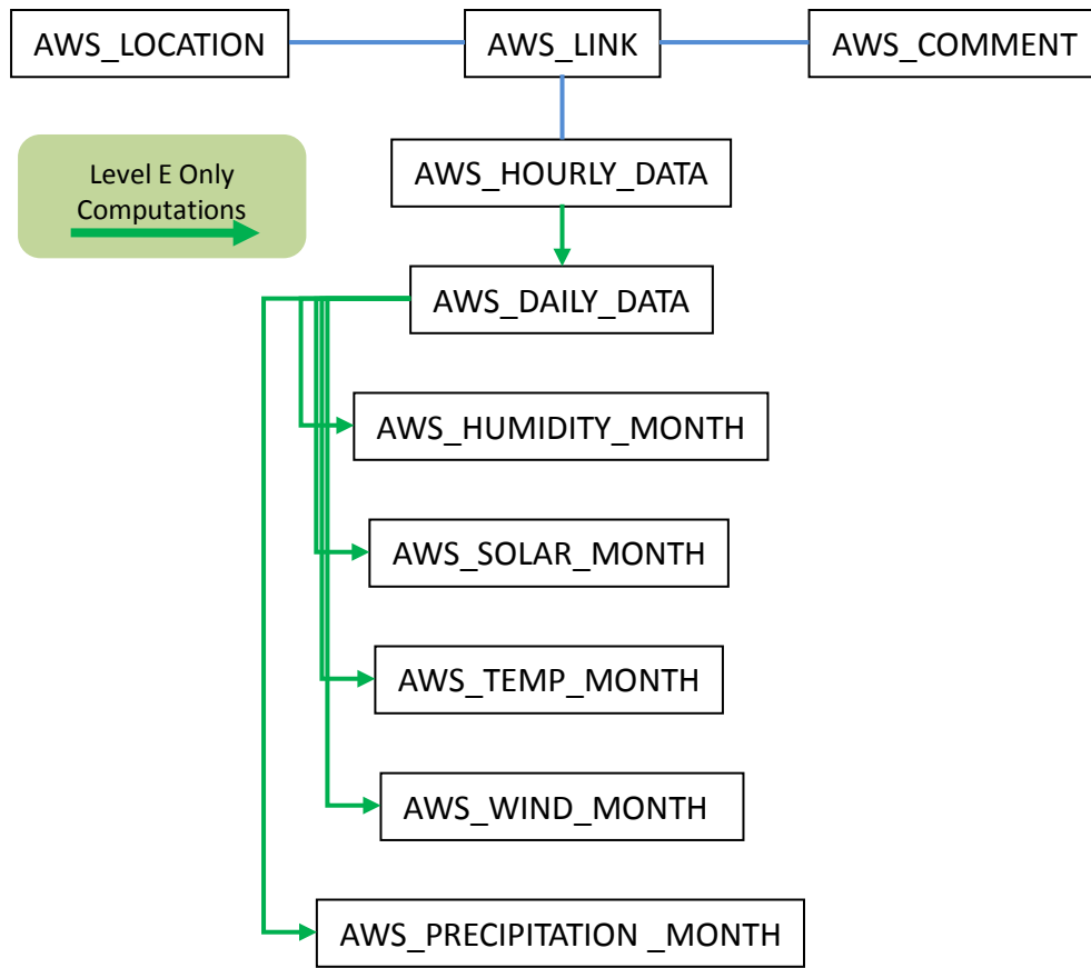
Figure 4. Organization and computational relationships between the AWS tables.
