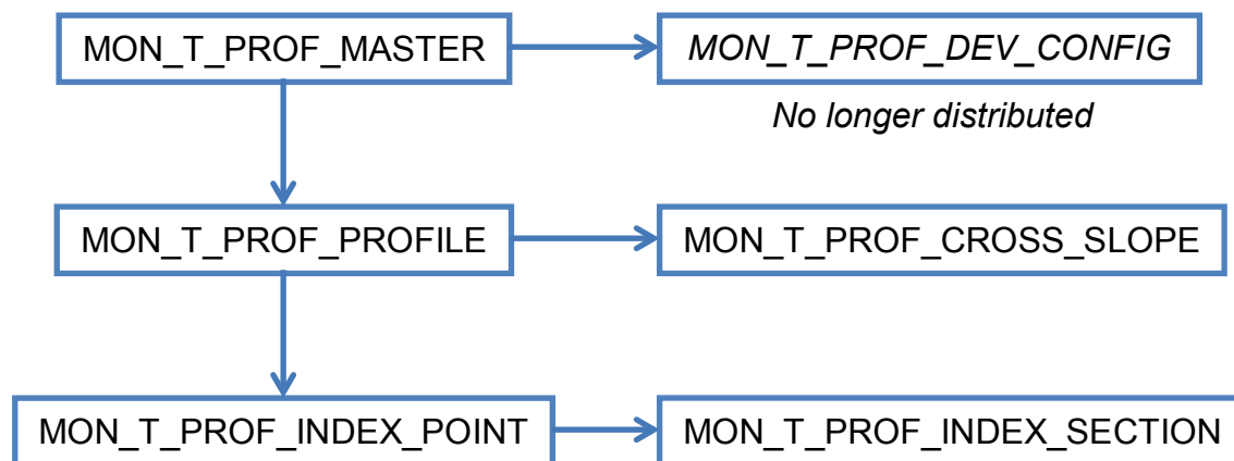
Figure 12. Relational structure between tables in the MON_T_PROF module.
