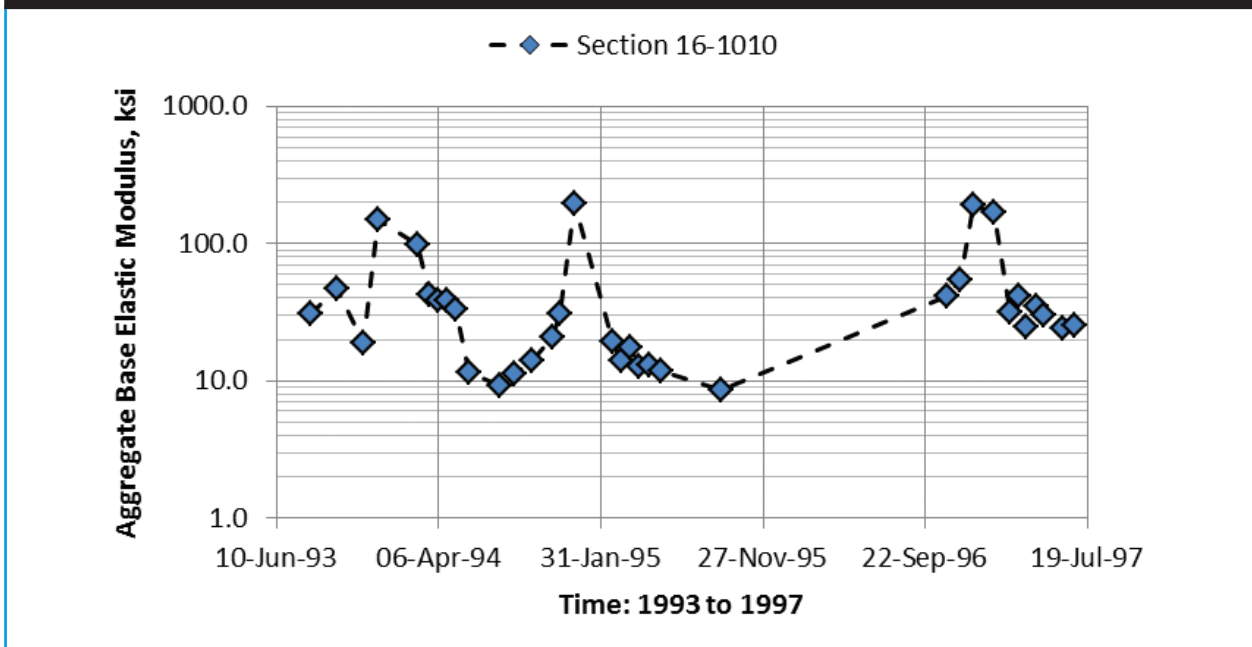
Figure 5. Idaho SMP project.
