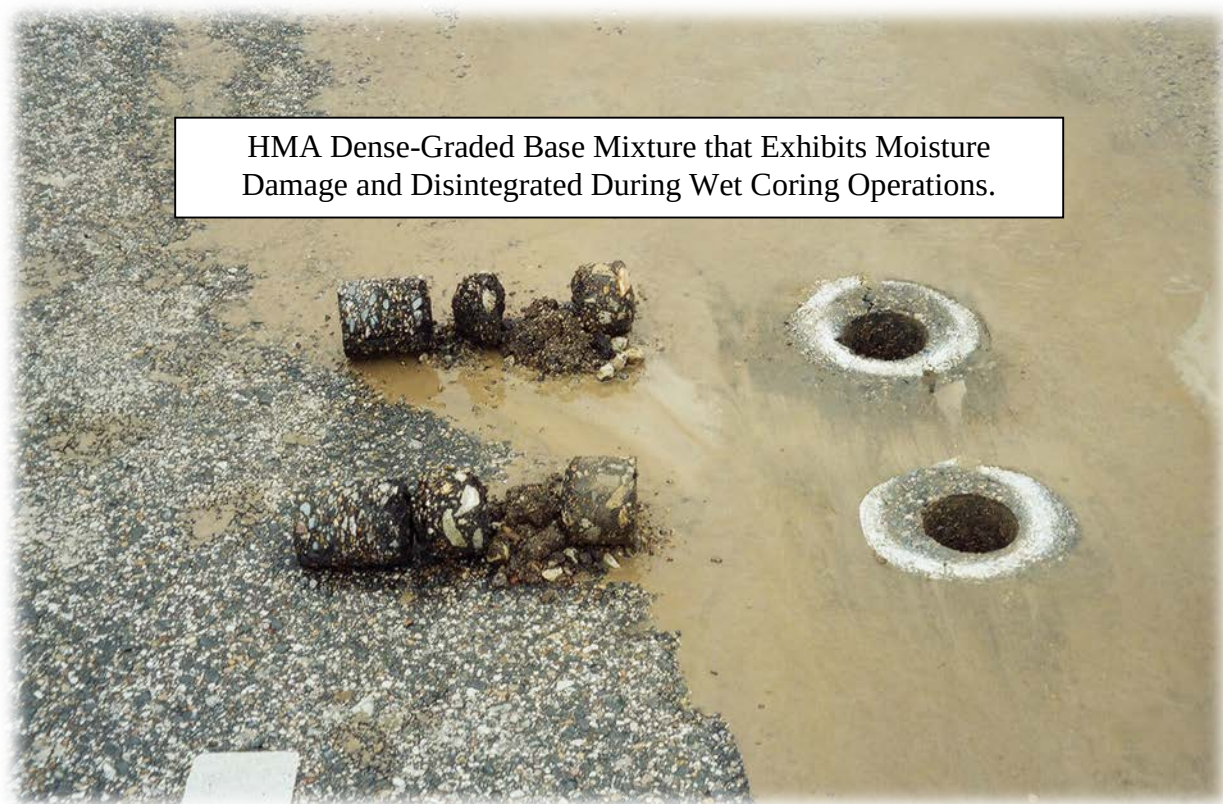
Figure 34. Photo. Cores recovered where moisture damage occurred, decreasing the in-place modulus of the layer/mixture (Texas SPS-5 project).
