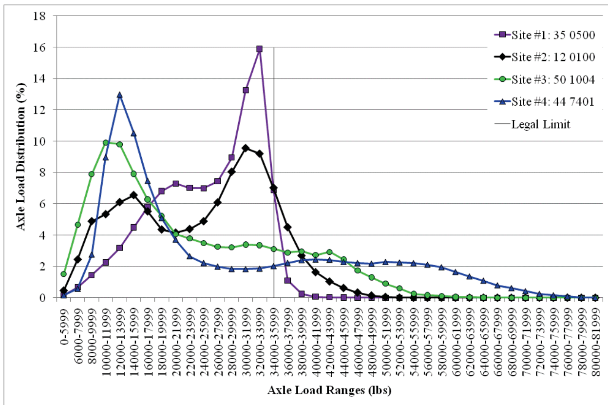
Figure 7. Graph. Tandem NALS for class 9 vehicles for four LTPP sites.
