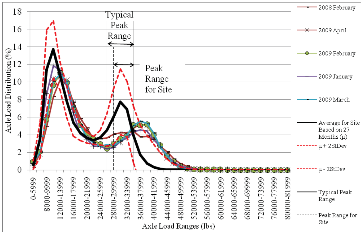
Figure 32. Graph. Monthly NALS for tandem axes for site 26-0100 class 9 trucks.
