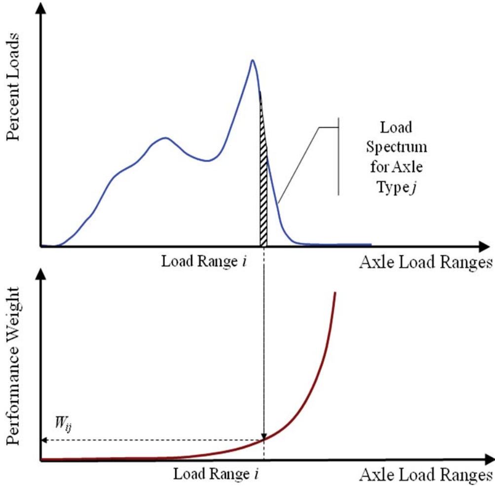
Figure 13. Graph. Estimation of parameters for PWLE.
