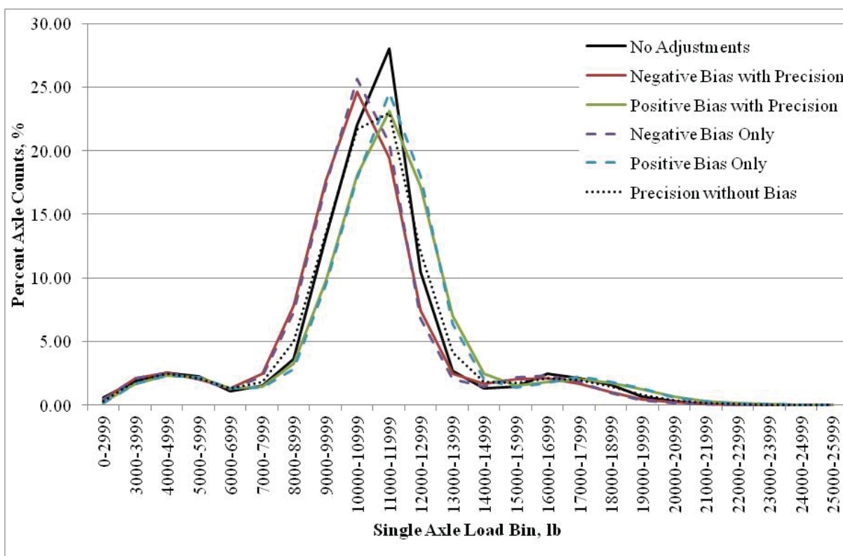
Figure 21. Graph. Example of biased single axle load spectra for class 9 vehicles.
