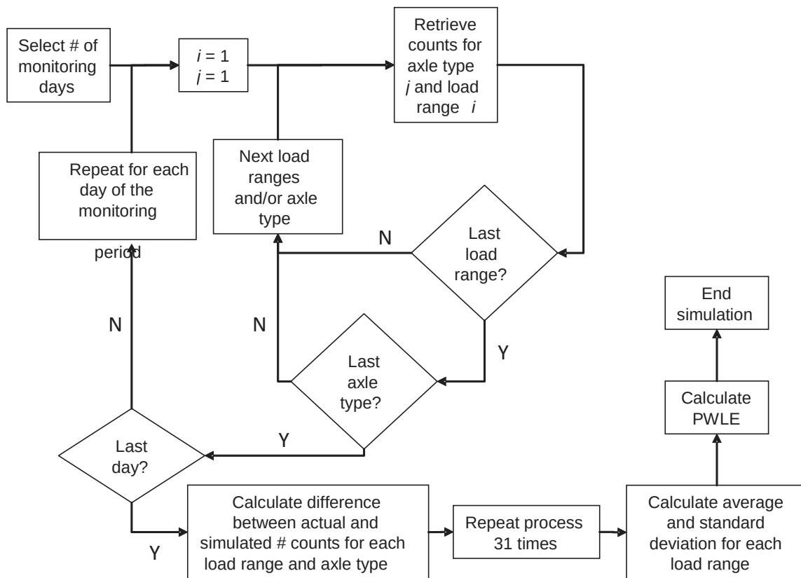
Figure 14. Flowchart. Monte Carlo simulation for analysis of data availability.
