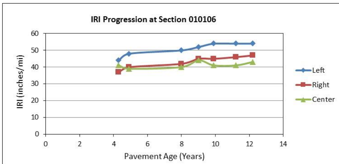
Figure 12. Graph. IRI progression at section 010106.
