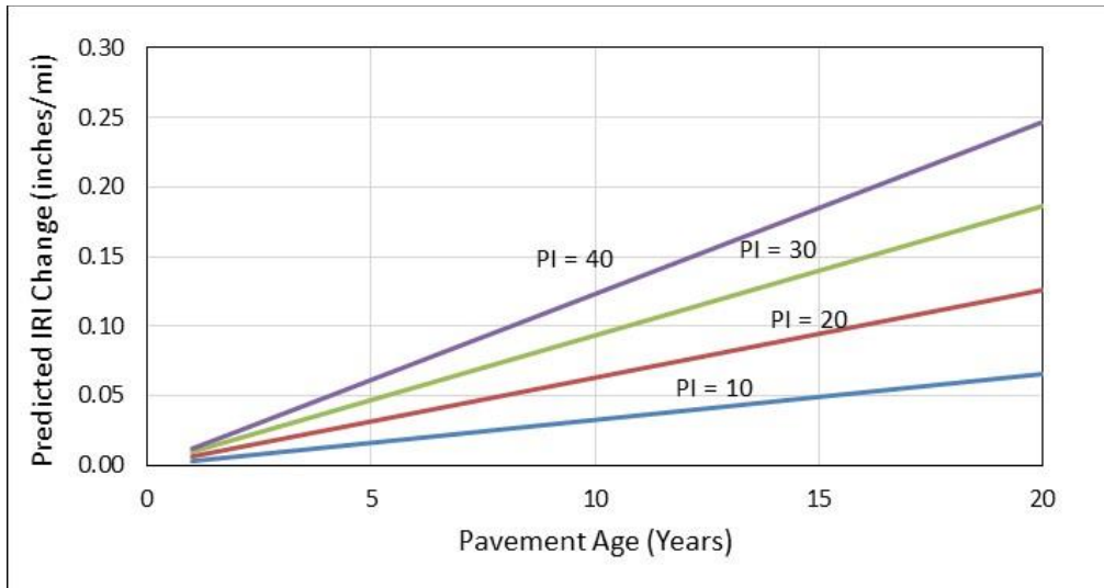
Figure 4. Graph. Increase in IRI due to PI of subgrade predicted by the MEPDG model for four different PI values.
