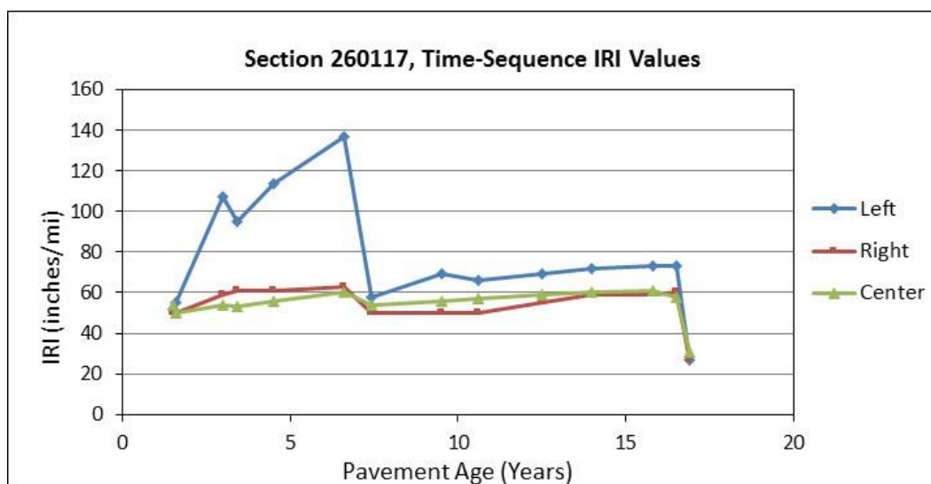
Figure 19. Graph. Time-sequence IRI values at section 260117.
