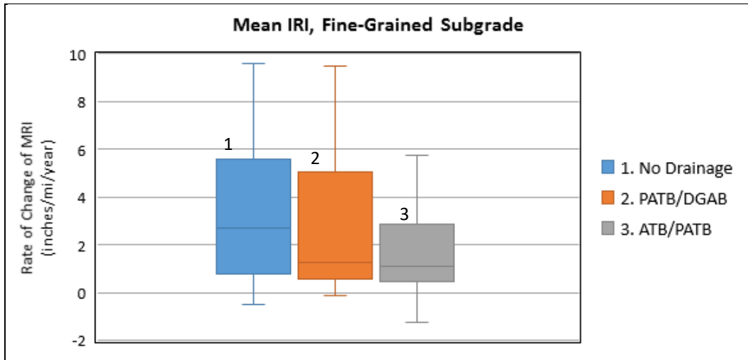
Figure 93. Graph. Box plots showing the rate of change of MIRI for sections on fine-grained subgrade, categorized according to type of drainage.
