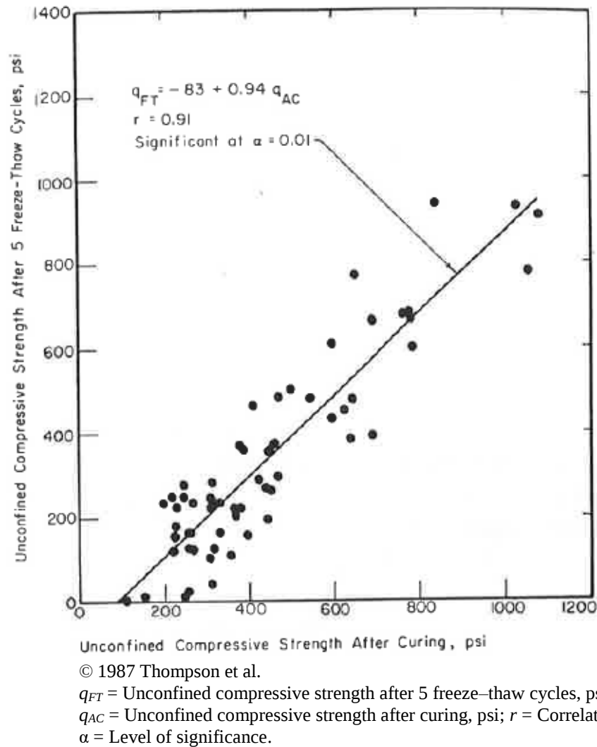
Figure 2. Graph. Relationship between strength of cured cement-stabilized materials and cement-stabilized materials subjected to freeze-thaw cycles. (35)
