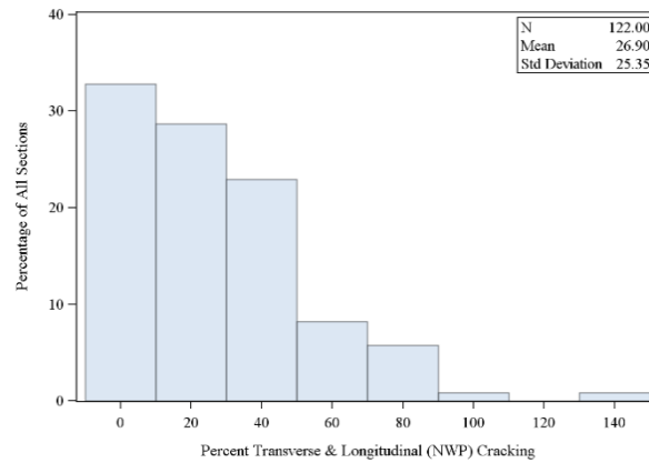
Figure 165. Graph. Distribution of transverse and longitudinal (non-wheel path) cracking for AC pavements after 15 yr in service.
