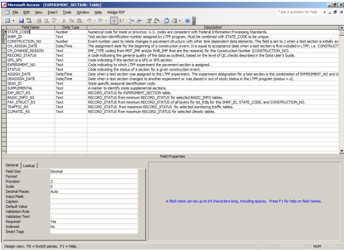
Figure 6. Screenshot. Design view of EXPERIMENT_SECTION Table.
