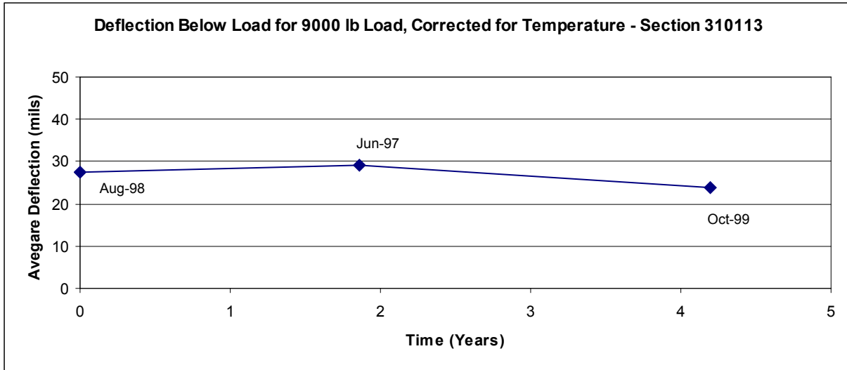
Figure 138. Graph. Average normalized deflection below 9,000-lb load, section 310113 (Nebraska).
