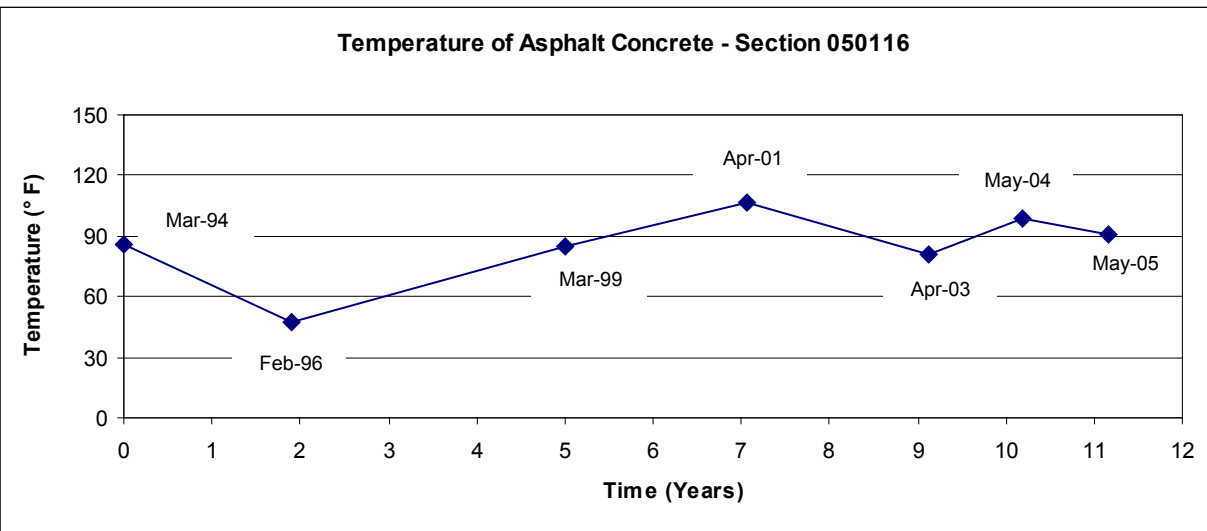
Figure 163. Graph. Mid-depth temperature of AC layer, section 050116 (Arkansas).
