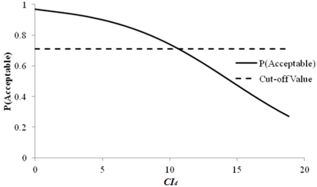
Figure 85. Graph. Sensitivity of transverse cracking acceptable probability to deflection parameter CI_4 for rigid pavements (12,000 lb (5,445 kg)).
