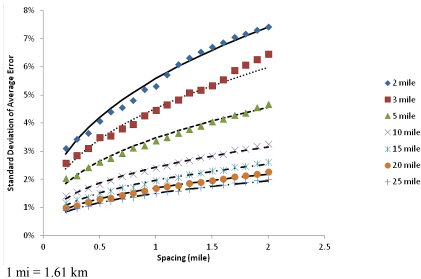
Figure 50. Graph. Observed standard deviation (data points) plotted with the computed average error (lines).
