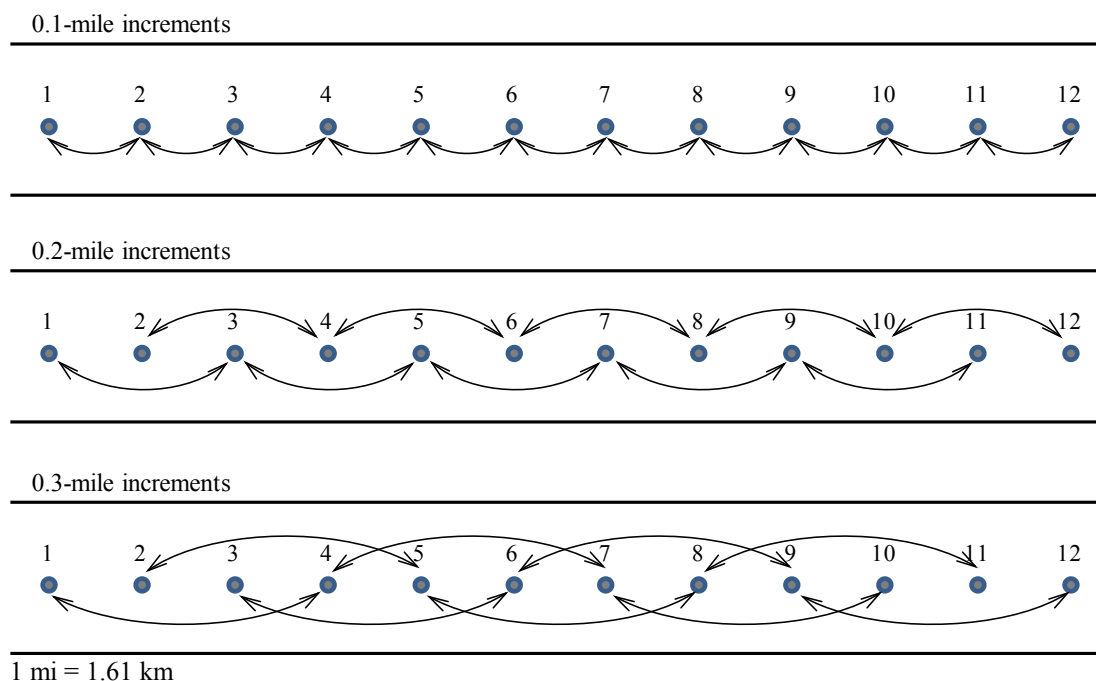
Figure 39. Illustration. Deflection measurement pairings based on 0.1-, 0.2-, and 0.3-mi (0.161-, 0.322-, and 0.483-km) spacings.
