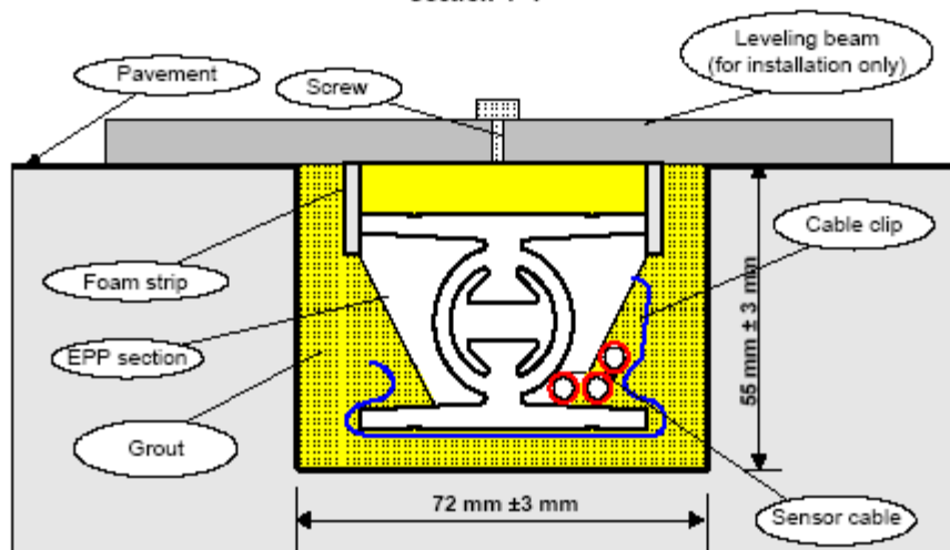
Section 1-1
