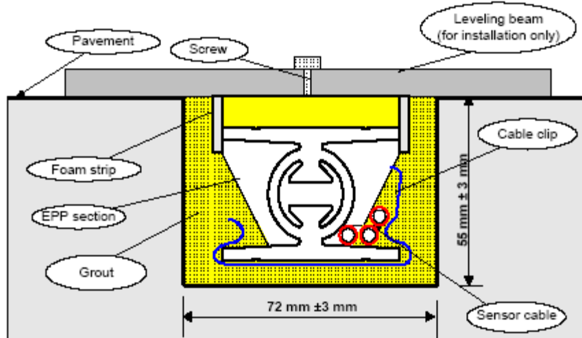
Section 1-1
