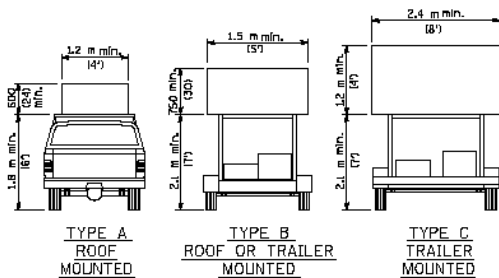
ARROW BOARDS
