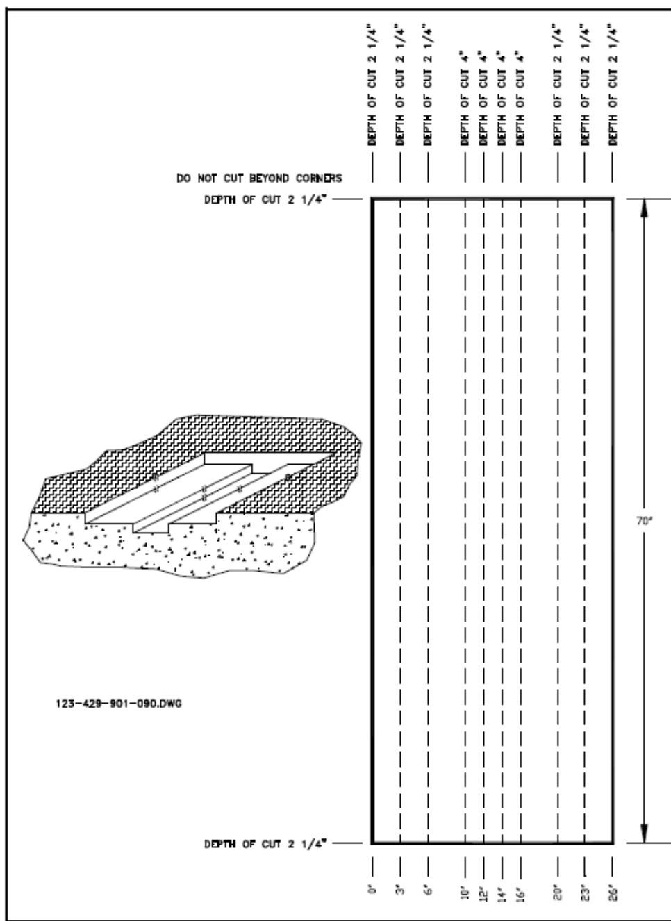
Figure 5 - Frame Recess Cutting Diagram
