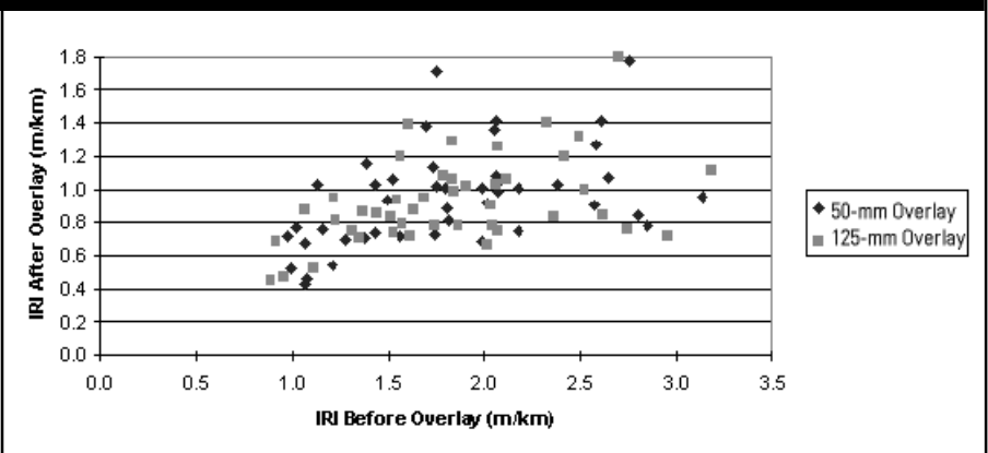
Figure 3. IRI before and after overlay.
