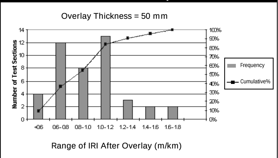
Figure 4. Frequency distribution of IRI after overlay for sections that received a 50-mm overlay.
