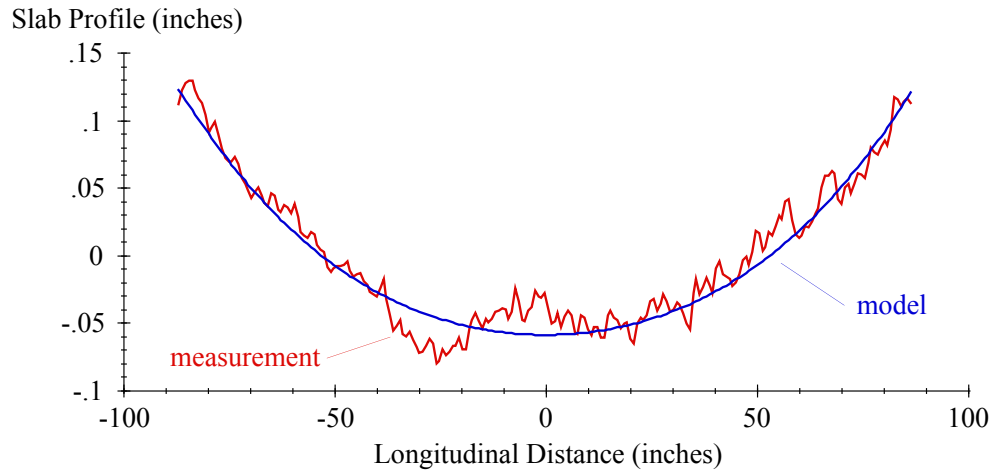
Figure 1. Example curve fit for estimation of PSG.
