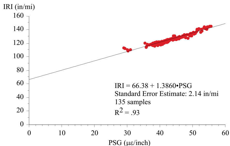
Figure 2. IRI versus PSG for right side of section 0215.
