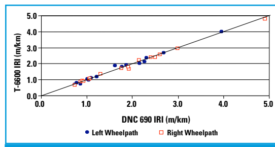
Figure 2. This chart shows the relationship between the IRI values for the K.J. Law Engineers DNC 690 and T-6600 profilers.
