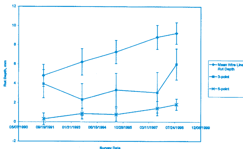
Figure 5. Example from section 21001 of the average rut depth and standard deviation measured over time (the bars represent \pm 1 standard deviation).
