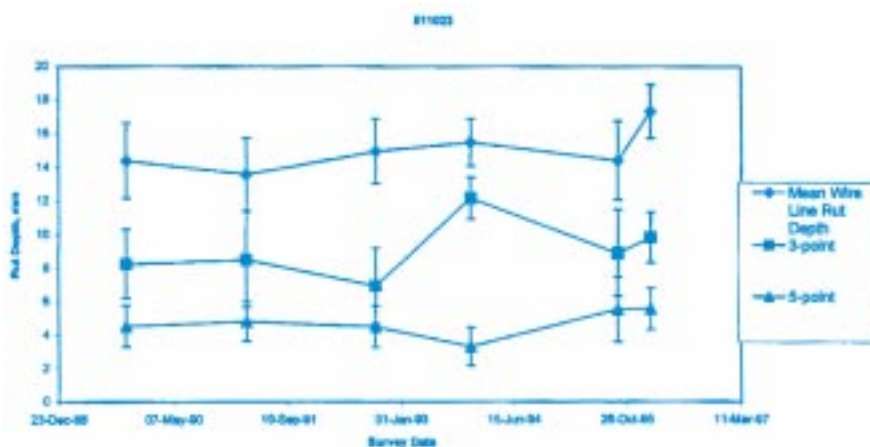
Figure 6. Example from section 511023 of the average rut depth and standard deviation measured over time (the bars represent \pm 1 standard deviation).
