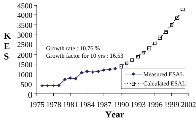
Figure 12. Measured ESAL and predicted ESAL
