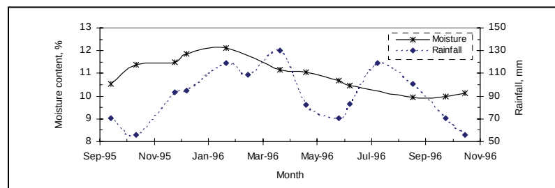
Figure 7. Moisture content and rainfall versus season for clayey soil, site 13-1005
