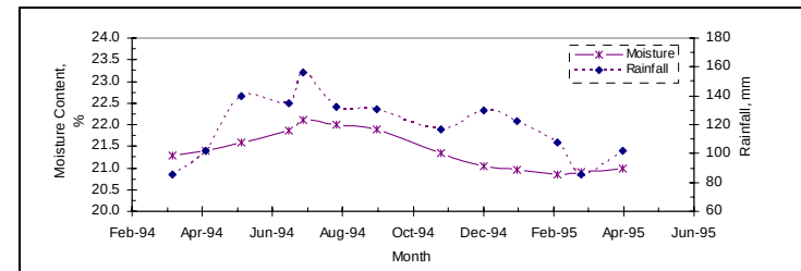
Figure 8. Moisture content and rainfall versus season for clayey soil, site 48-4143
