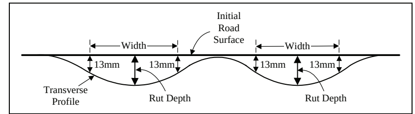
Figure 1. A schematic diagram for the measurement of rutted widths and rut depths from LTPP transverse profile data
