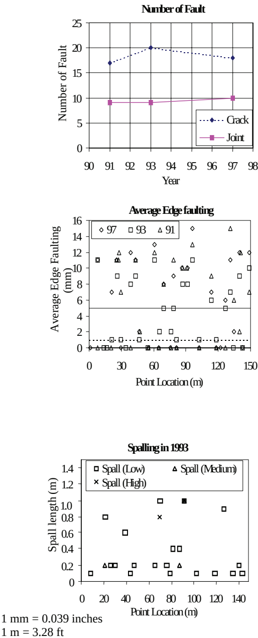
Figure 2. Distress progression as a function of time
