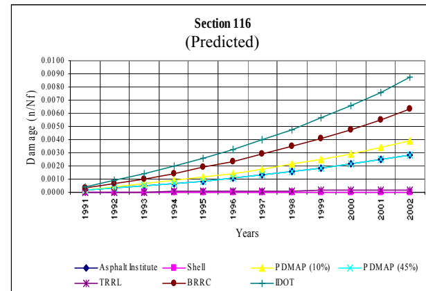
Figure 18. Example of observed and predicted fatigue cracking
