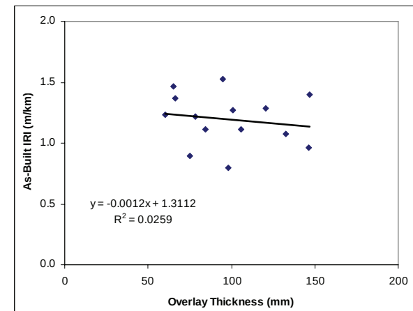
Figure 4. As-built roughness versus overlay thickness for C-LTPP data
