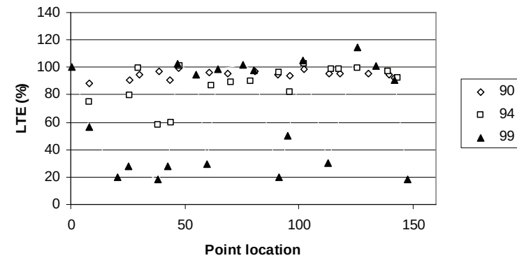
Figure 10. LTE versus point location (J4)
