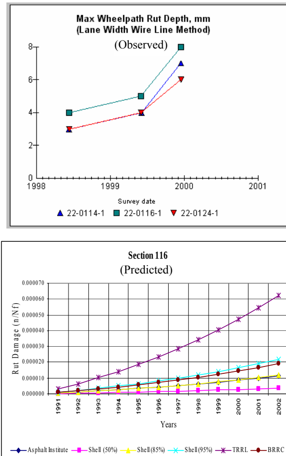
Figure 19. Example of observed and predicted rutting
