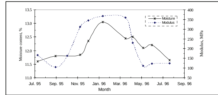
Figure 4. Moisture content and elastic modulus versus season for silty sand, site 28-1016
