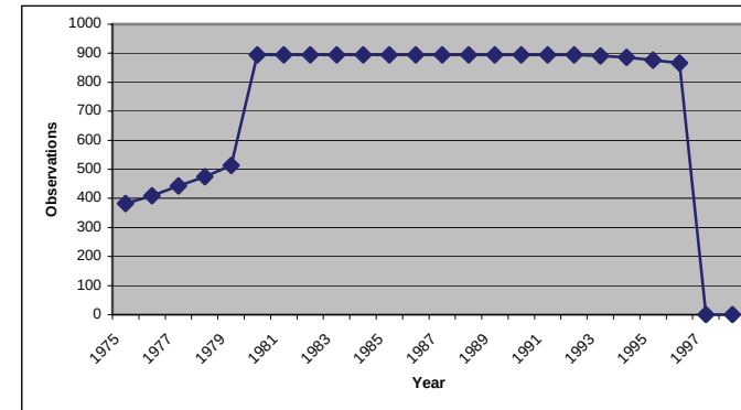
Figure 1. The number of text sections having climate records each year.
