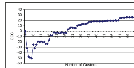
Figure 3. CCC versus number of clusters (Type I data)
