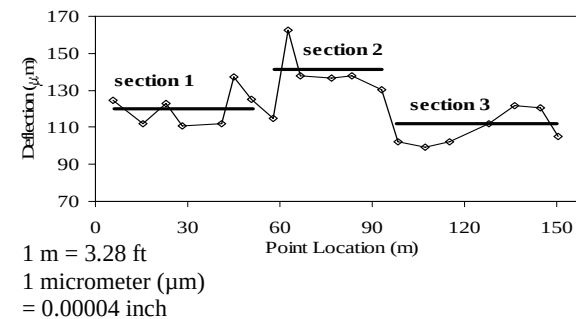
Figure 6. Deflection profile as function of distance
