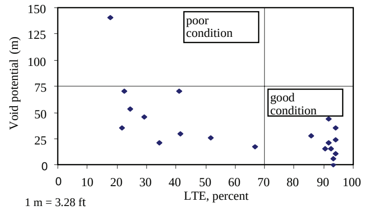
Figure 11. Relationship between LTE and void ratio
