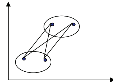
Figure 2. Distance measurement of the average linkage clustering method
