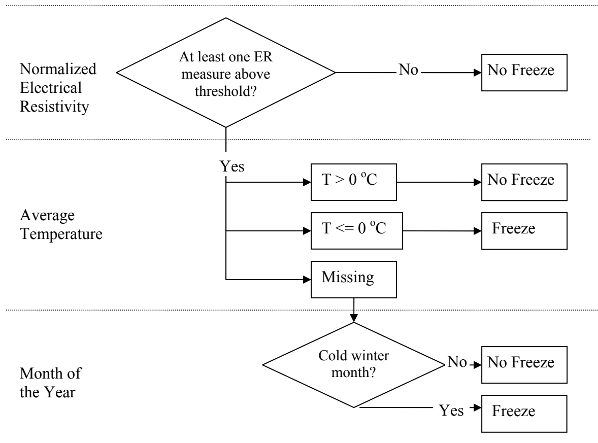
Figure 2. Chart. Previous FROST decision tree.
