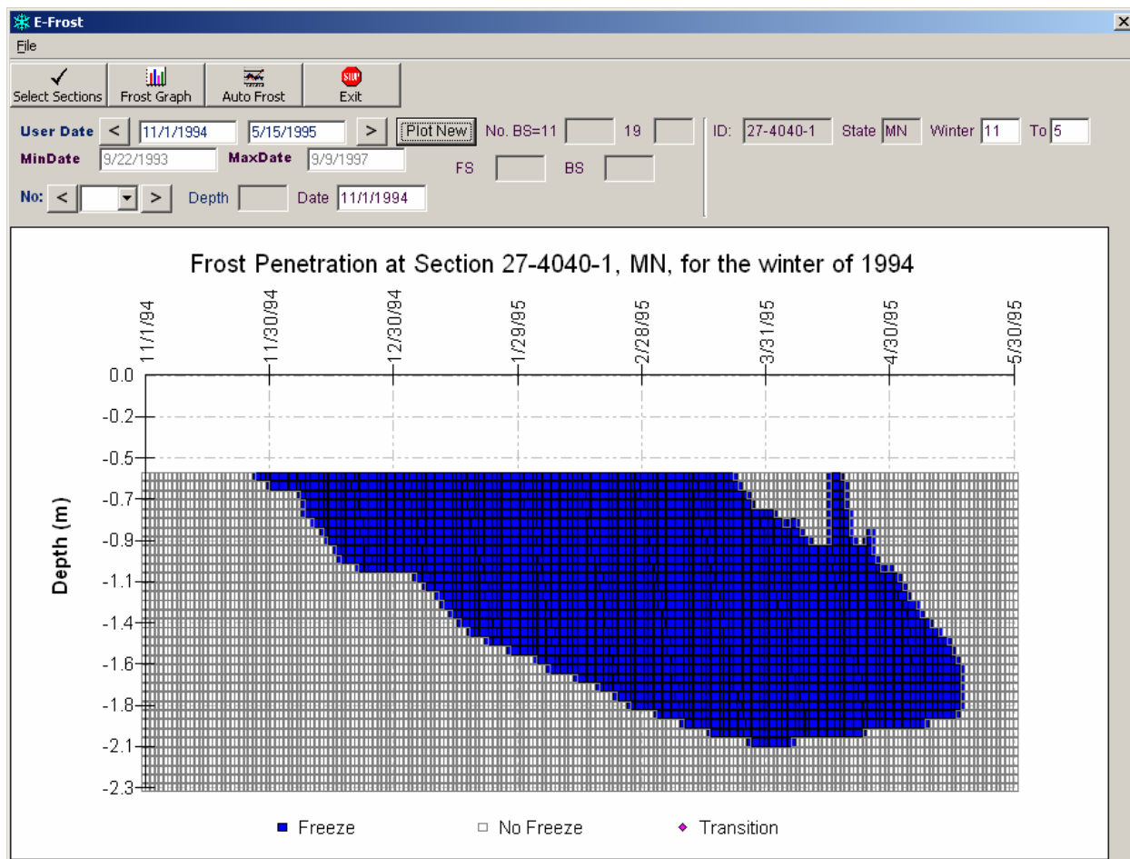
Figure 23. Chart. Frost penetration profile showing solid freeze with partial spring thaw and refreeze.
