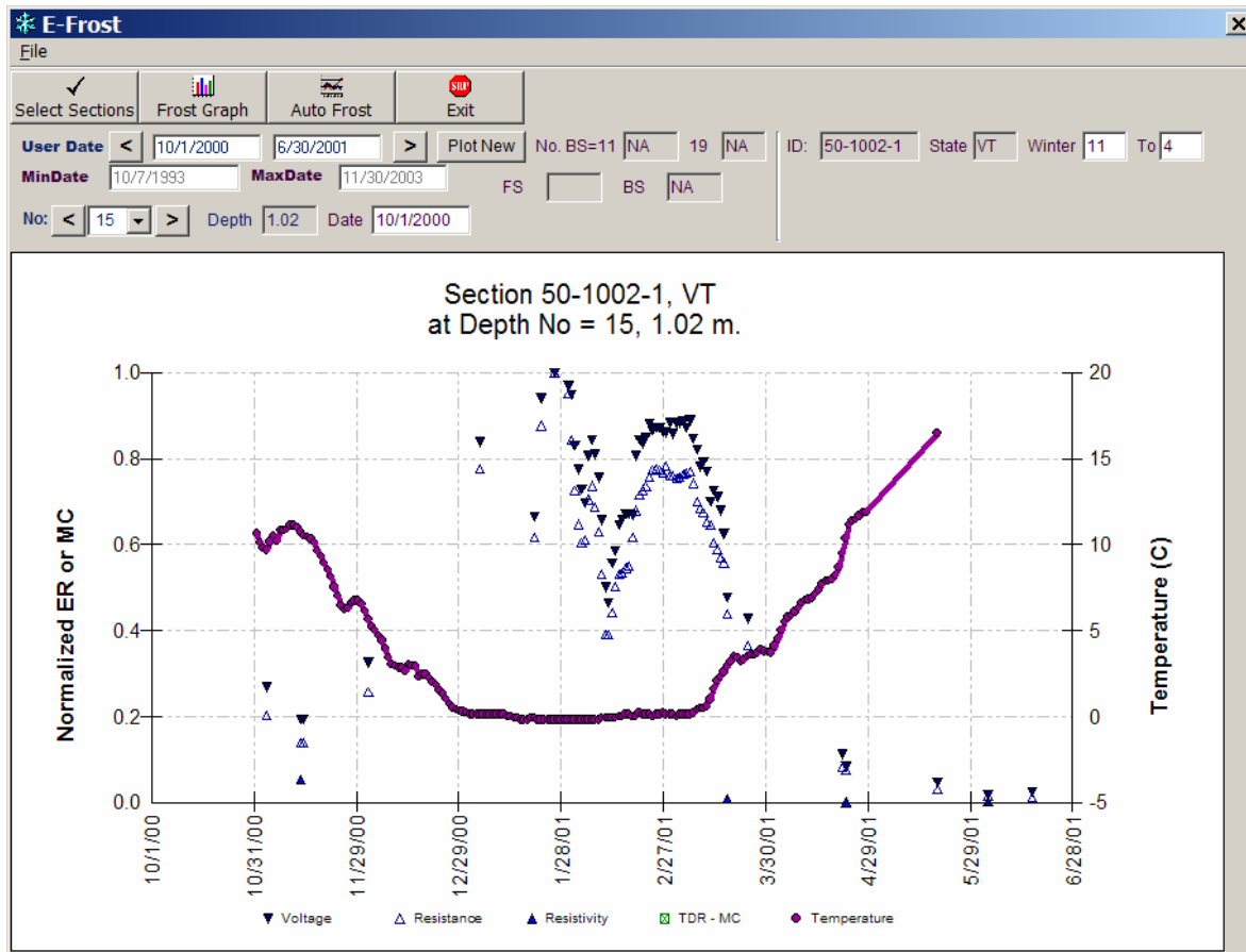
Figure 19. Chart. Temperature and ER trends at 1.02 m (3.35 ft) for site 50-1002 during winter season 2000–2001.
