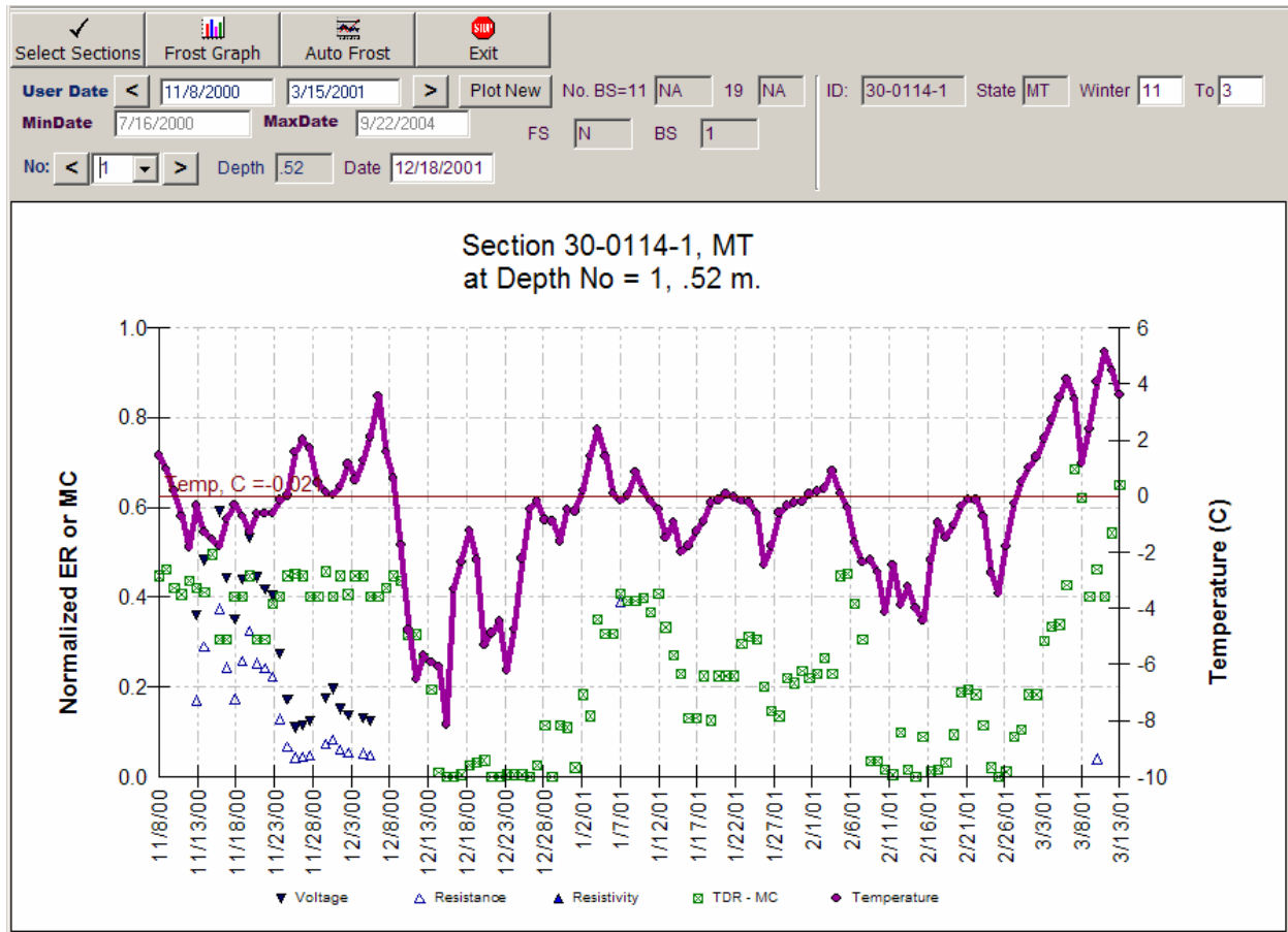
Figure 4. Chart. Comparison of ER, temperature, and moisture trends for section 0114 in Montana.
