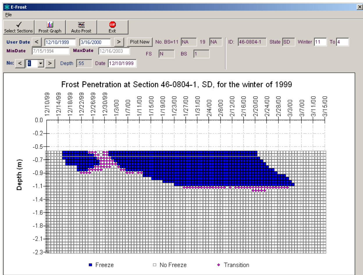
Figure 35. Chart. Final frost penetration profile for SMP site 46-0804 for the winter of 1999.
