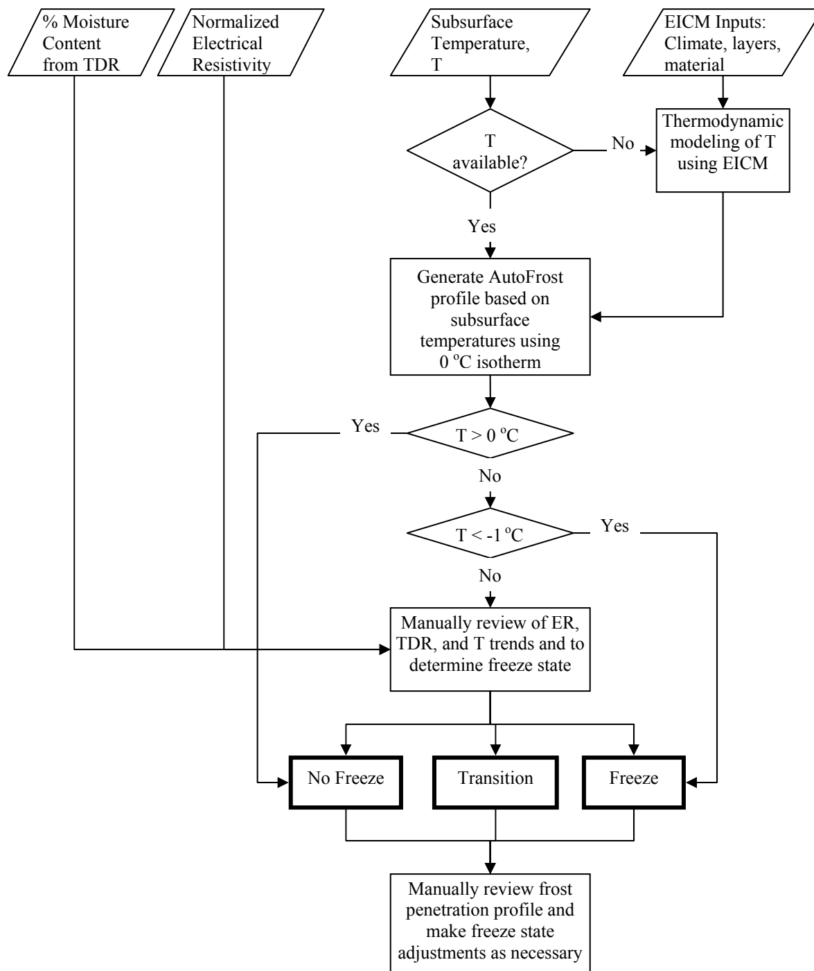
Figure 15. Chart. Enhanced FROST algorithm.
