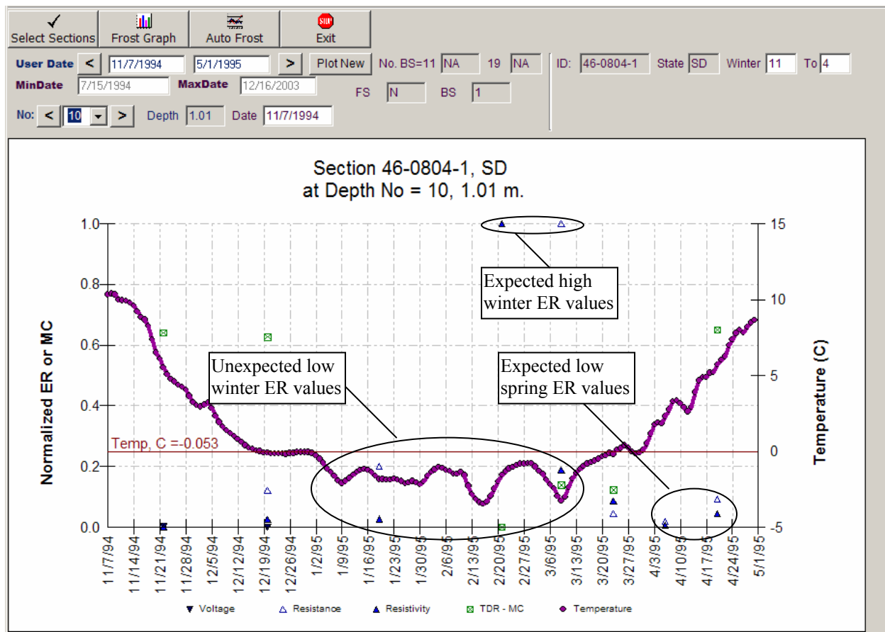
Figure 7. Chart. Comparison of ER, temperature, and moisture trends for section 0804 in South Dakota at 1.01 m (3.31 ft) depth.
