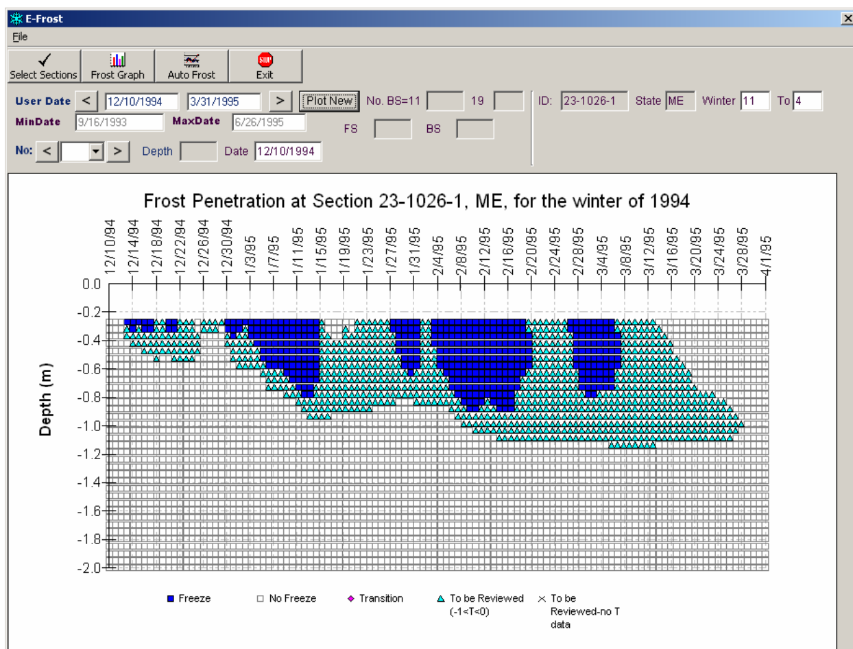
Figure 8. Chart. Frost predictions for section 1026 in Maine.
