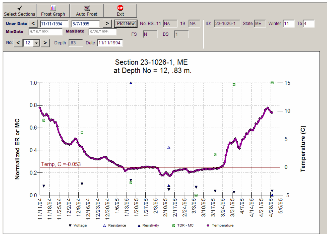
Figure 9. Chart. Comparison of ER, temperature and moisture trends for section 1026 in Maine.
