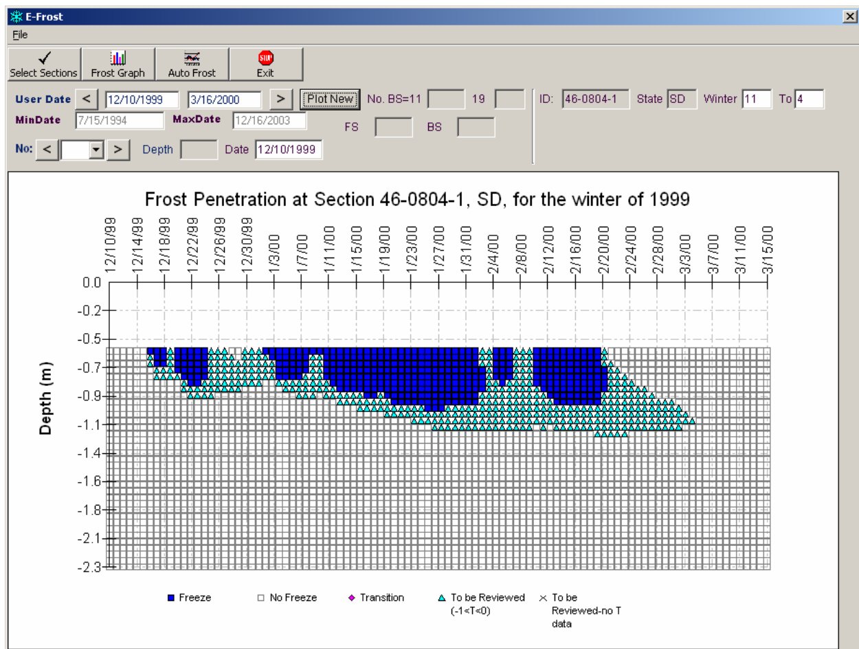
Figure 33. Chart. Automatically generated frost penetration profile at SMP site 46-0804 for the winter of 1999.
