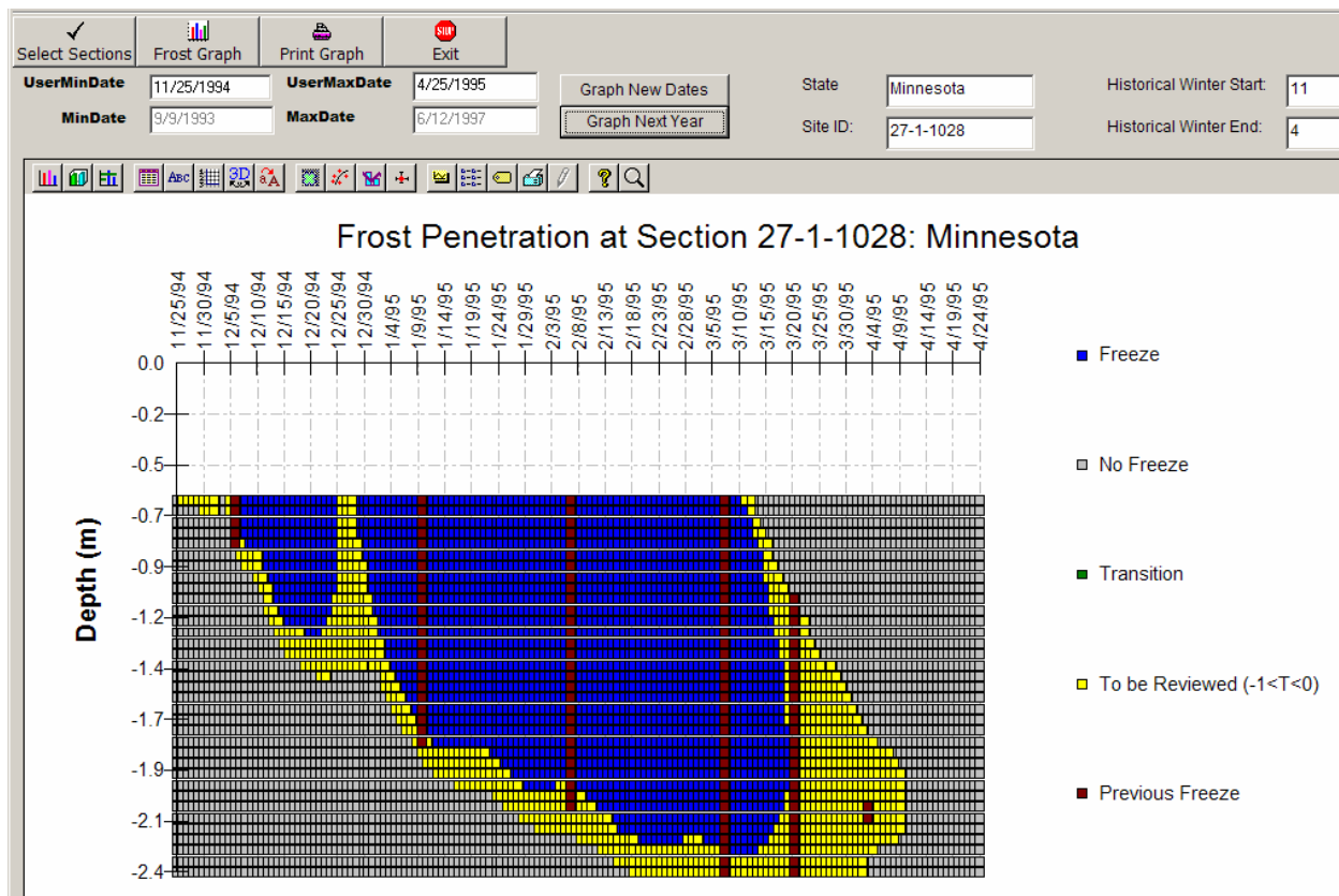
Figure 5. Chart. Frost predictions for section 1028 in Minnesota.
