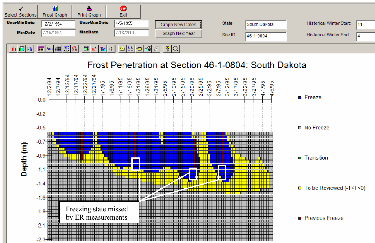
Figure 6. Chart. Frost predictions for section 0804 in South Dakota for 1994–1995 winter season.
