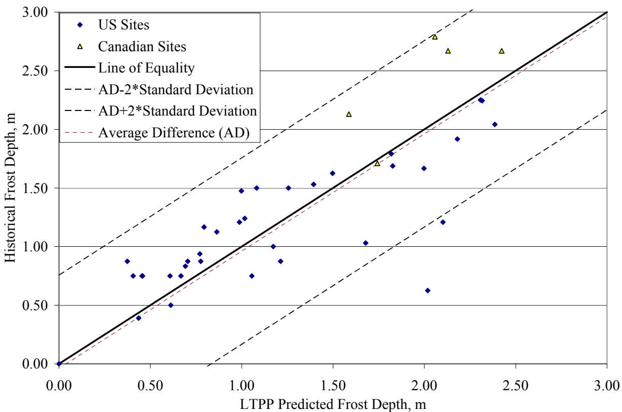
Figure 24. Graph. Comparison of frost penetration depths.
