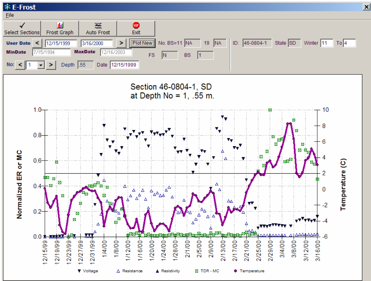
Figure 34. Chart. Time series plot for SMP site 46-0804 for the winter of 1999 at analysis depth = 0.55 m (1.8 ft).
