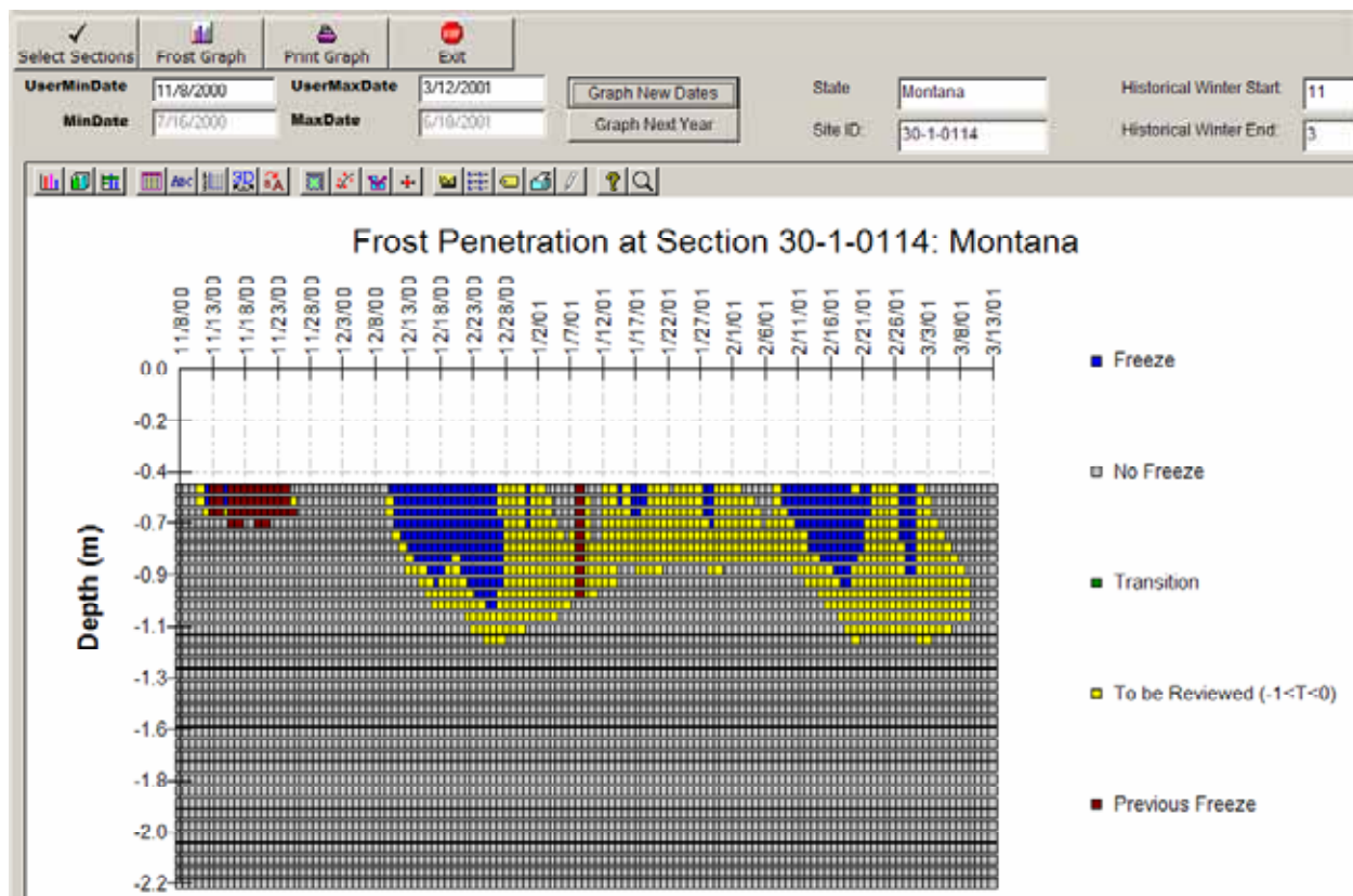
Figure 3. Chart. Frost predictions for section 0114 in Montana.
