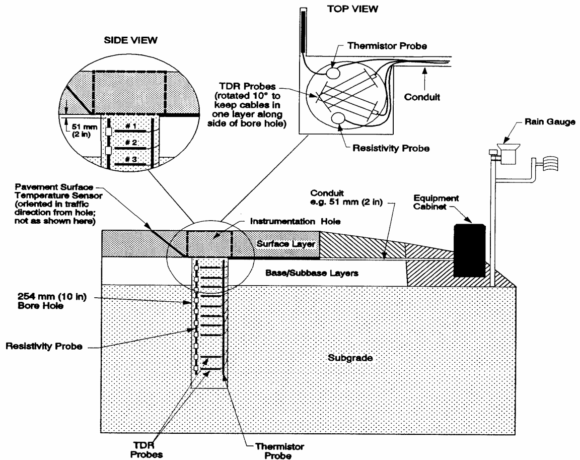
Figure 1. Illustration. LTPP SMP instrumentation layout. (4)
