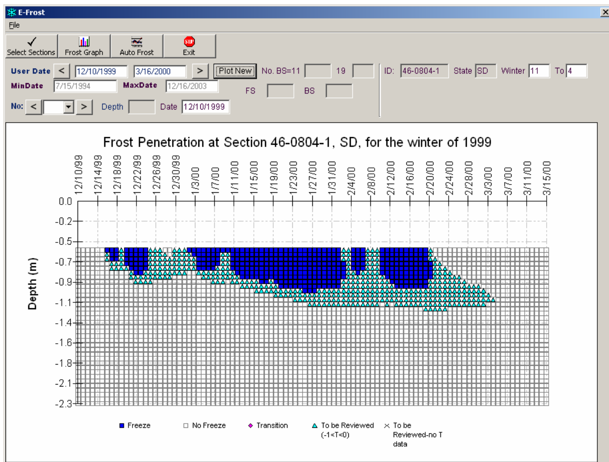
Figure 16. Chart. Example of temperature-based frost penetration profile for section 0804 in South Dakota.
