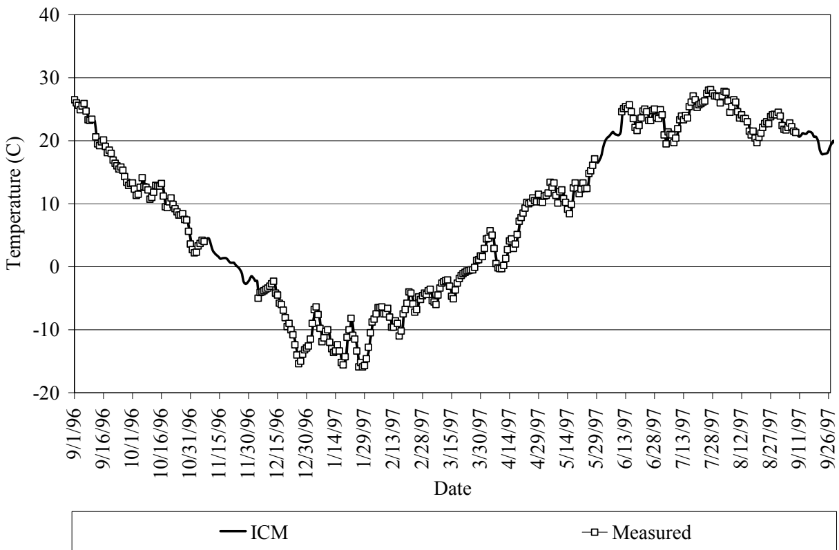
Figure 11. Chart. Measured and EICM predicted temperatures for section 6251 in Minnesota at 0.8 m (2.6 ft) depth after auto-correction.
