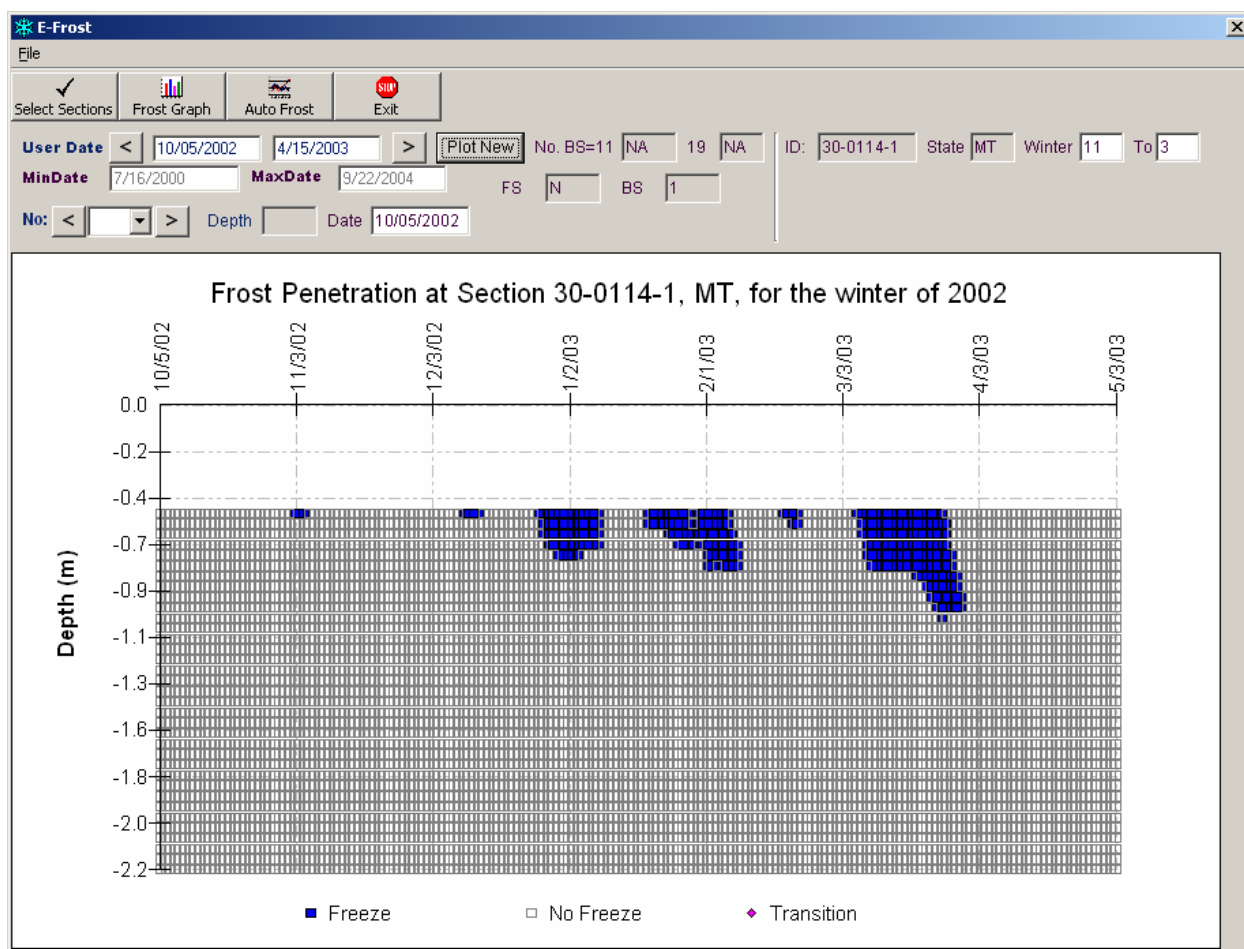
Figure 21. Chart. Frost penetration profile showing multiple freeze-thaw cycles.
