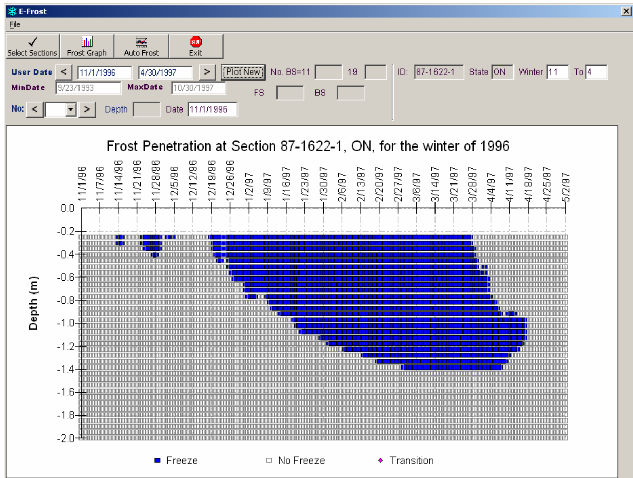
Figure 22. Chart. Frost penetration profile showing shallow freeze cycles in the fall followed by solid deep freeze with spring thaw.
