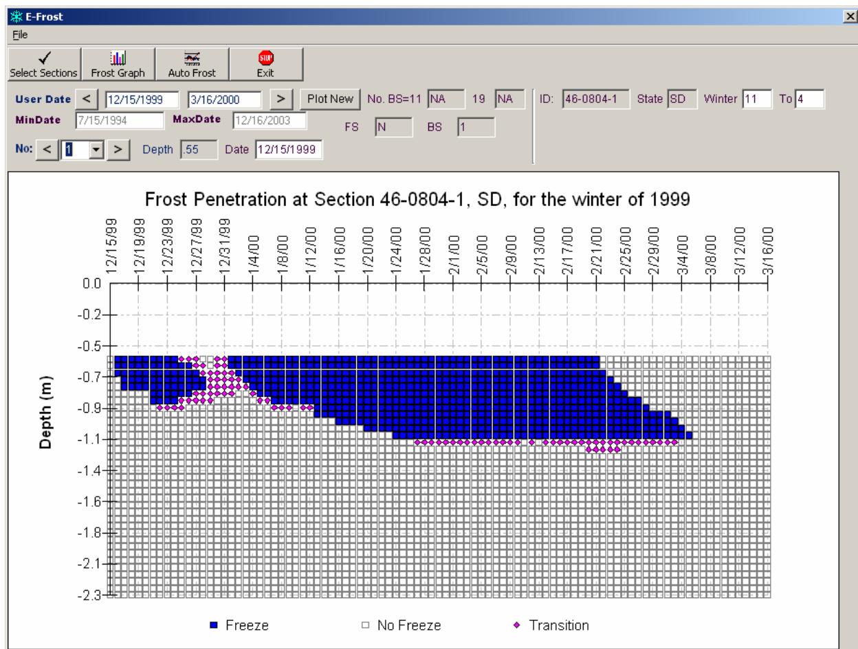
Figure 18. Chart. Example of final frost penetration profile for SMP site 46-0804 for the winter of 1999.
