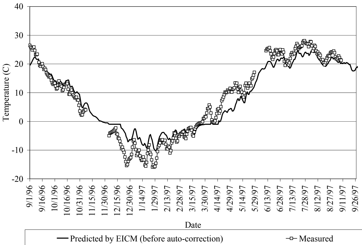
Figure 10. Chart. Measured and EICM predicted temperatures for section 6251 in Minnesota at 0.8 m (2.6 ft) depth before auto-correction.
