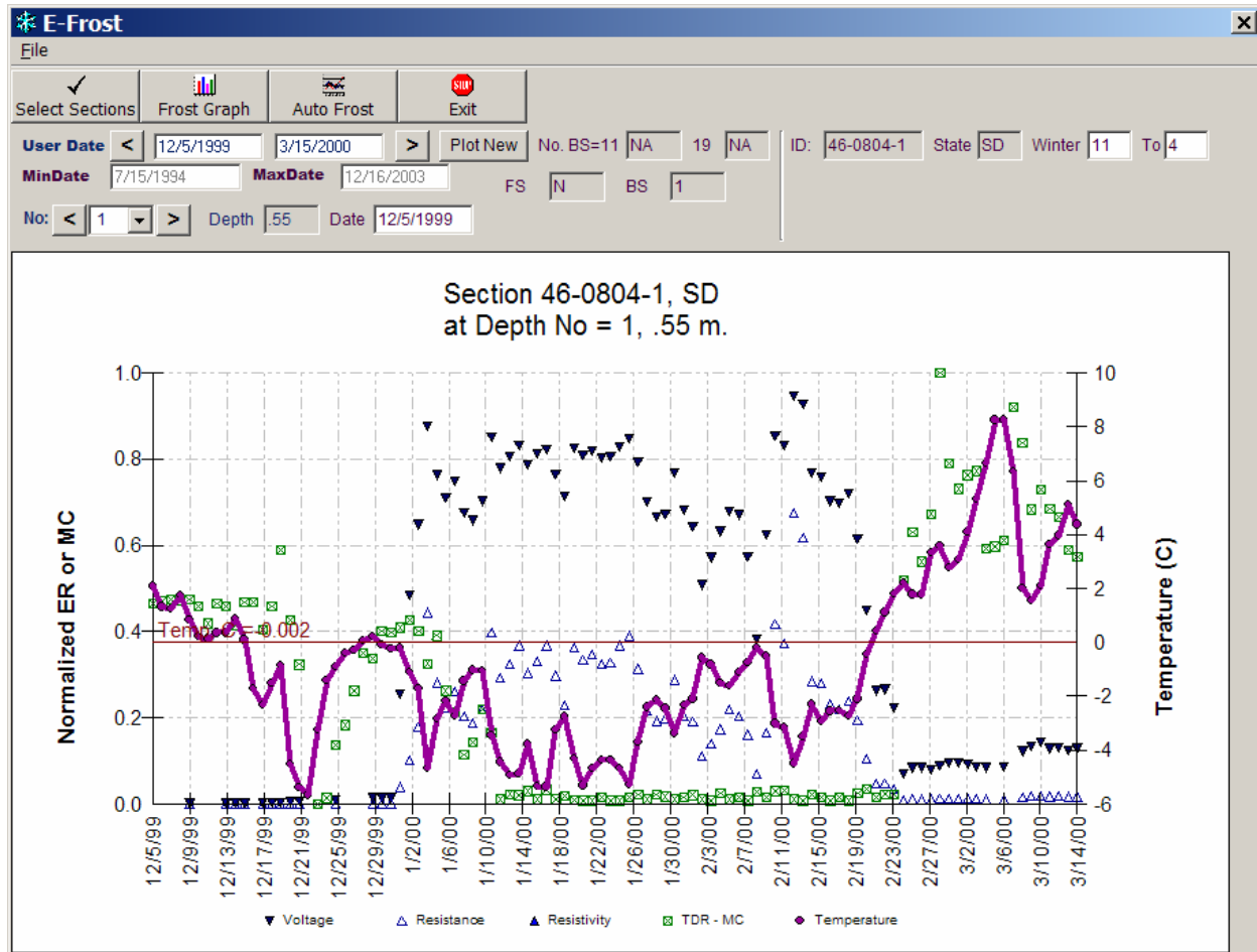
Figure 17. Chart. Example of ER, temperature, and moisture trends for section 0804 in South Dakota at 0.55 m (1.8 ft) depth.
