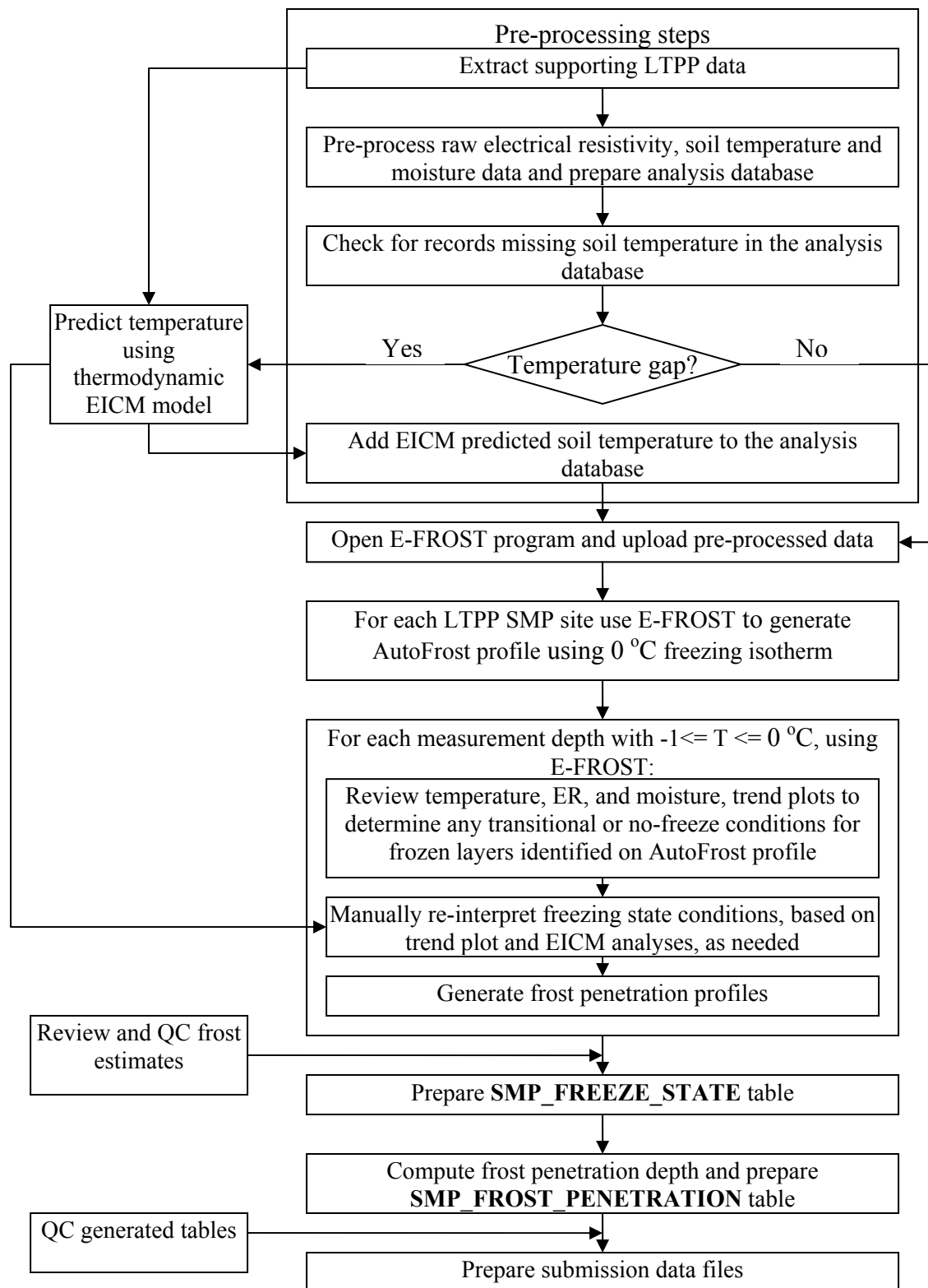
Figure 12. Chart. Frost depth and layers interpretation using E-FROST.
