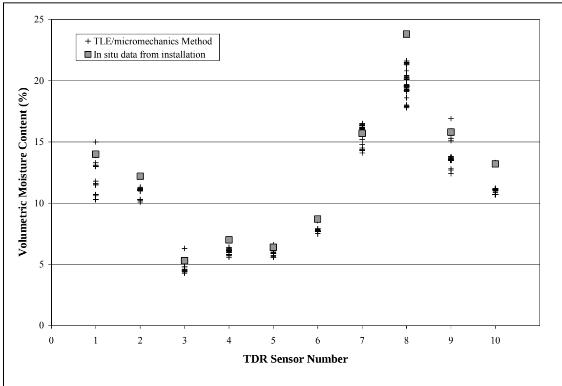
Figure 32. Graph. Results from the TLE micromechanics method for LTPP section 313018.
