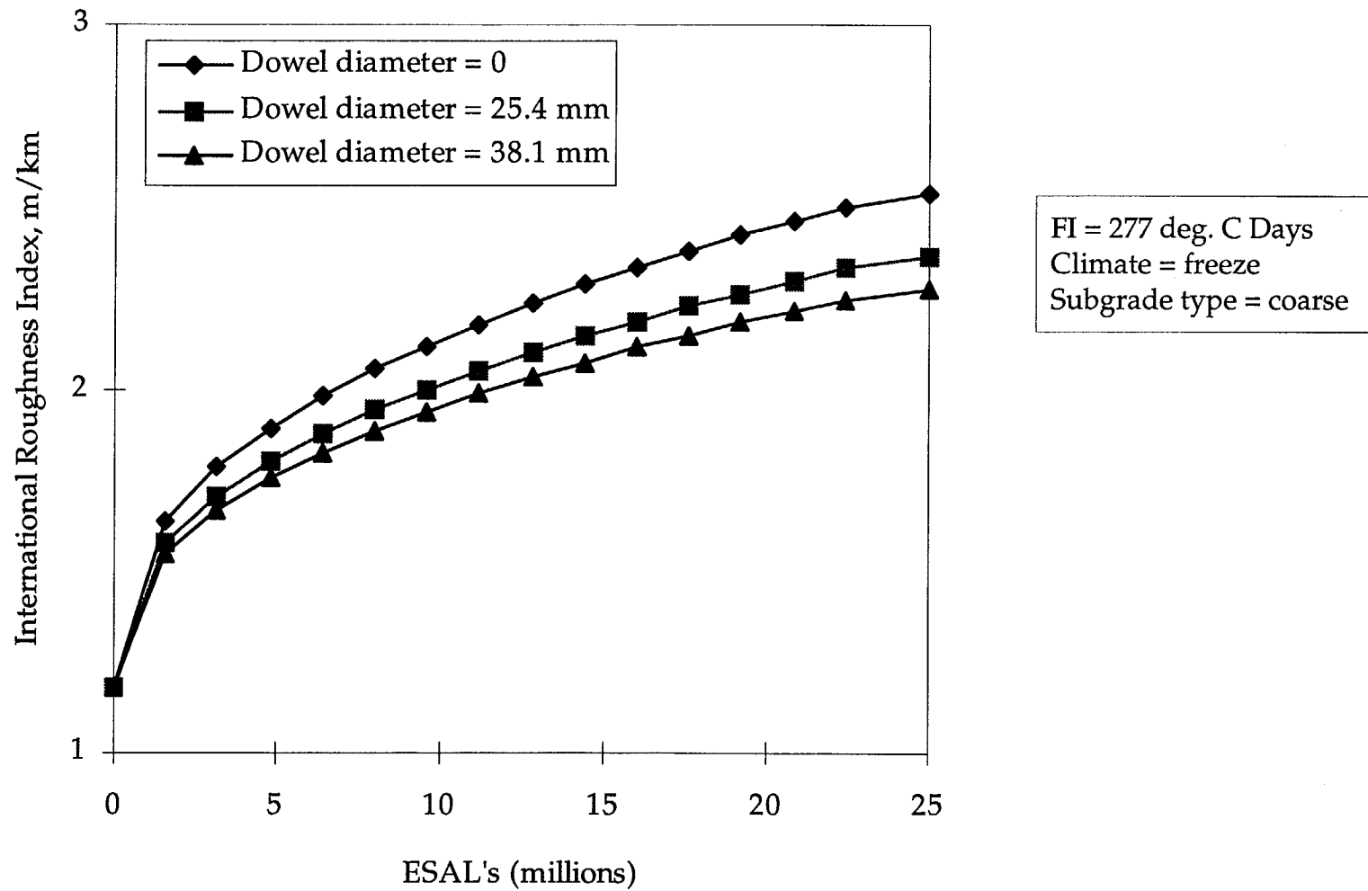
Figure 24. Influence of dowel diameter on JPCP roughness.
