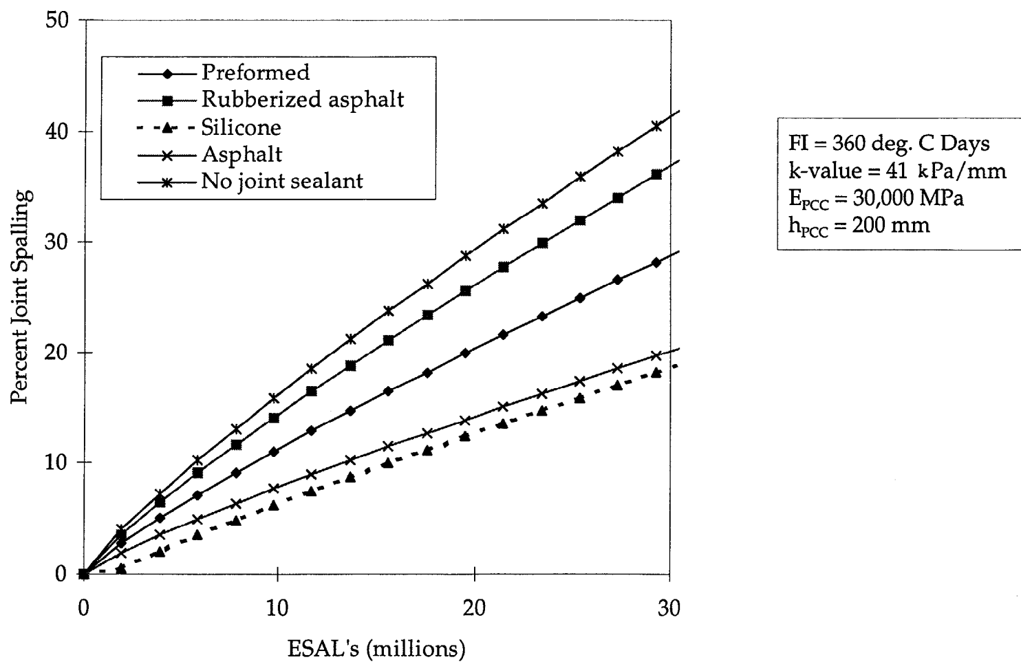
Figure 25. Influence of joint sealant type on JRCP transverse joint spalling.
