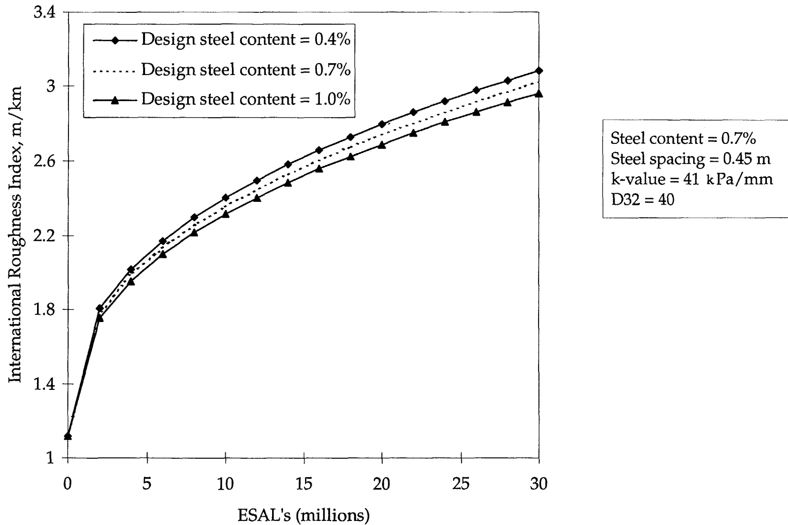
Figure 26. Influence of design longitudinal steel content on CRCP roughness.
