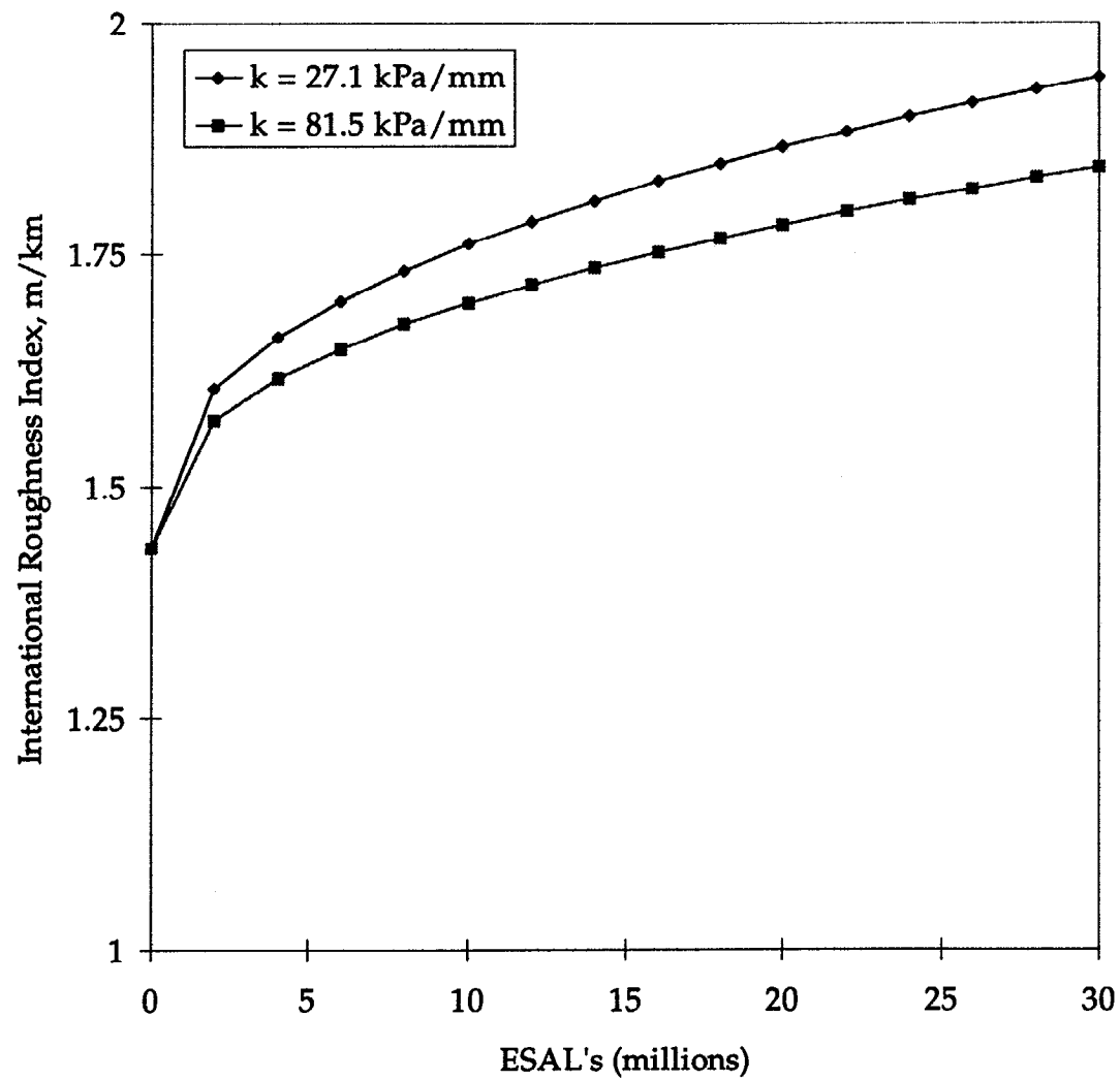
Figure 16. Effect of modulus of subgrade reaction on IRI for CRCP.
