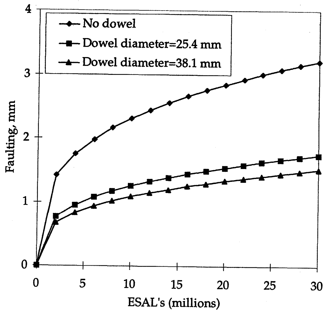
Figure 17. Influence of dowels on JPCP faulting.
