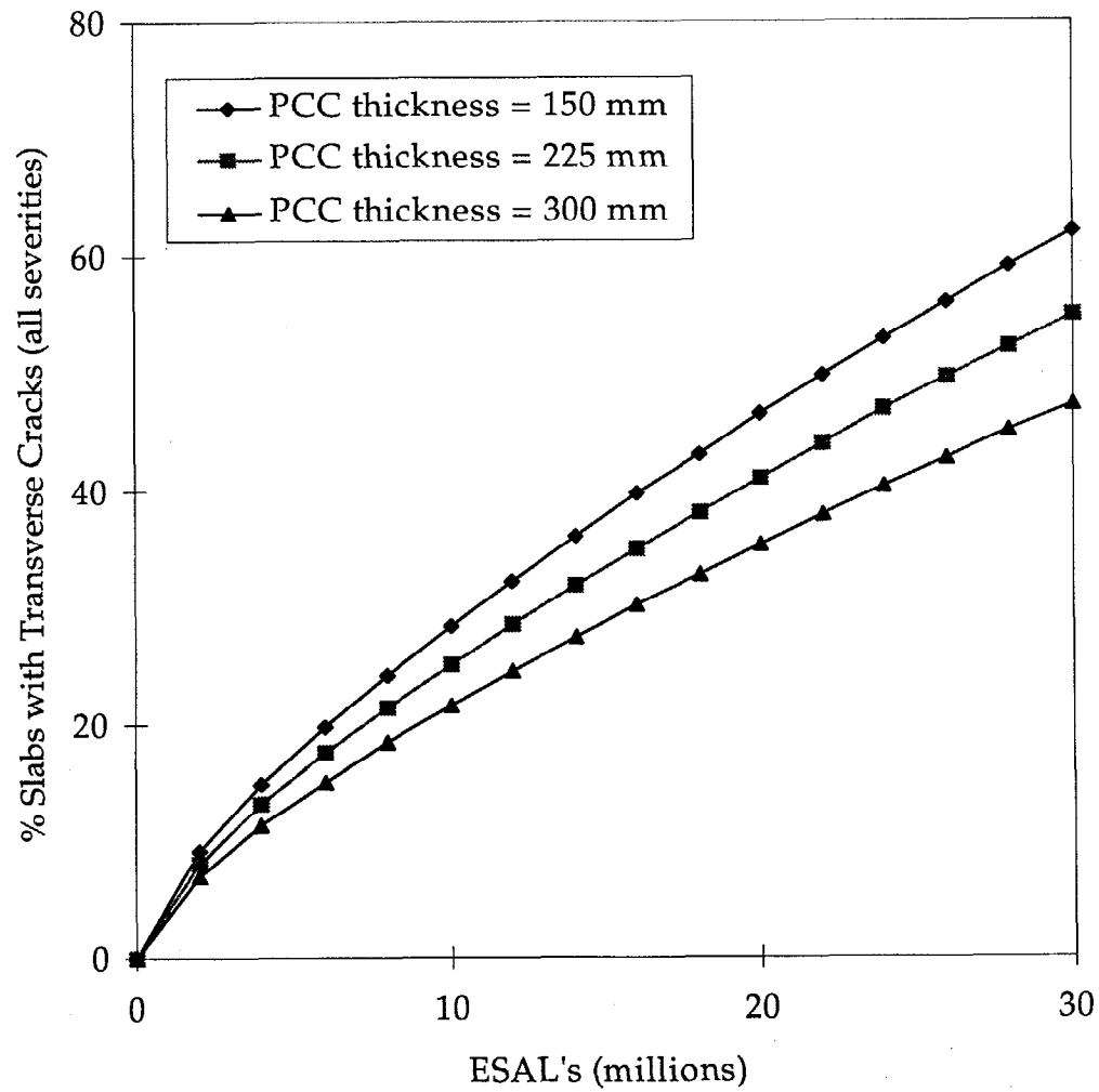
Figure 2. Percent slabs with transverse cracking versus traffic loadings, showing the effect of different PCC slab thickness.
