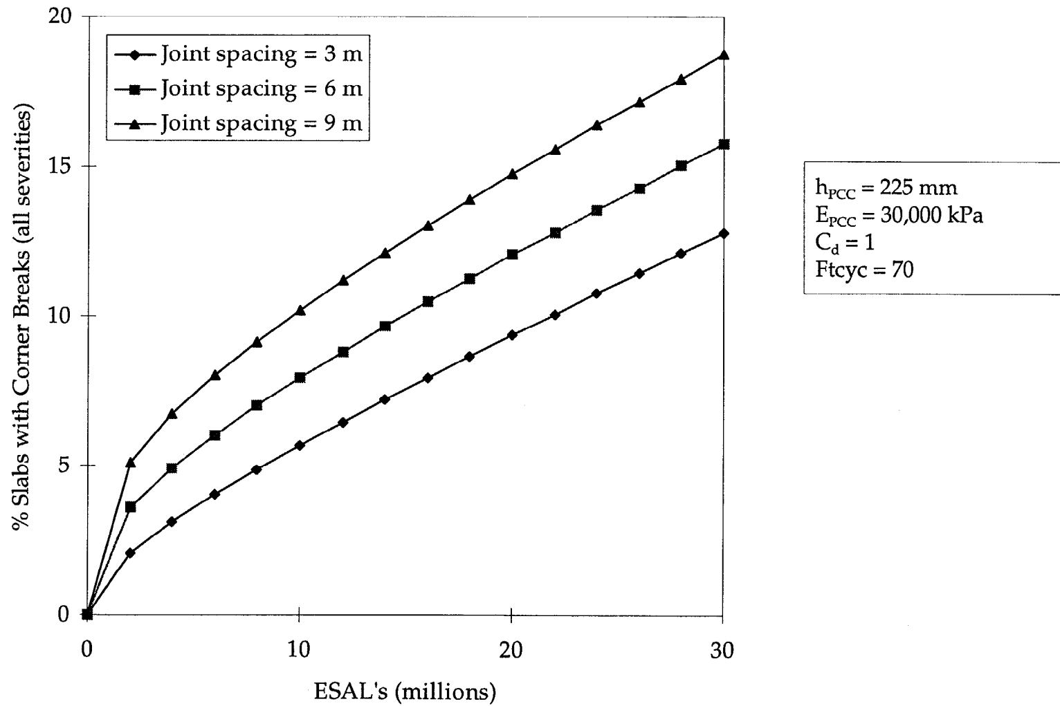
Figure 23. Plot of percent slabs with corner breaks versus cumulative ESAL's for different PCC slab joint spacing.
