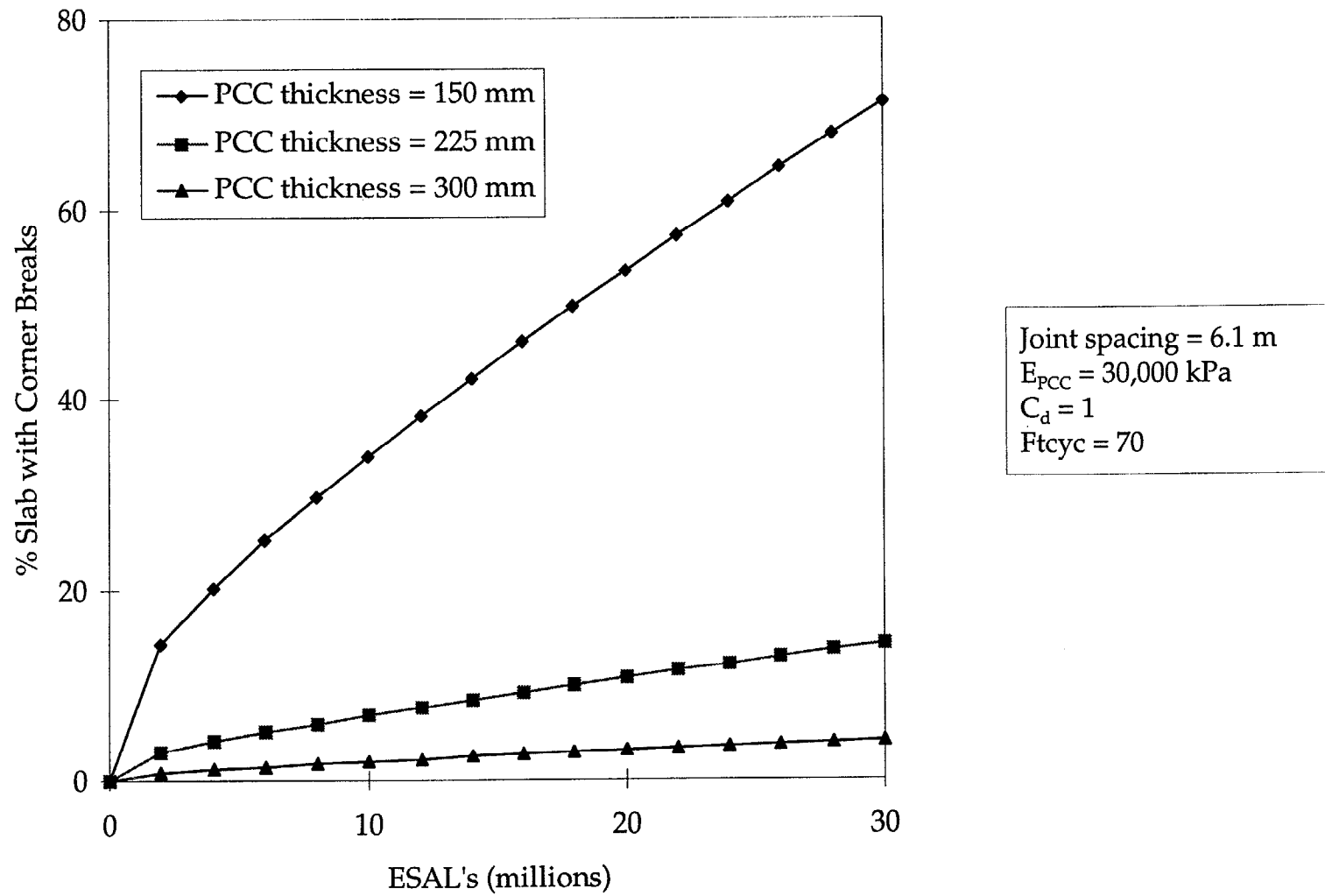
Figure 22. Percent slabs with corner breaks versus cumulative ESAL's for different slab thicknesses.
