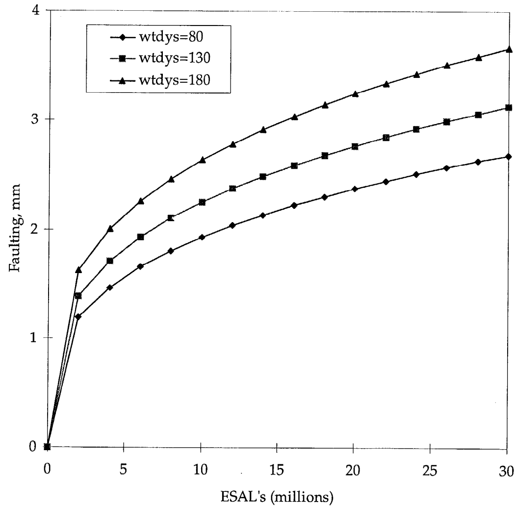
Figure 7. Effect of annual number of wet days on JPCP faulting.
