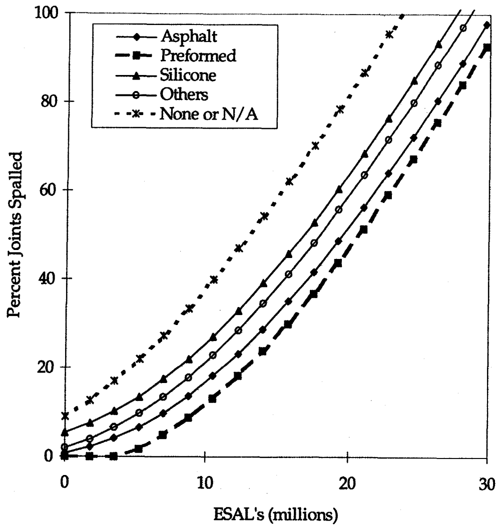
Figure 20. Plot of percent JPCP spalling versus traffic for the different joint sealant materials evaluated.
