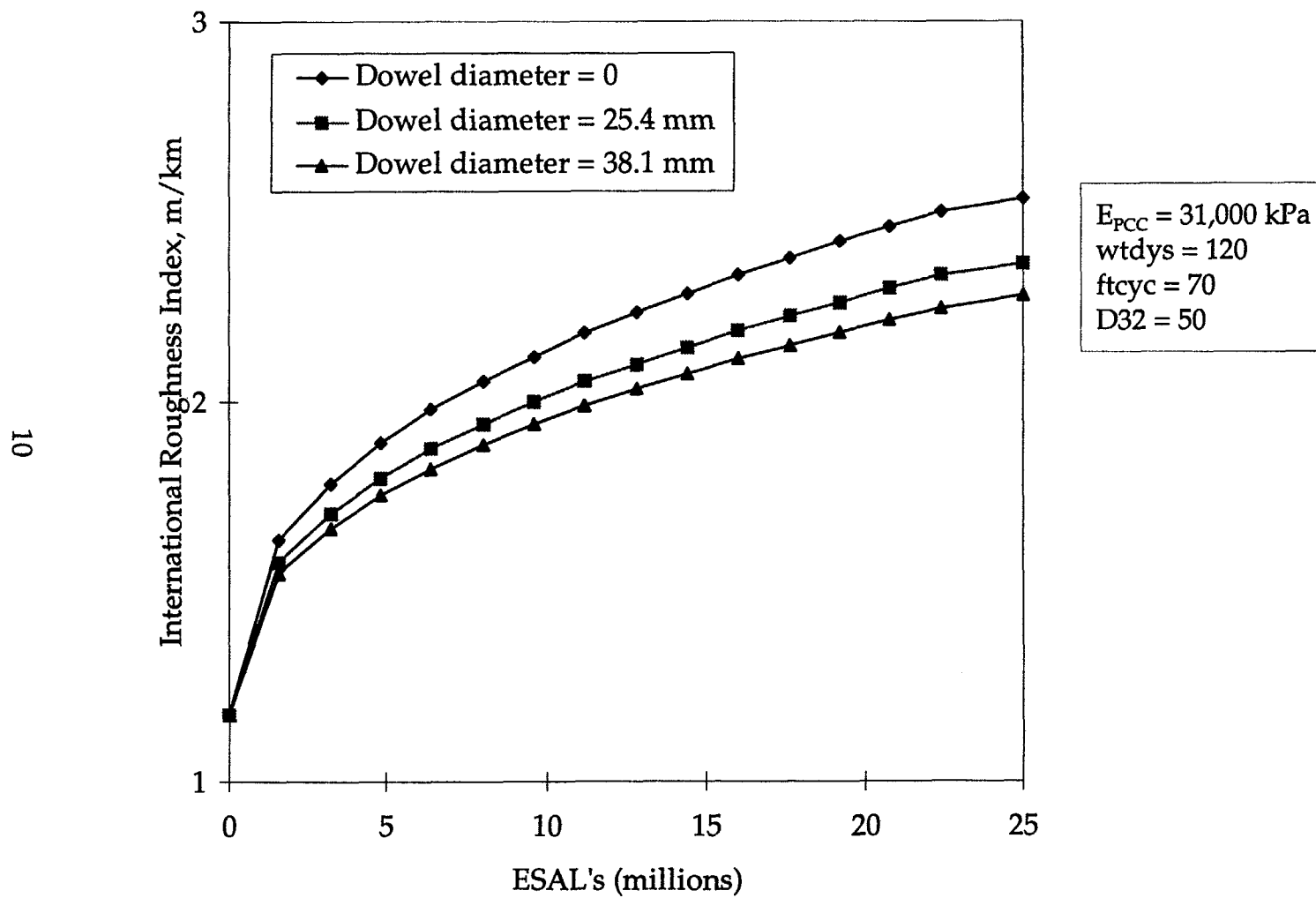
Figure 4. Plot of roughness versus traffic loadings, showing the effect of different dowel diameters.
