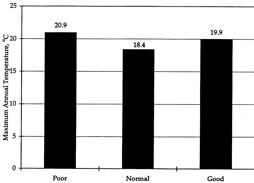
Figure 102. Effect of maximum annual temperature for CRCP localized failures.
