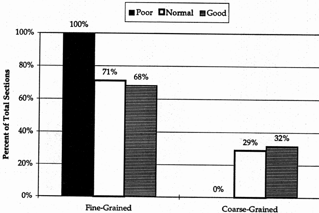
Figure 43. Effect of subgrade soil on JRCP performance.
