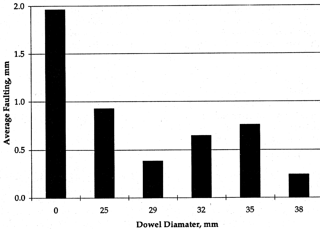
Figure 69. Effect of dowel bar diameter on JPCP/JRCP performance.
