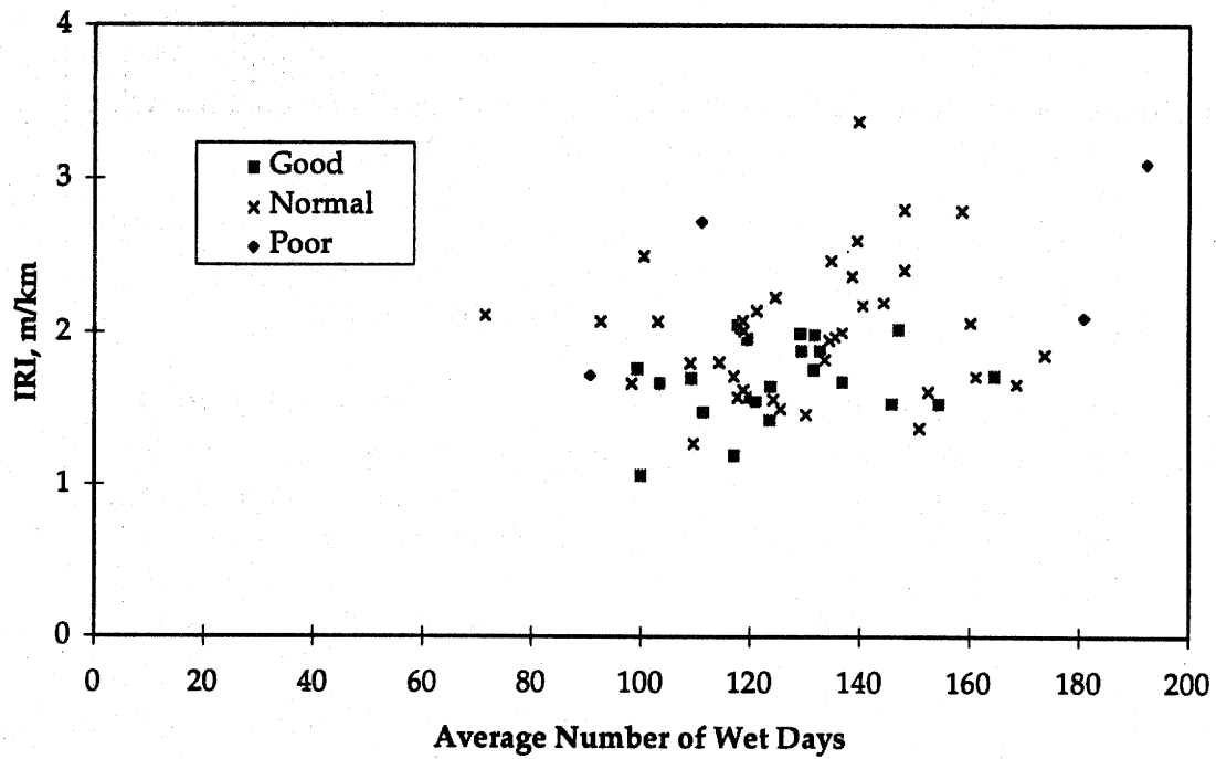
Figure 41. Average number of wet days versus IRI for JRCP.
