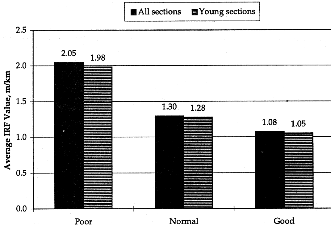
Figure 37. Comparison of average IRF values for JPCP.
