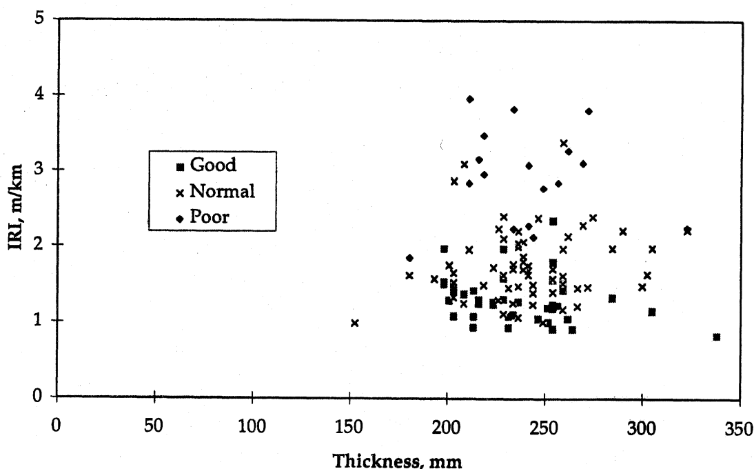
Figure 27. PCC slab thickness versus IRI for JPCP.
