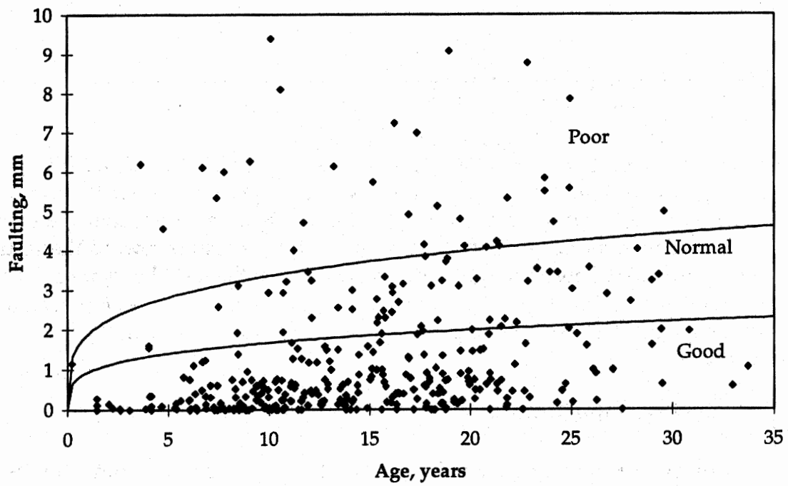
Figure 65. Faulting versus pavement age (all observations).
