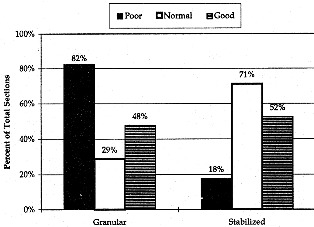
Figure 28. Effect of base-layer type on JPCP IRI performance.
