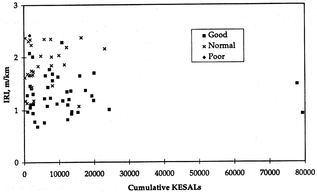
Figure 56. Cumulative KESALs versus IRI for CRCP.
