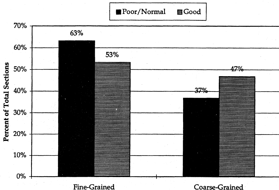
Figure 55. Effect of subgrade soil on CRCP performance.
