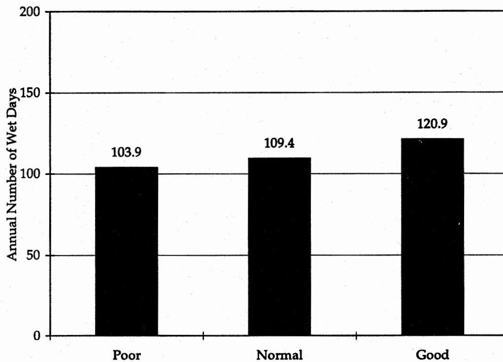
Figure 106. Effect of annual wet days on CRCP localized failures.
