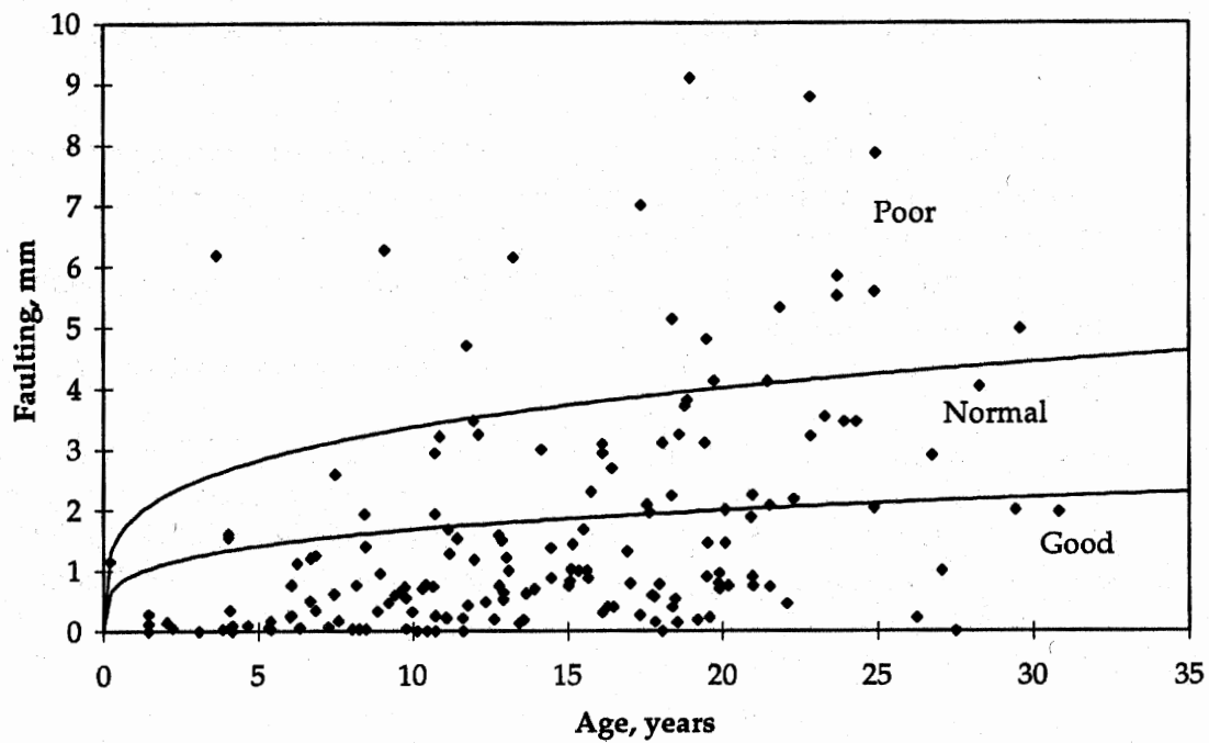
Figure 66. Faulting versus pavement age (last observation only).
