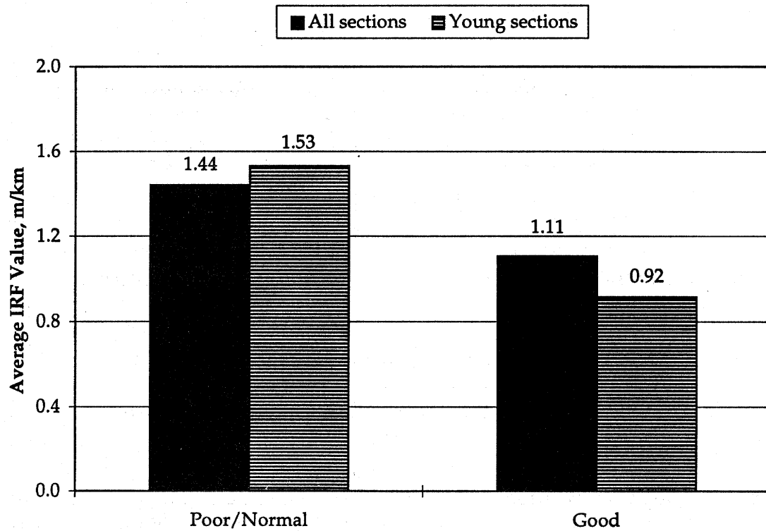
Figure 63. Comparison of average IRF values for CRCP.
