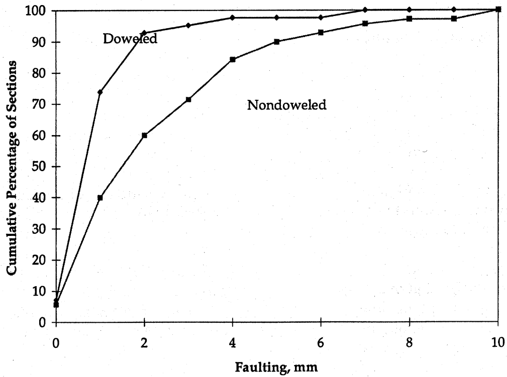
Figure 68. Cumulative frequency curves for doweled and non-doweled JPCP.
