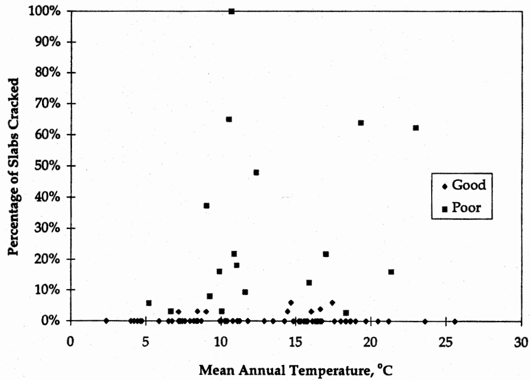
Figure 89. Average annual mean temperature versus JPCP transverse cracking.
