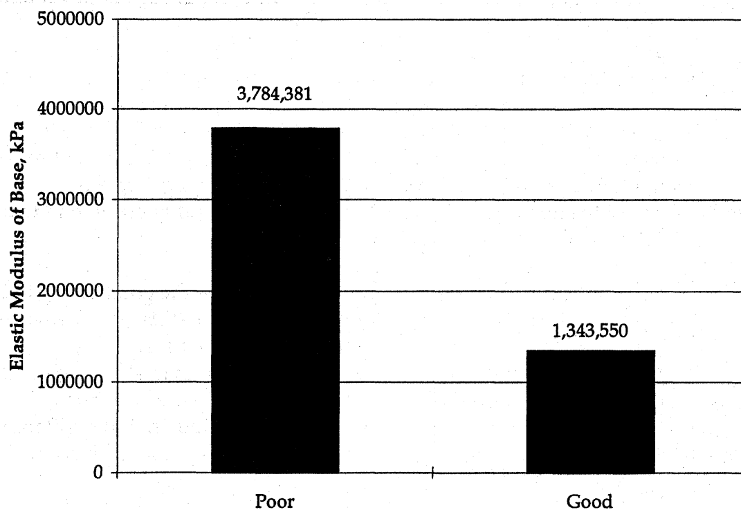
Figure 8. Effect of average elastic modulus of base on JPCP IRI performance
