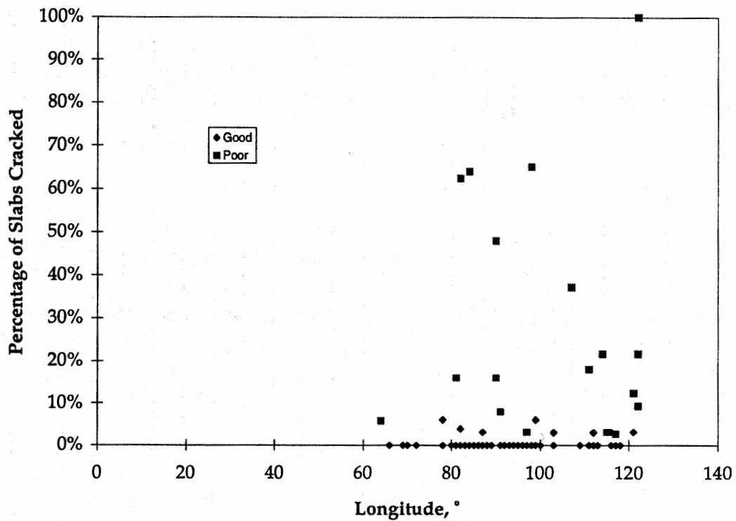
Figure 88. Longitude versus percentage of cracked slabs.
