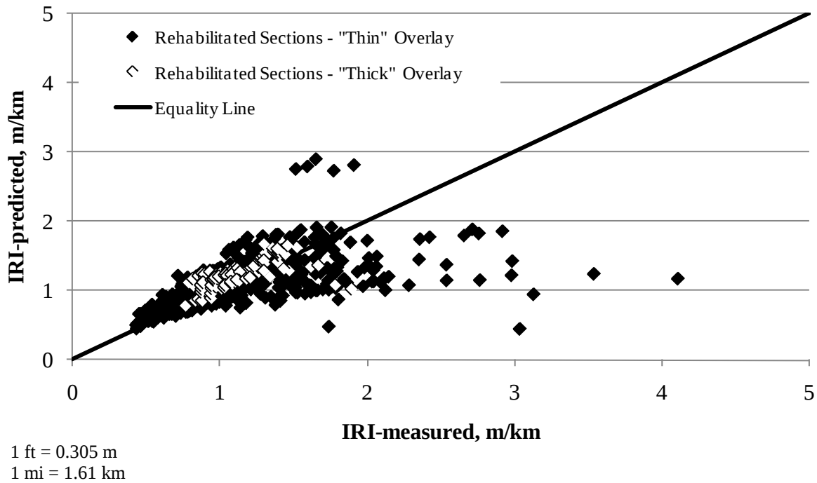
Figure 72. Graph. LTPP-measured versus MEPDG-predicted IRI for SPS-5 rehabilitated sections grouped by thickness.
