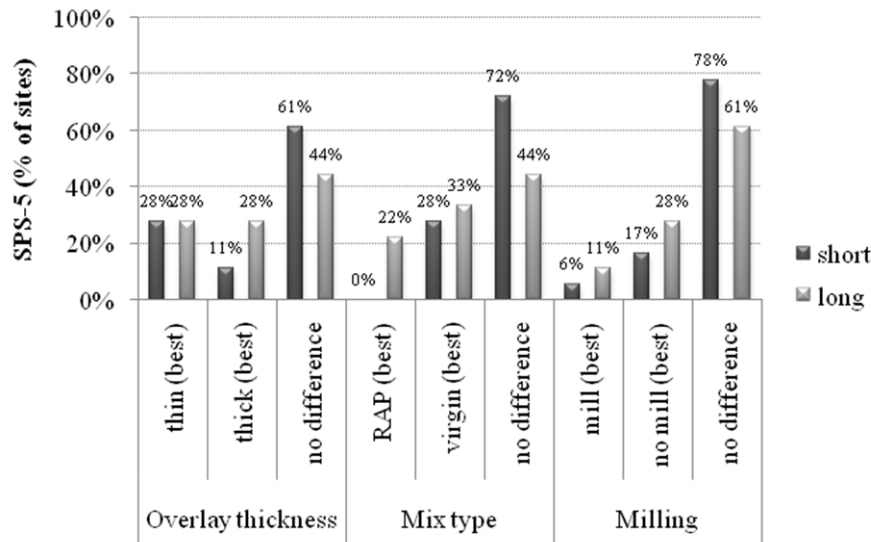
Figure 20. Graph. Summary of SPS-5 sites by best-performing design feature for rutting according to repeated measures ANOVA results.
