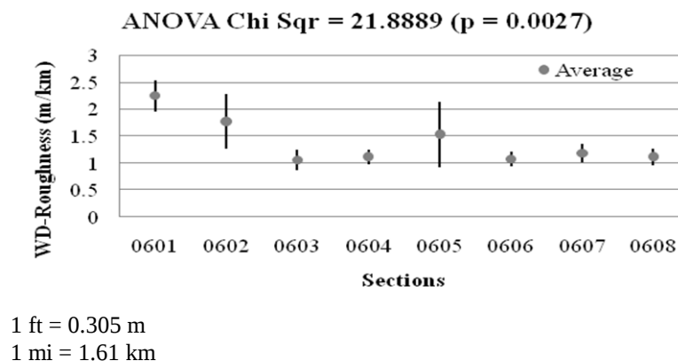
Figure 48. Graph. Short-term WD-roughness values for JRCP at SPS-6 sites.
