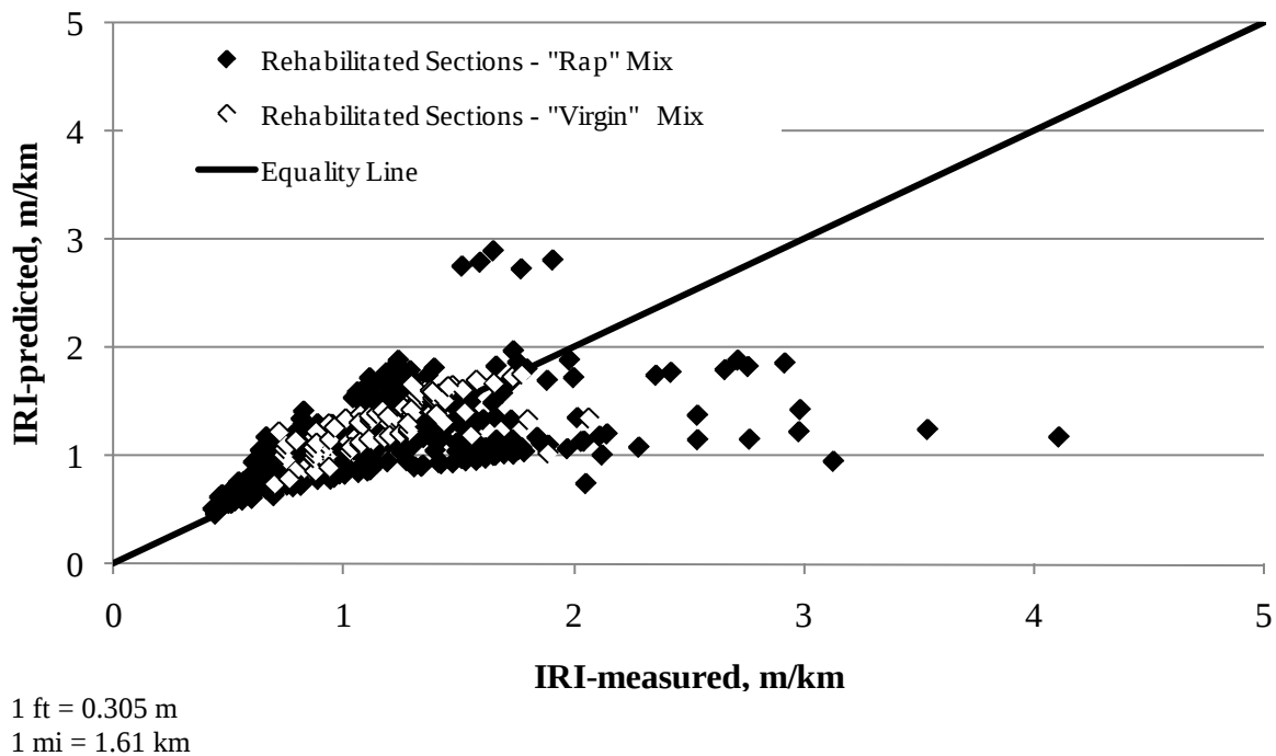
Figure 73. Graph. LTPP-measured versus MEPDG-predicted IRI for SPS-5 rehabilitated sections grouped by mix type.
