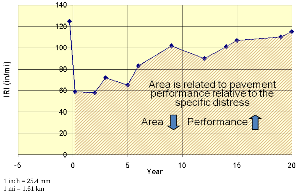
Figure 24. Graph. Example of WD-distress values in comparative performance analysis for IRI trend after rehab.
