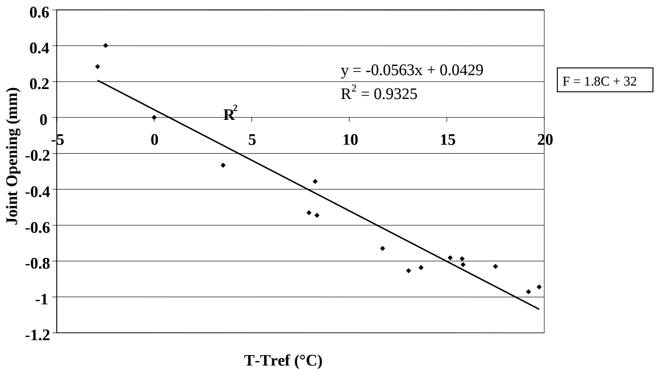
Figure 87. Change in joint opening versus change in PCC temperature, section 484143.
