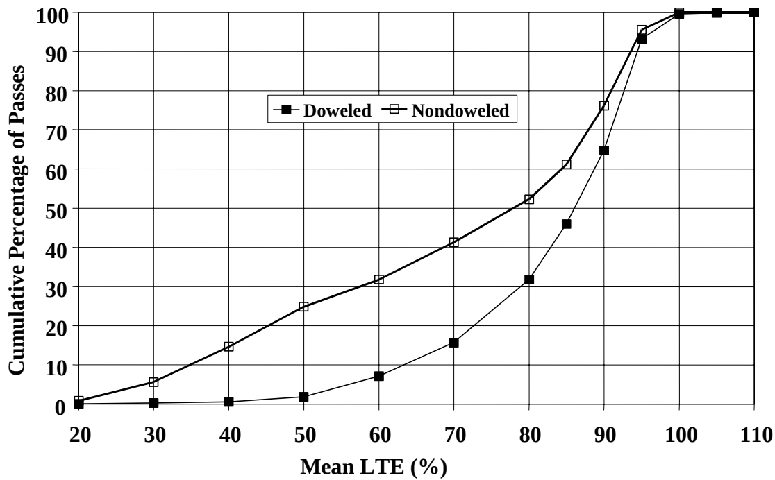
Figure 22. Distribution of section LTE mean value, nondoweled versus doveled, leave test (J5).
