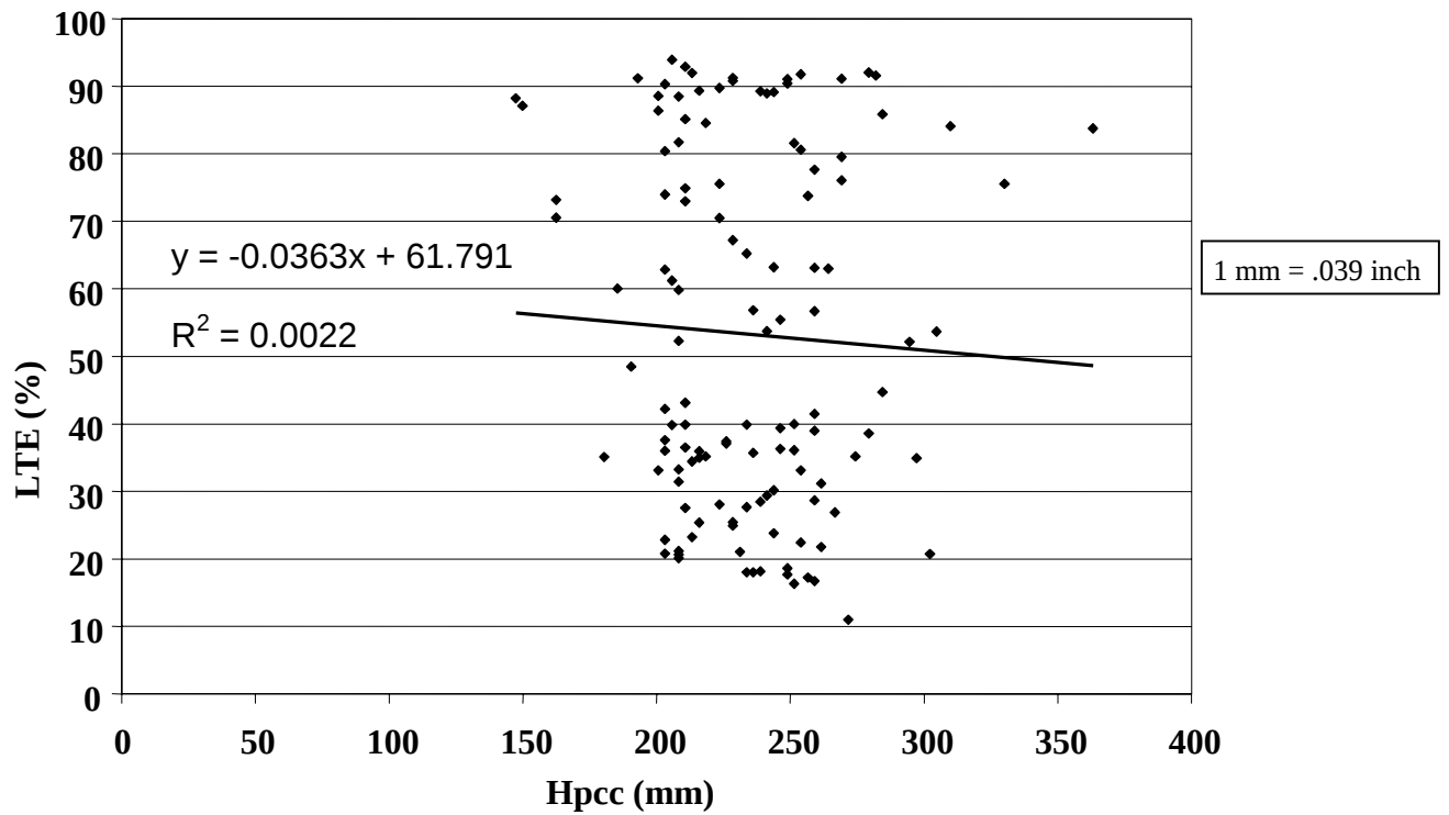
Figure 37. PCC thickness versus LTE in JCP nondoweled sections.
