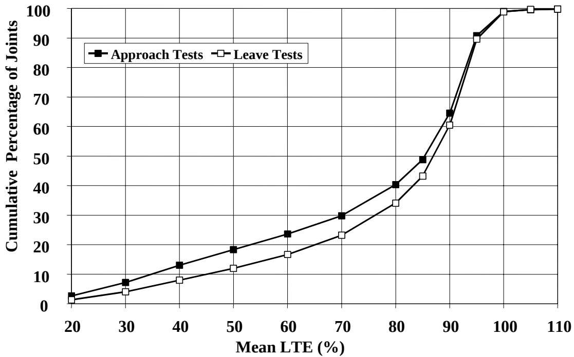
Figure 9. Distribution of joint LTE mean values, JCP sections.
