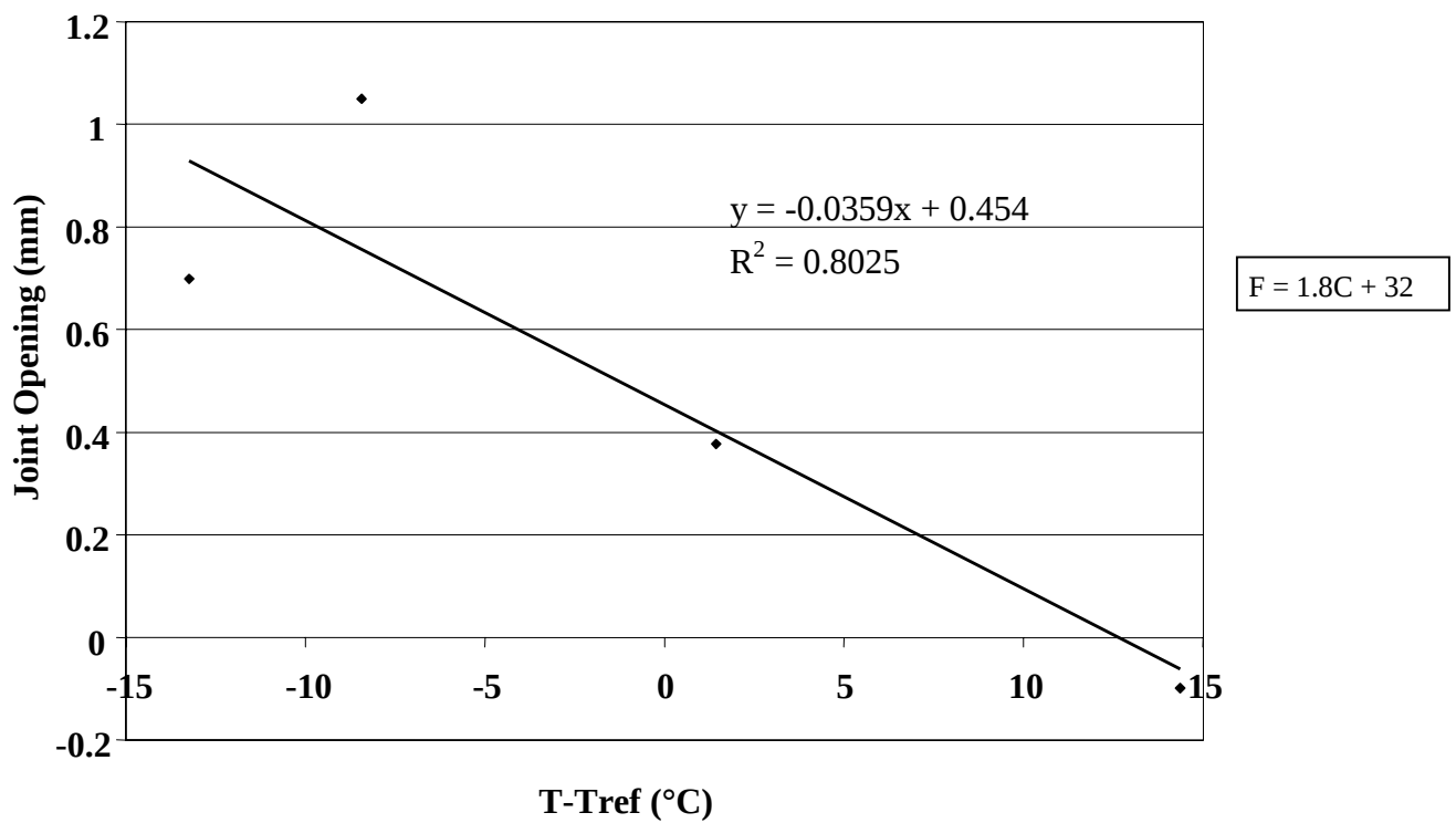
Figure 79. Change in joint opening versus change in PCC temperature, section 204054.
