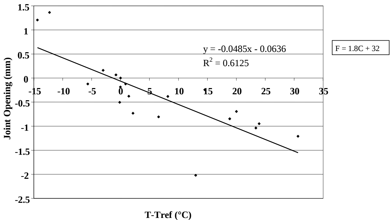
Figure 89. Change in joint opening versus change in PCC temperature, section 833802.
