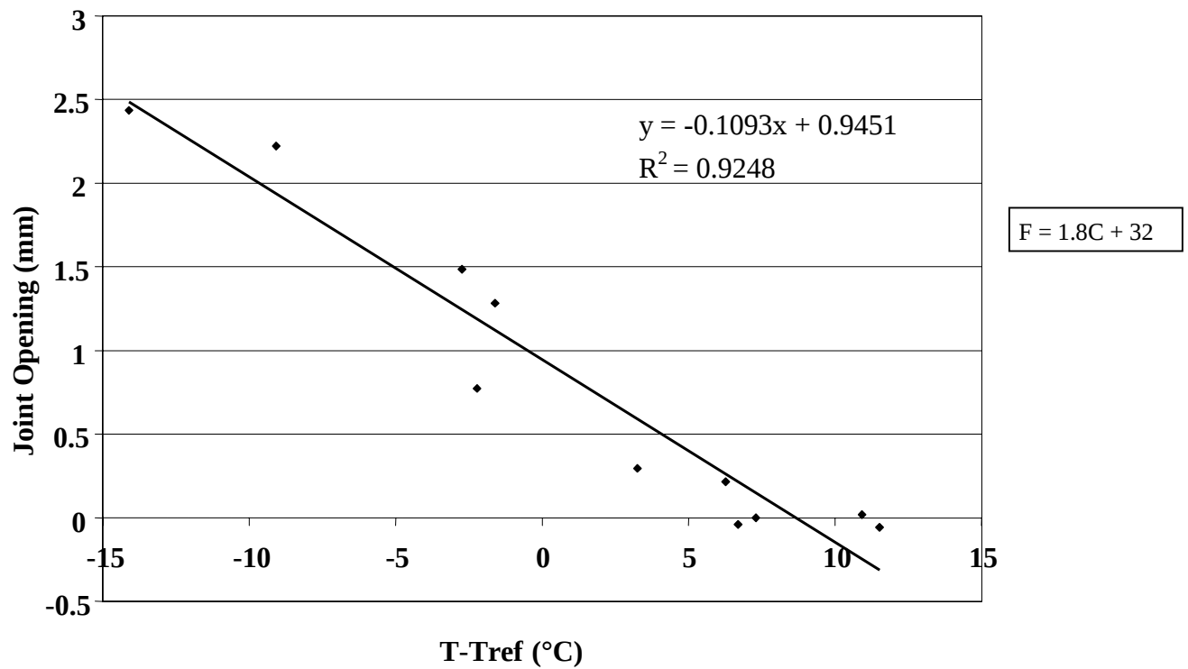
Figure 85. Change in joint opening versus change in PCC temperature, section 421606.
