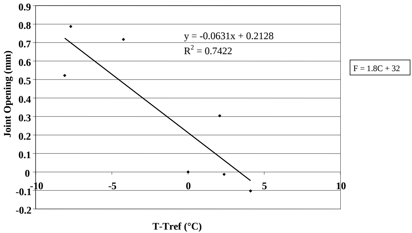
Figure 84. Change in joint opening versus change in PCC temperature, section 390204.
