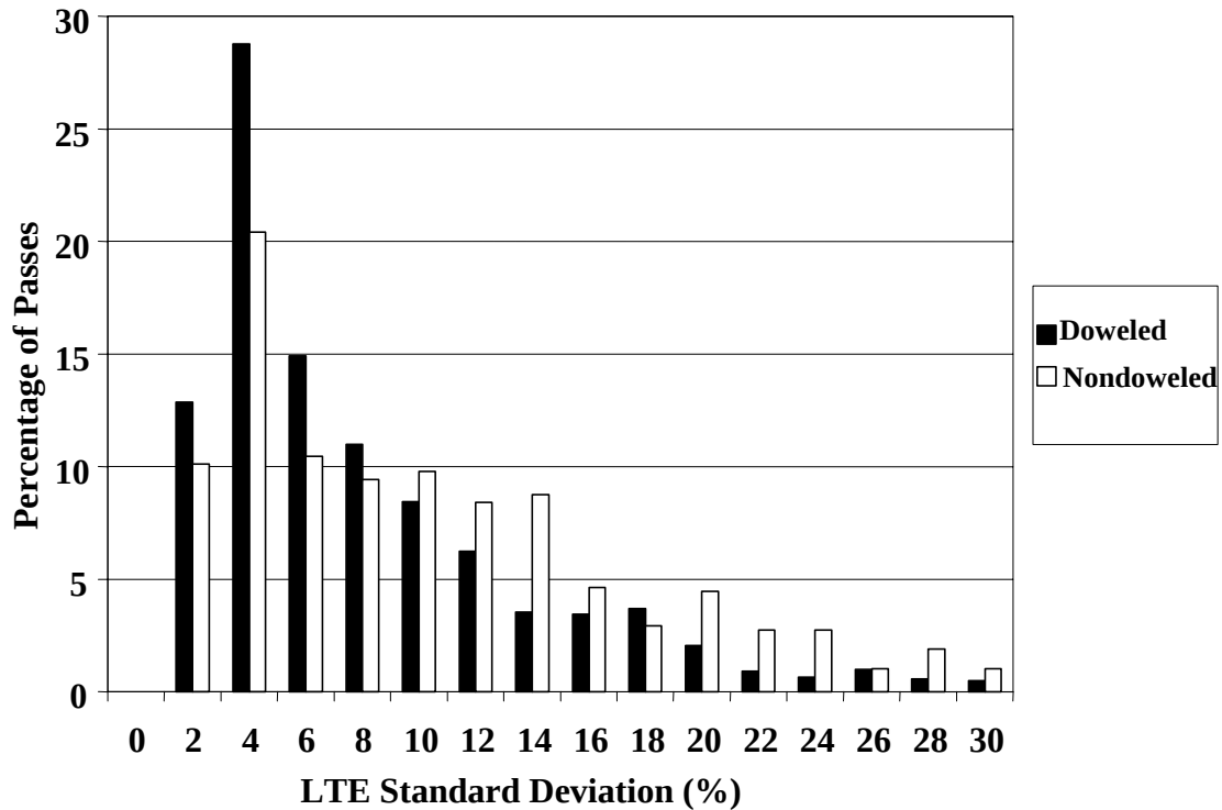
Figure 19. Comparison of standard deviations of section LTE for doweled and nondoweled JCP sections (approach tests).
