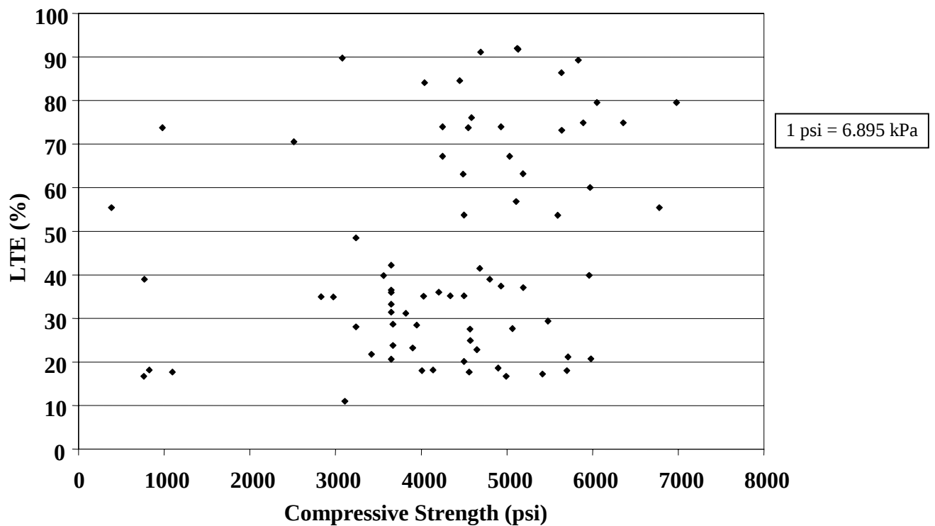
Figure 40. PCC compressive strength versus LTE in nondoweled sections.
