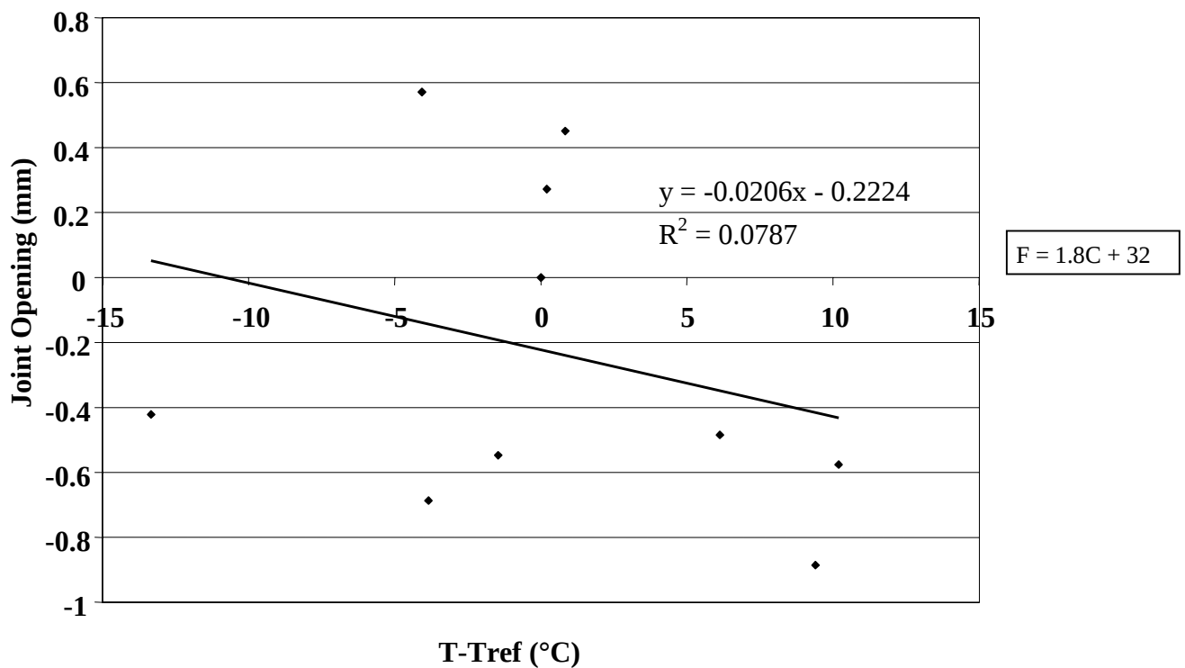
Figure 83. Change in joint opening versus change in PCC temperature, section 370201.
