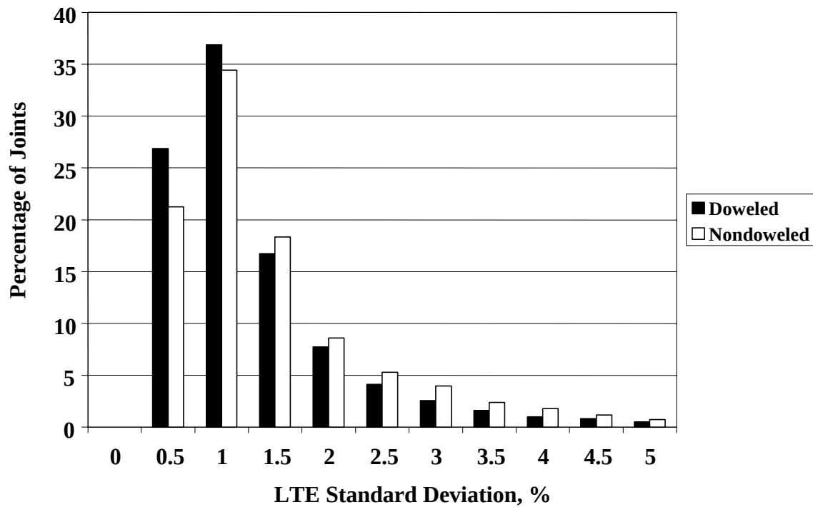
Figure 13. Frequency distributions of standard deviations of LTEs for nondoweled and doweled joints, approach test.
