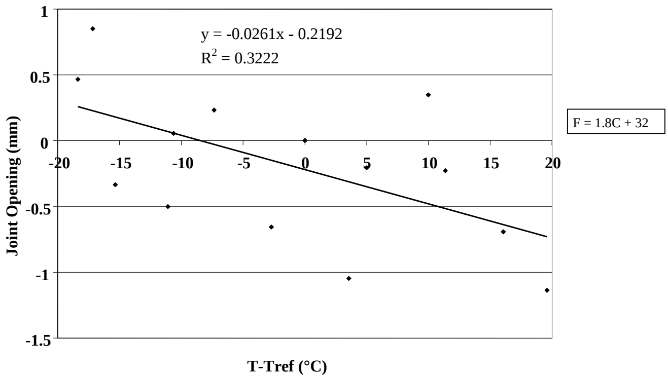
Figure 76. Change in joint opening versus change in PCC temperature, section 040215.
