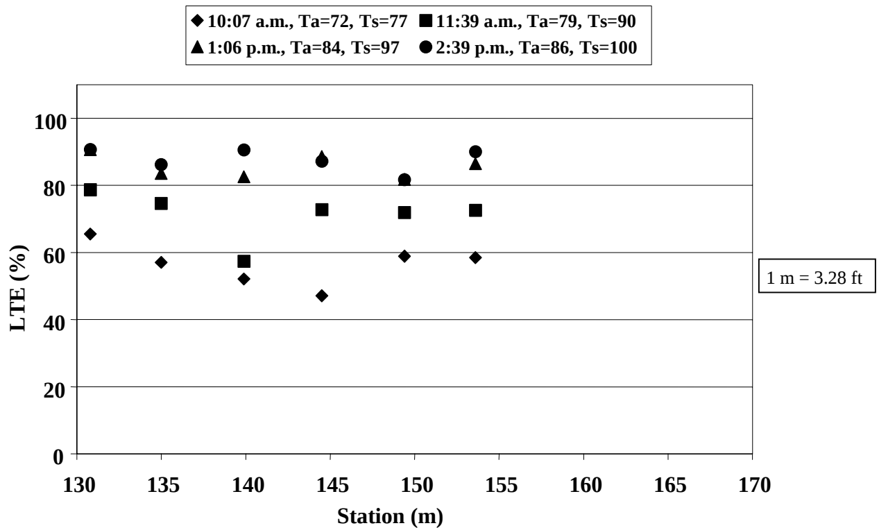
Figure 59. Daily variation in calculated leave LTE, section 4_0215 (March 1996).
