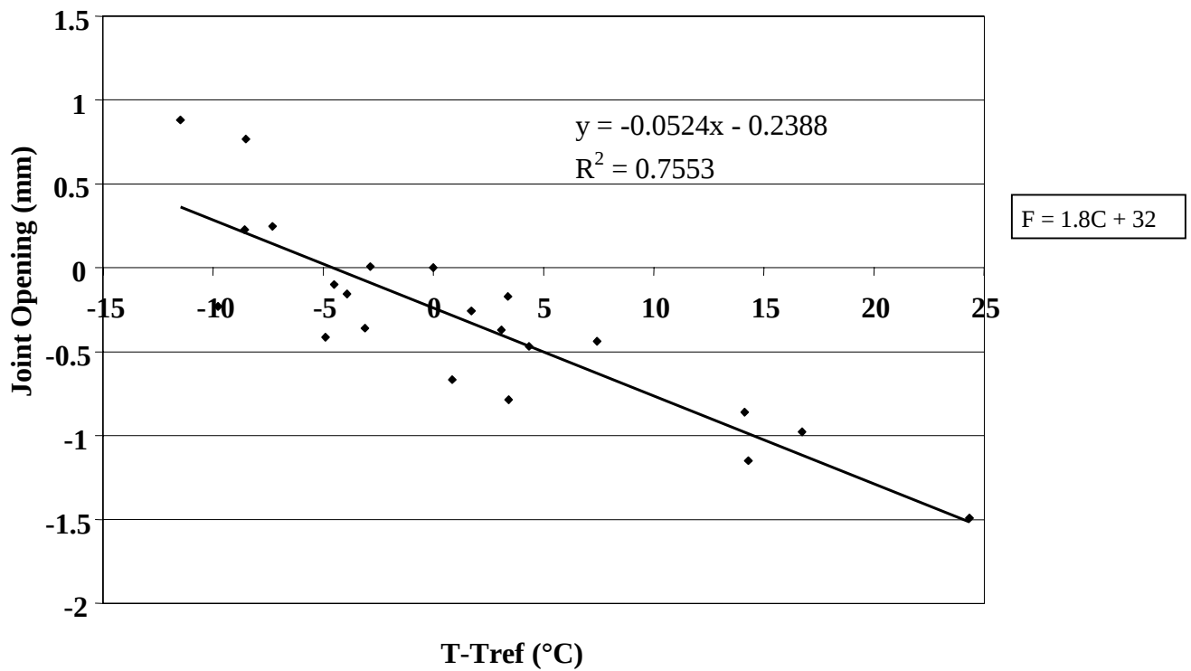
Figure 80. Change in joint opening versus change in PCC temperature, section 274040.
