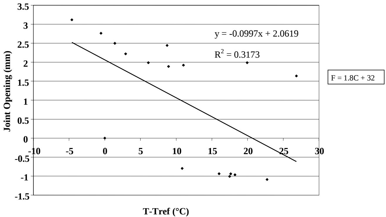
Figure 82. Change in joint opening versus change in PCC temperature, section 364018.
