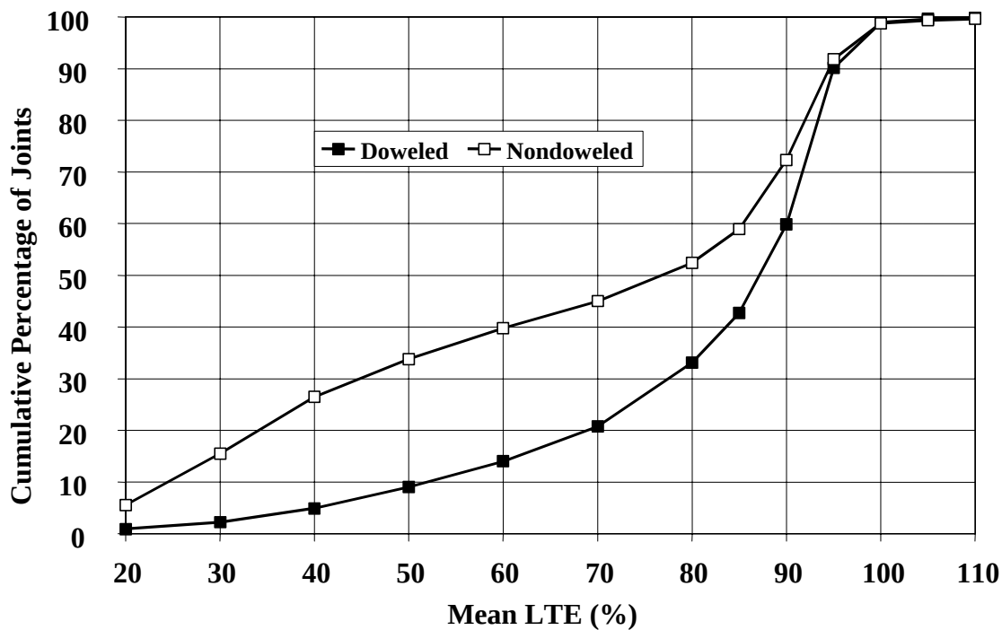
Figure 23. Distribution of joint LTE mean value, nondoweled versus doveled, approach test (J4).
