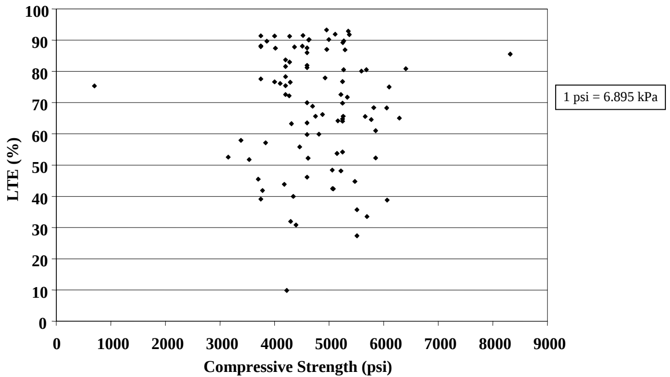
Figure 39. PCC compressive strength versus LTE in JCP doweled sections.
