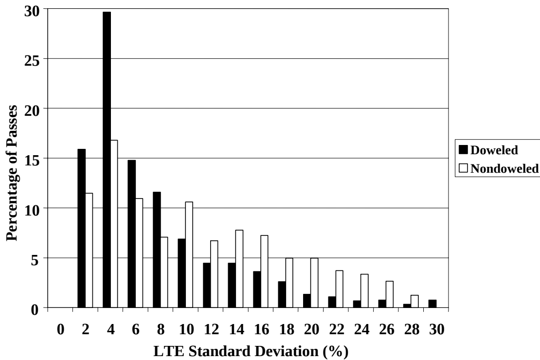
Figure 20. Comparison of standard deviations of section LTE for doveled and nondoweled JCP sections (leave tests).
