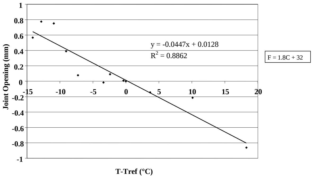
Figure 88. Change in joint opening versus change in PCC temperature, section 493011.
