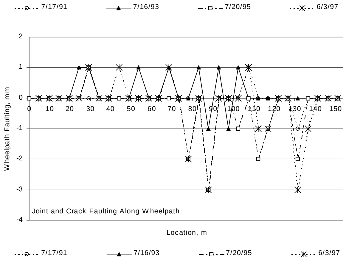
Figure 5. Example of consistent negative faulting (GPS-3 section 893016).
