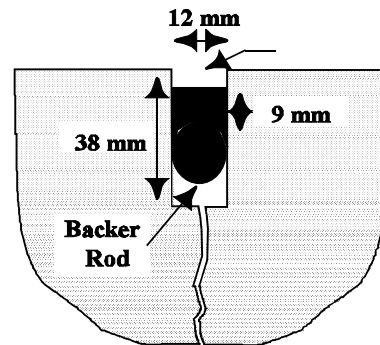
J. Deep Reservoir-and-Recess (backer rod)
