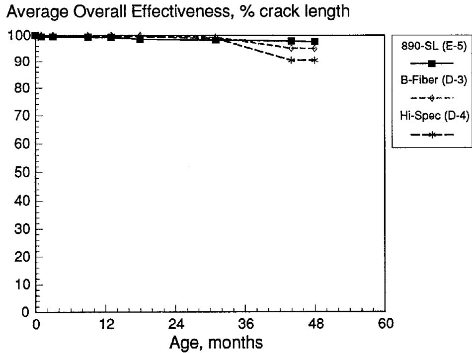
Figure 29. Time-series effectiveness trends of Elma, WA crack-seal treatments (continued).
