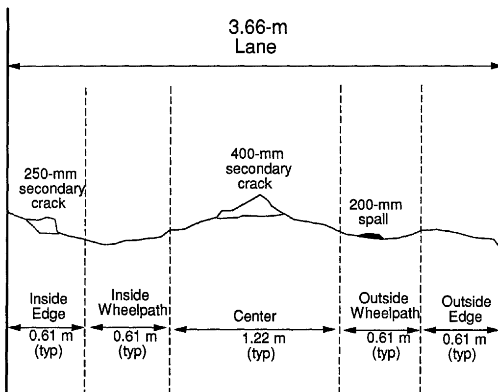
Figure 9. Initial inspection sketch of transverse crack.
