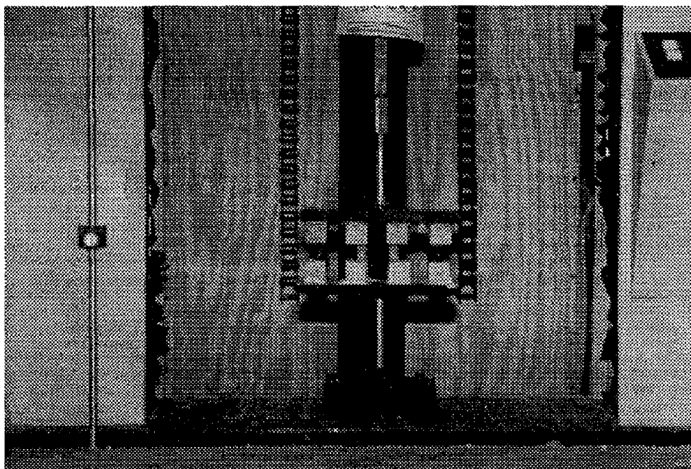
Figure 25. ASTM D 3583 tensile adhesion testing.
