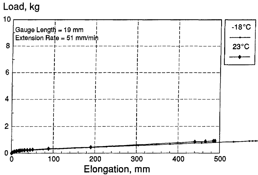
Figure C-5. ASTM D 412 load-deformation curves for 890-SL
