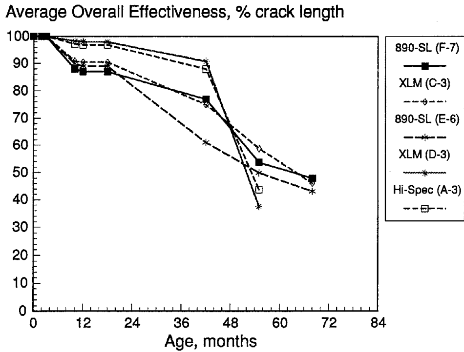
Figure 30. Time-series effectiveness trends of Wichita, KS adverse-conditions crack-seal treatments (continued).
