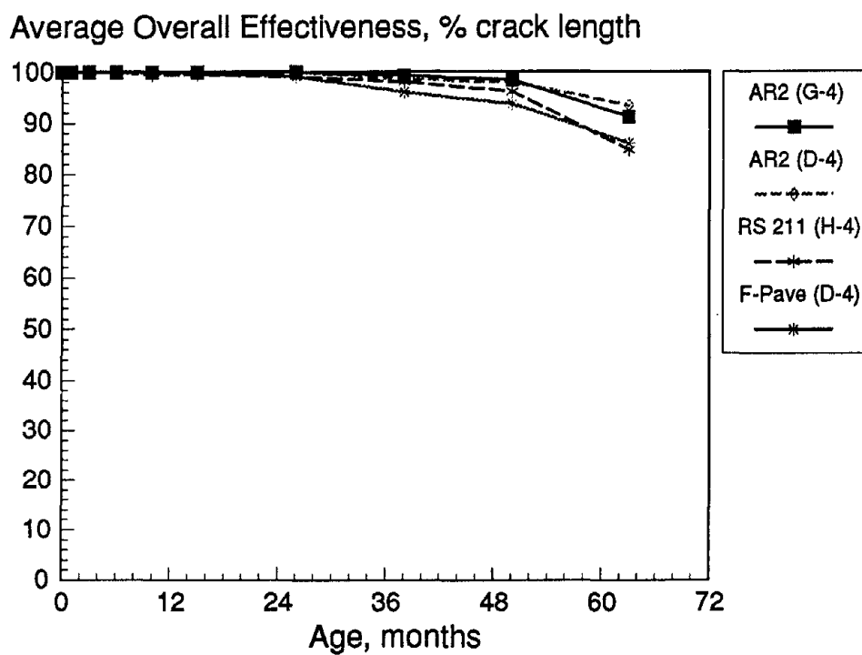
Figure 36. Time-series effectiveness trends of Prescott, ON crack-fill treatments.
