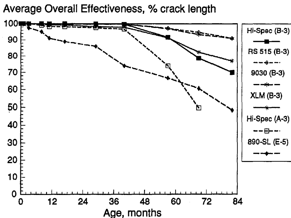
Figure 28. Time-series effectiveness trends of Abilene, TX crack-seal treatments.
