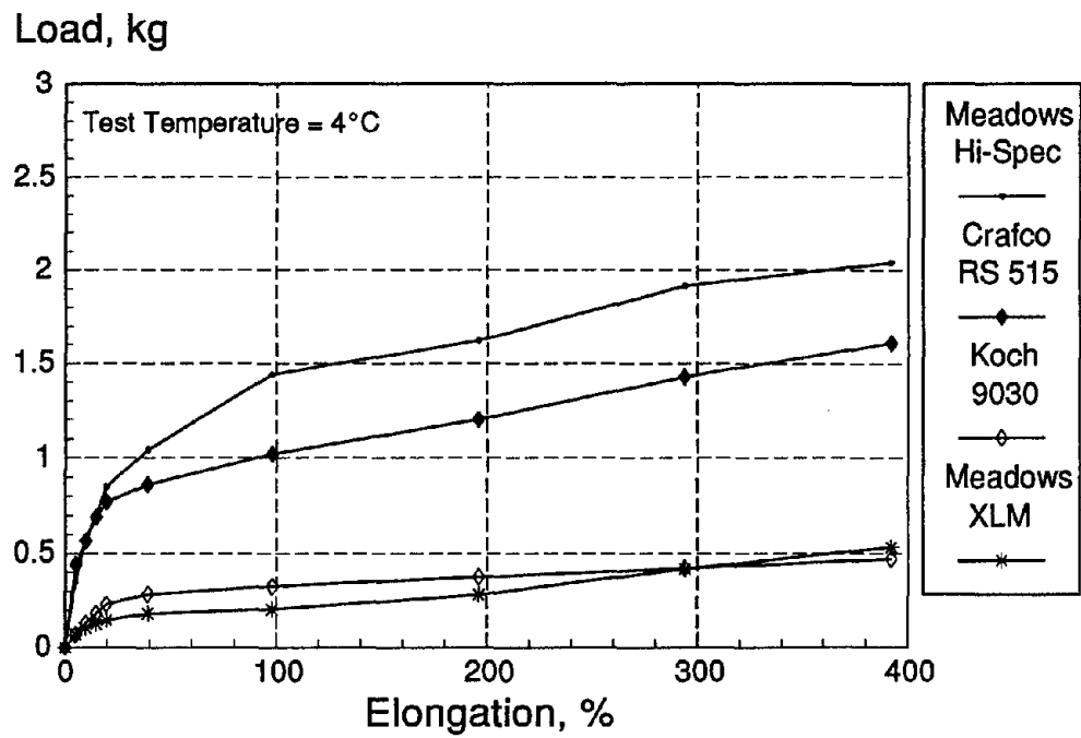
Figure 23. Load-elongation curves for modulus test conducted at 4°C.
