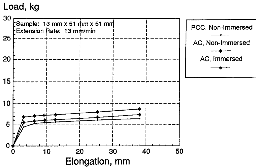
Figure C-7. ASTM D 3583 load-deformation curves for RS 515.
