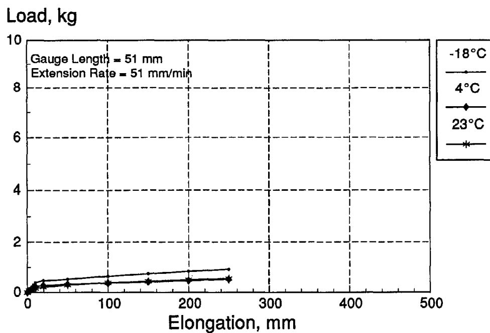
Figure C-3. ASTM D 412 load-deformation curves for 9030.
