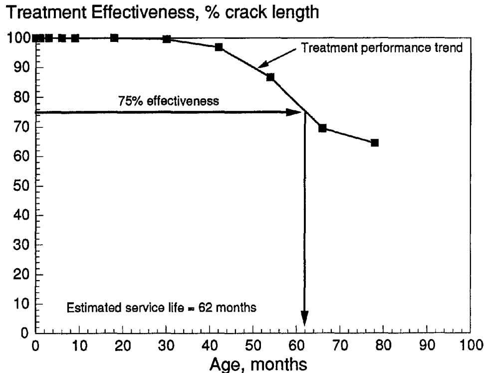
Figure 37. Illustration of service life estimation, based on 75 percent effectiveness.
