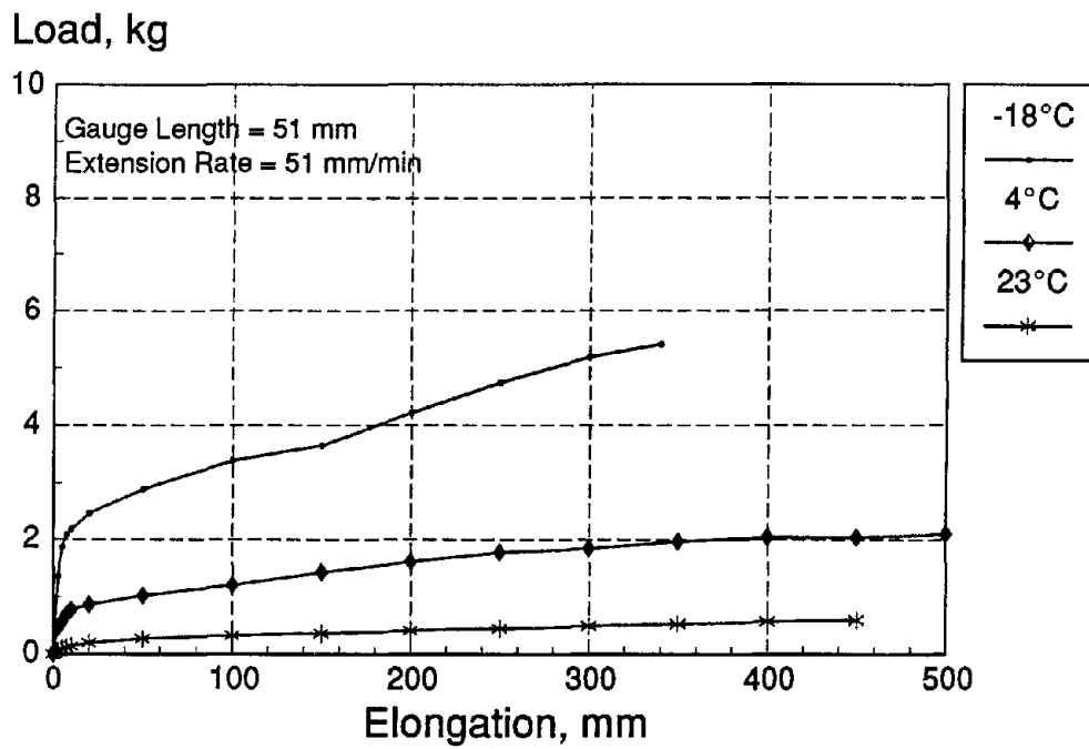
Figure C-2. ASTM D 412 load-deformation curves for RS 515.
