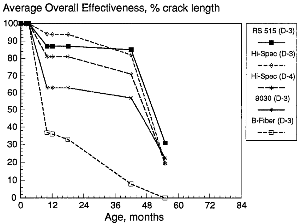
Figure 30. Time-series effectiveness trends of Wichita, KS adverse-conditions crack-seal treatments (continued).
