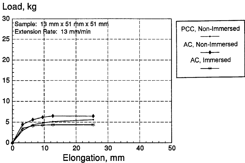
Figure C-8. ASTM D 3583 load-deformation curves for 9030.
