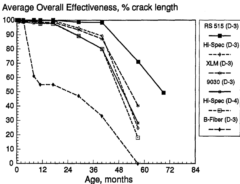
Figure 28. Time-series effectiveness trends of Abilene, TX crack-seal treatments (continued).
