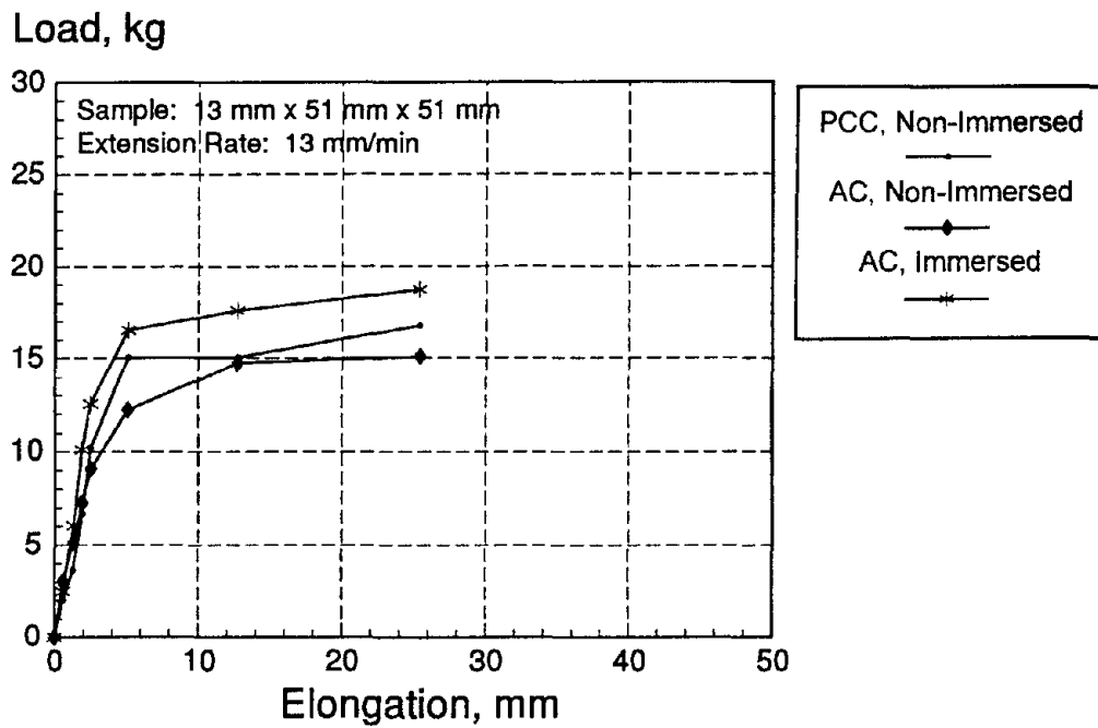
Figure C-10. ASTM D 3583 load-deformation curves for 890-SL,
