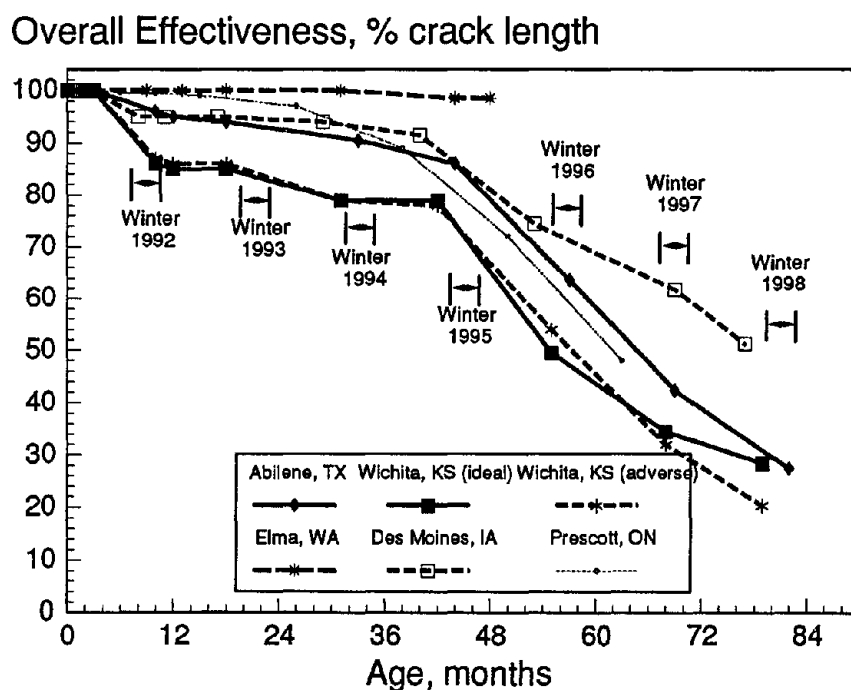
Figure 27. Overall performance trends of primary experimental treatments by site.
