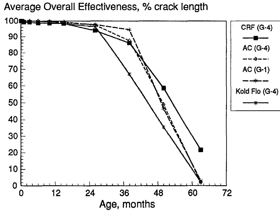
Figure 36. Time-series effectiveness trends of Prescott, ON crack-fill treatments (continued).
