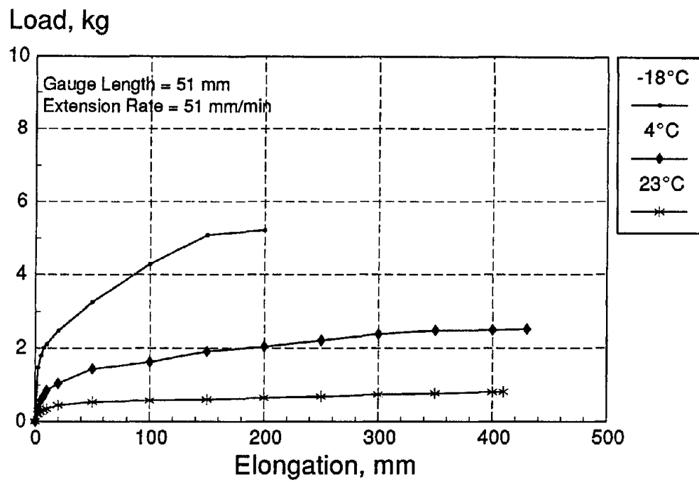
Figure C-1. ASTM D 412 load-deformation curves for Hi-Spec.
