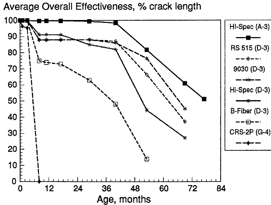
Figure 32. Time-series effectiveness trends of Des Moines, IA crack-seal treatments (continued).
