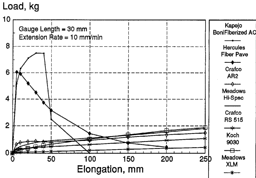
Figure 20. Force-ductility load-elongation curves for various primary materials.
