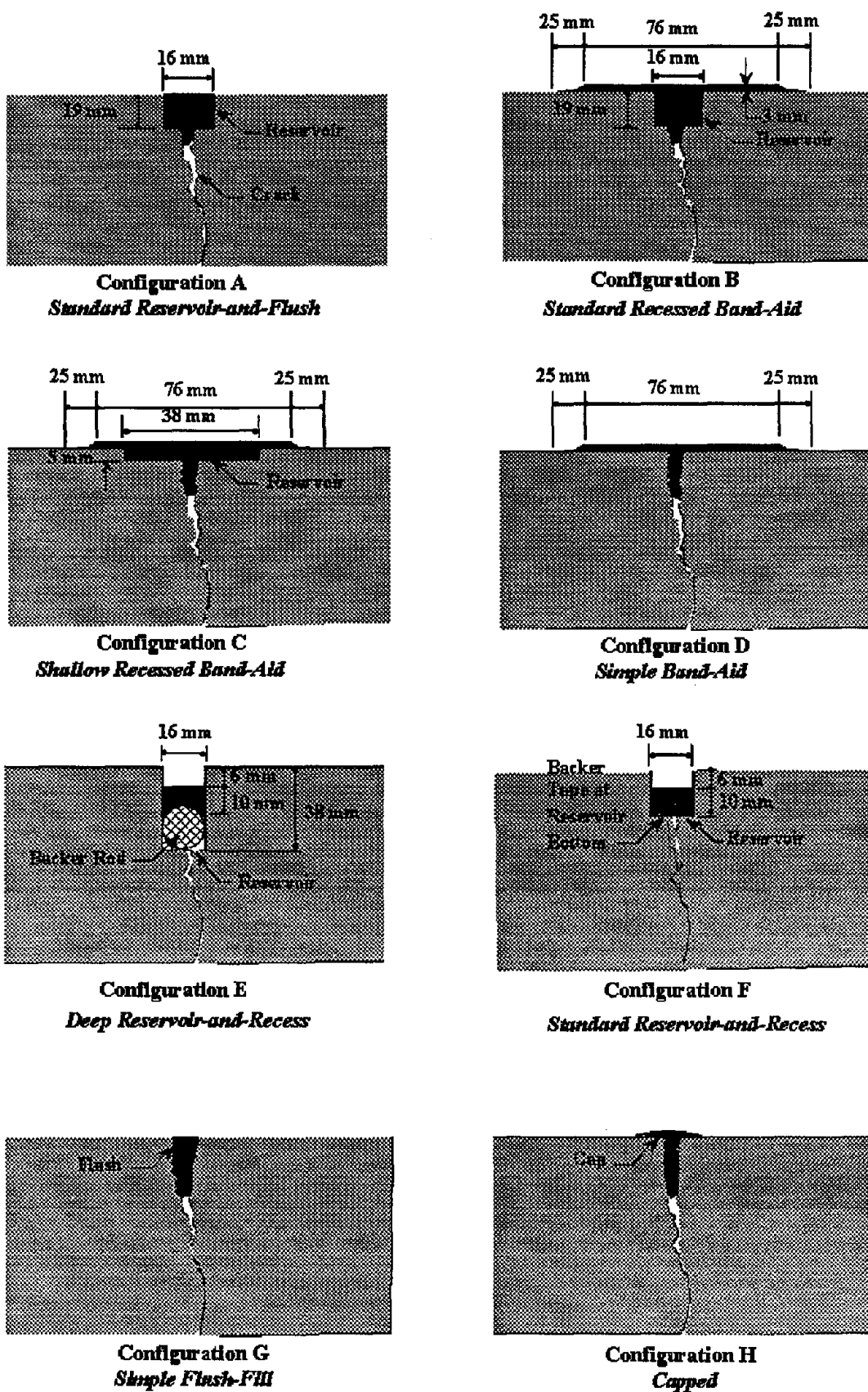
Figure 2. Material placement configurations for AC crack treatments.
