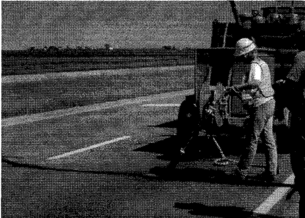
Figure 18. Hot airblasting using hot compressed-air (HCA) lance (crack preparation procedure 3).
