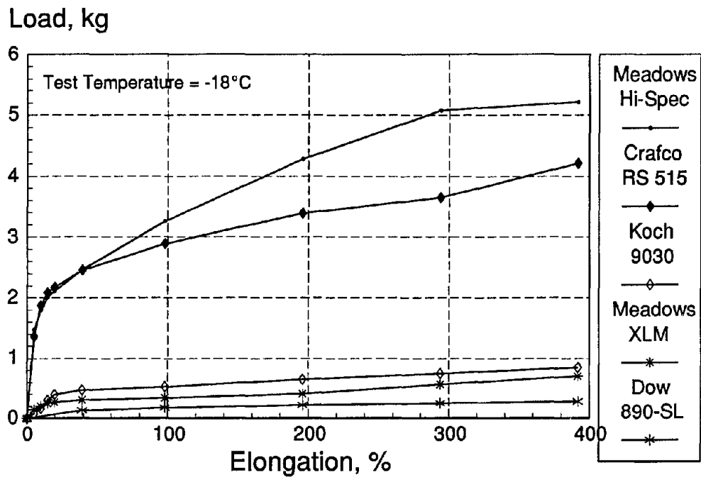
Figure 24. Load-elongation curves for modulus test conducted at -18°C.
