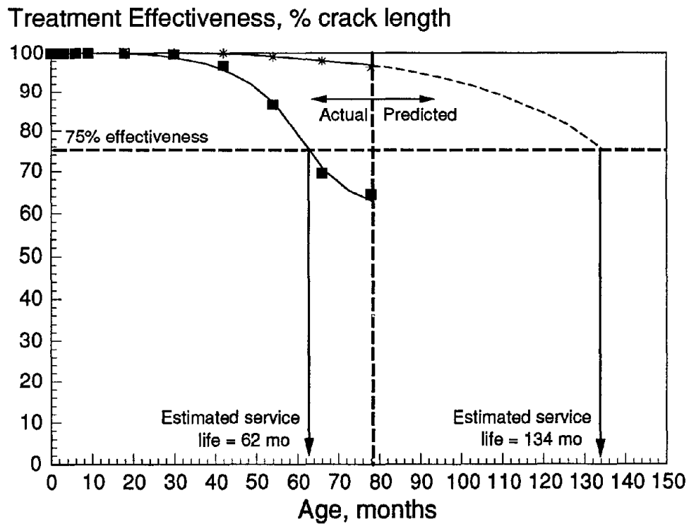
Figure 38. Illustration depicting estimates of actual versus predicted service lives.
