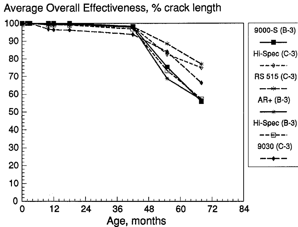
Figure 30. Time-series effectiveness trends of Wichita, KS adverse-conditions crack-seal treatments.
