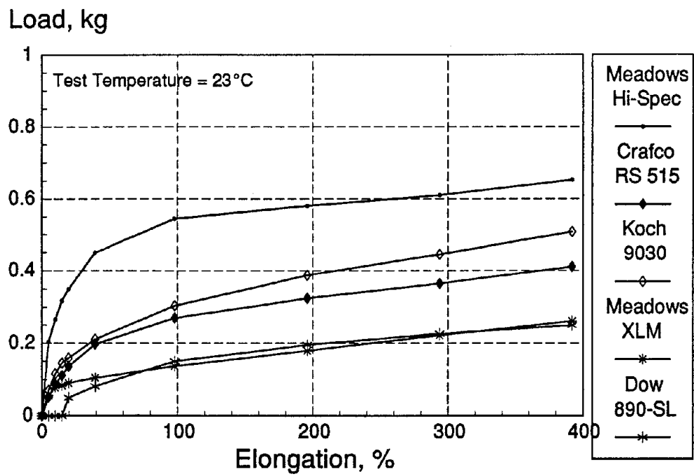
Figure 22. Load-elongation curves for modulus test conducted at 23°C.
