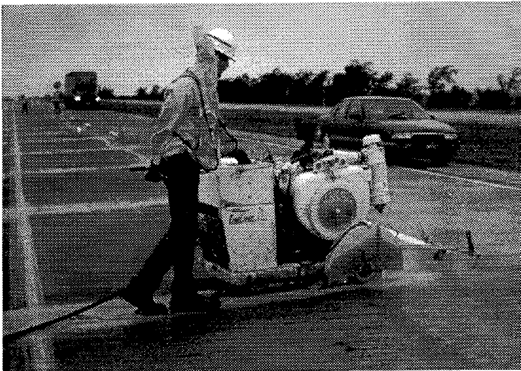
Figure 11. Joint-sawing operation.
