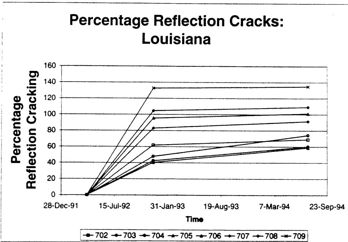
Figure 8. Percentage reflection cracks - Louisiana.
