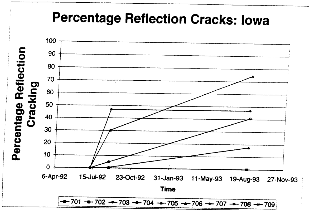
Figure 7. Percentage reflection cracks - Iowa.
