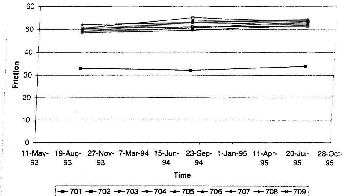
Figure 26. Average friction - Iowa.
