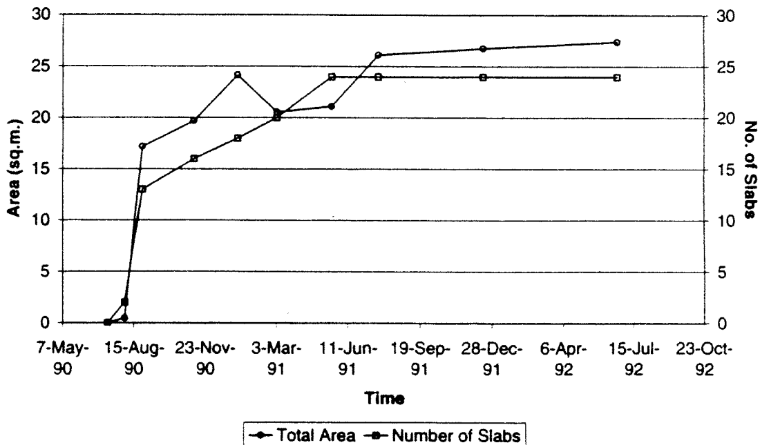
Figure 11. Delamination - Missouri (703).
