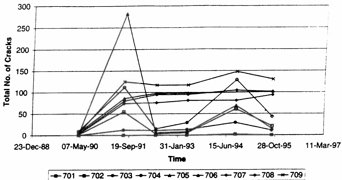
Figure 5. Total transverse cracks (PADIAS) - Missouri.
