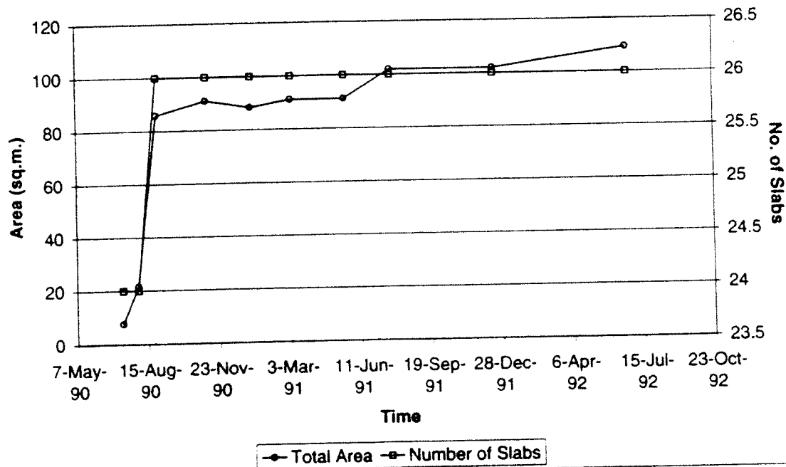
Figure 13. Delamination - Missouri (705).
