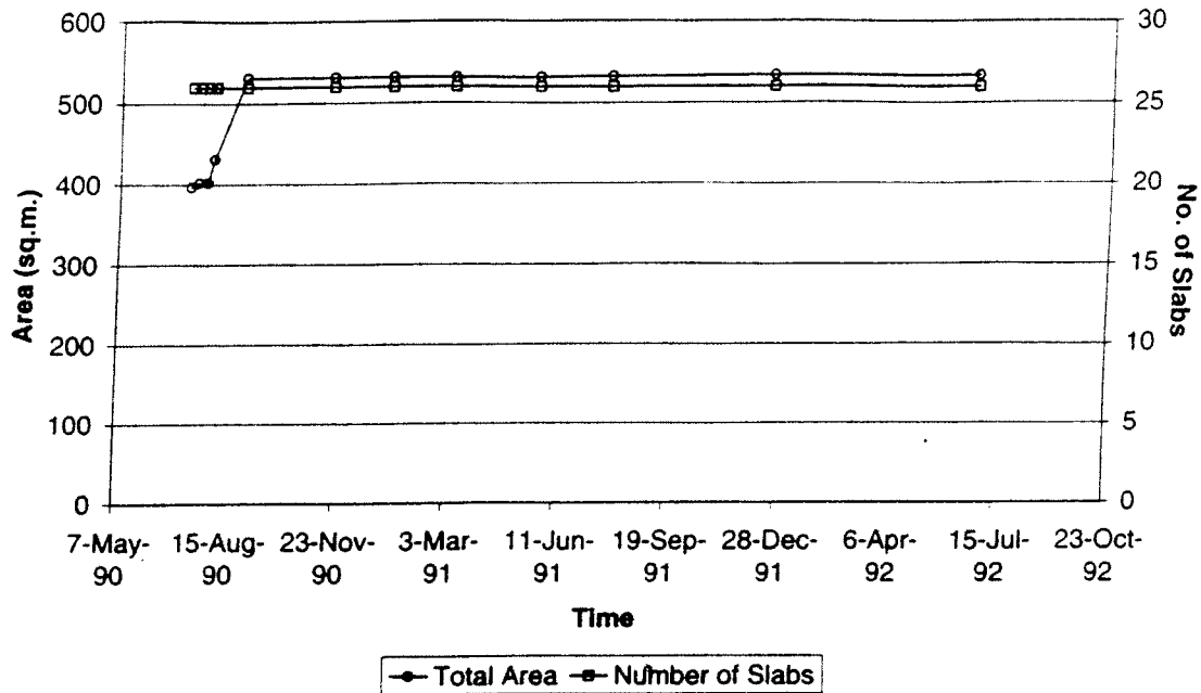
Figure 14. Delamination - Missouri (706).
