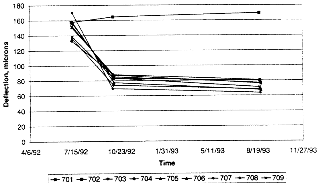
Figure 19. Maximum deflection - Iowa.
