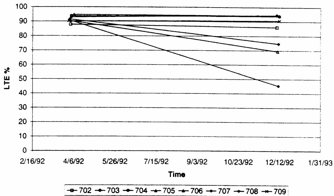
Figure 23. Load transfer efficiency - Louisiana.
