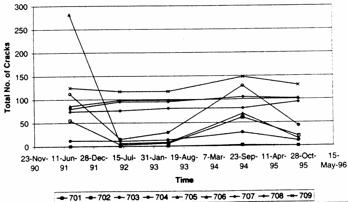
Figure 6. Total transverse cracks - Missouri.
