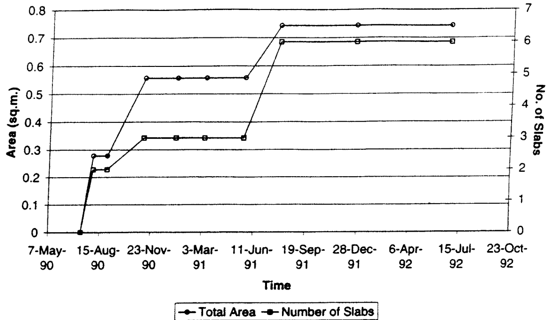
Figure 10. Delamination - Missouri (702).
