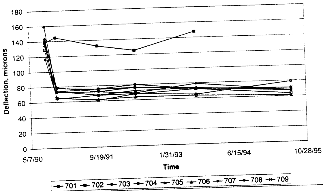
Figure 21. Maximum deflection - Minnesota.
