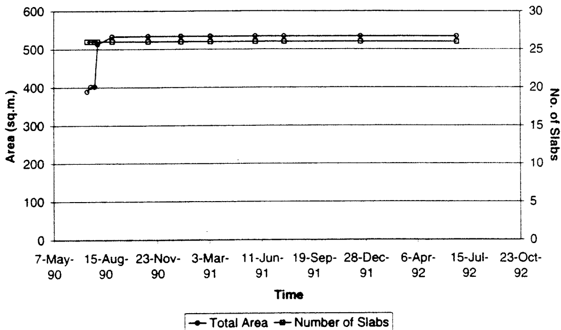
Figure 15. Delamination - Missouri (707).
