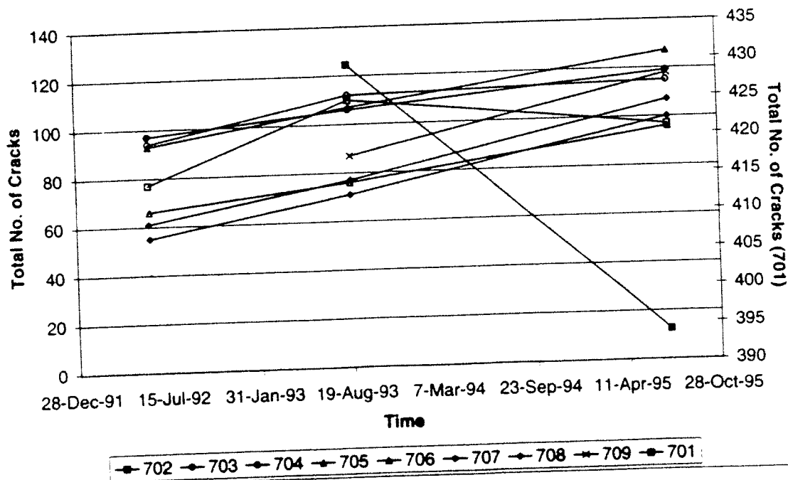
Figure 4. Total transverse cracks - Minnesota.
