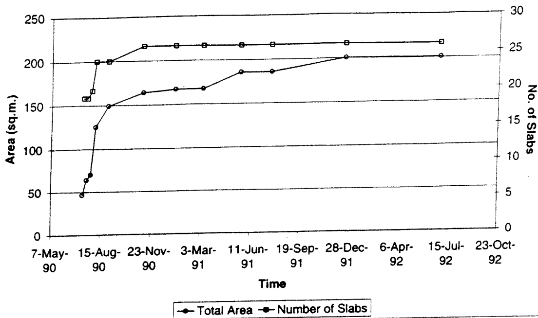
Figure 12. Delamination - Missouri (704).
