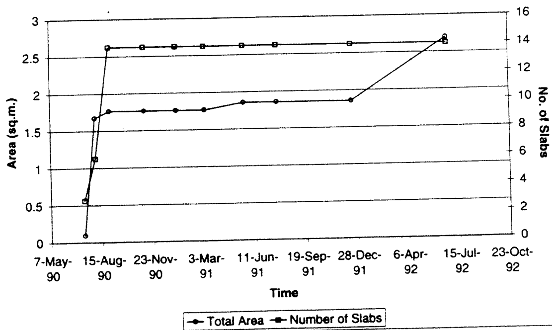
Figure 17. Delamination - Missouri (709).
