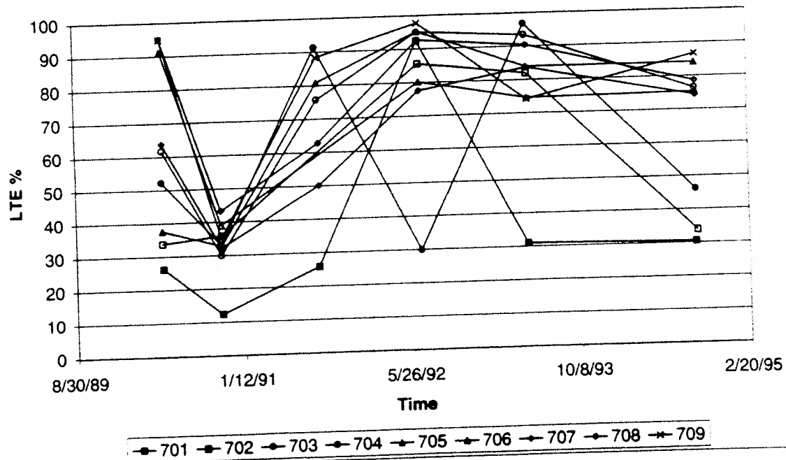
Figure 25. Load transfer efficiency - Missouri.
