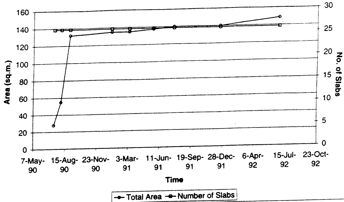
Figure 16. Delamination - Missouri (708).
