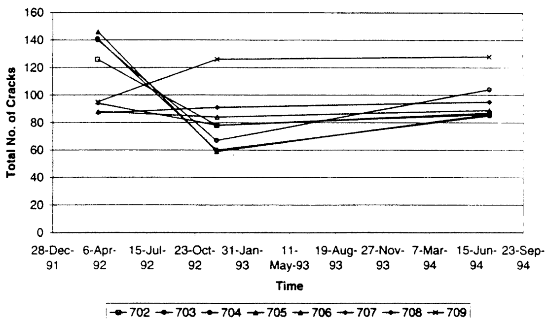
Figure 2. Total transverse cracks - Louisiana.
