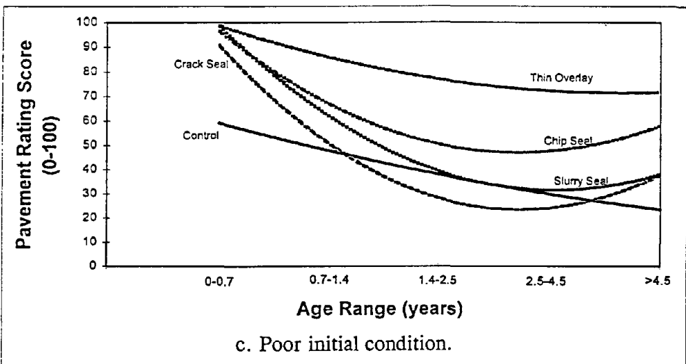
Figure 13. Pavement rating score (PRS) vs. age range by treatment type and initial condition for the wet-freeze environmental zone, post-construction data only.
