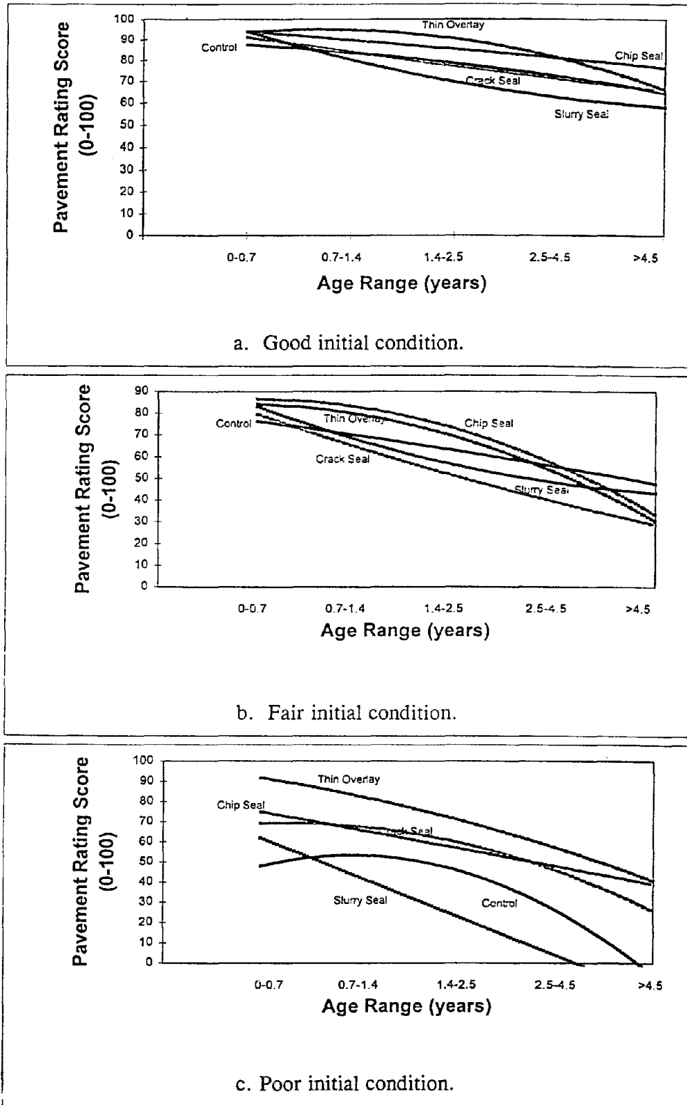
Figure 11. Pavement rating score (PRS) vs. age range by treatment type and initial condition for the dry-freeze environmental zone, post-construction data only.
