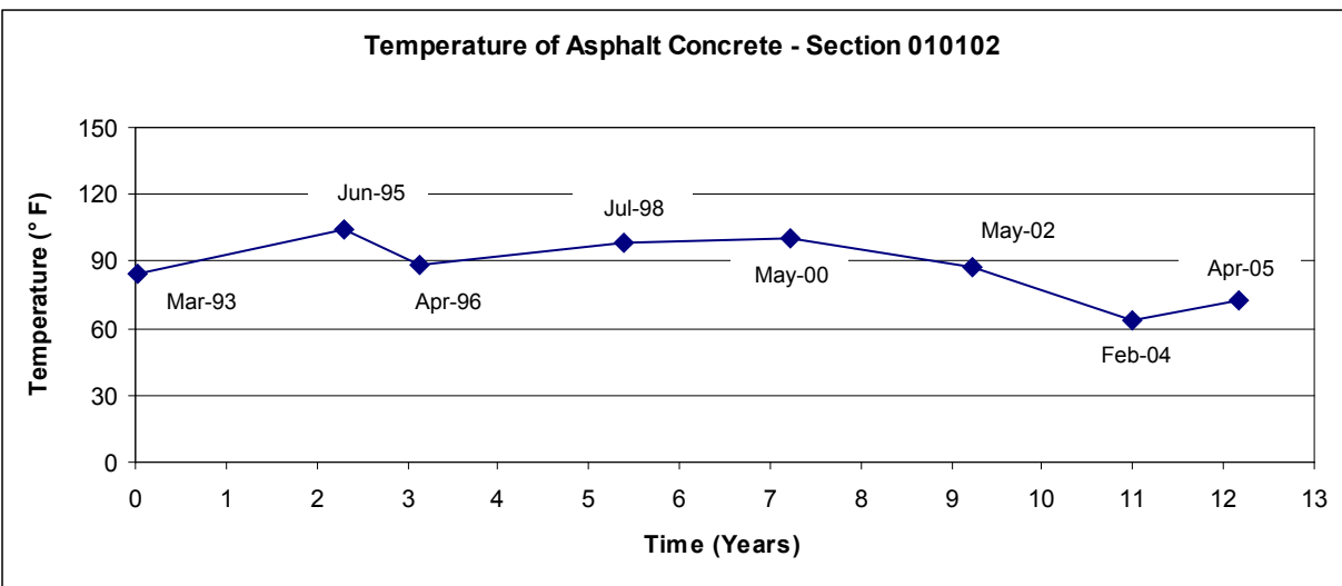
Figure 141. Graph. Mid-depth temperature of AC layer, section 010102 (Alabama).
