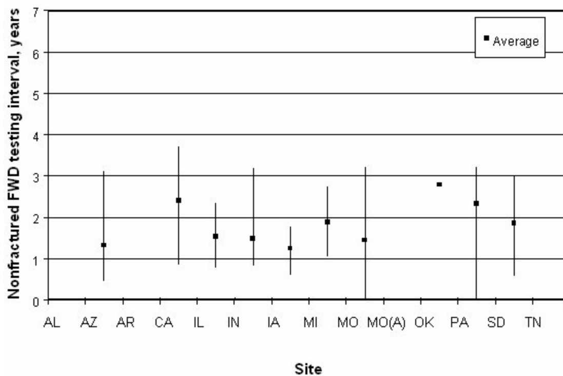
Figure 4. Nonfractured FWD testing intervals for each site.
