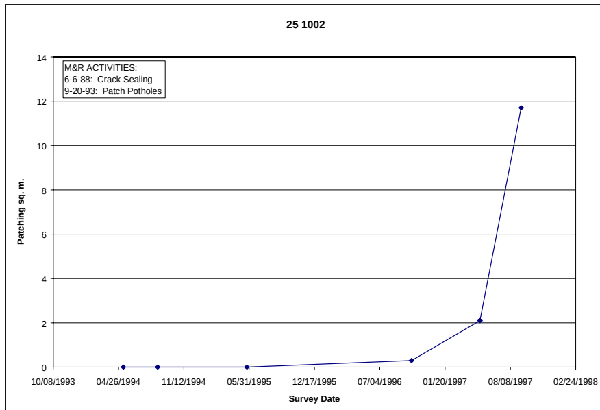
Figure 5. Discrepancy noted for test section 251002 – no area of patching recorded on 4/26/94 after potholes were patched on 9/20/93.
