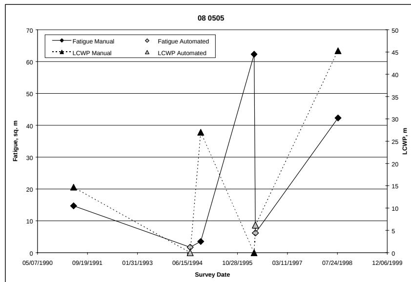
Figure 26. Examples of the difference between the automated and manual distress surveys for test section 080505.
