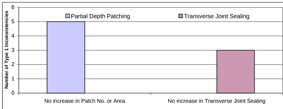
Figure 9. Distribution of JCP type 1 anomalies by type of treatment.
