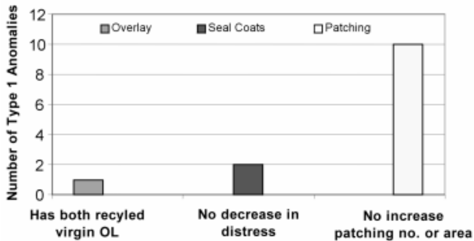
Figure 8. Distribution of HMA-surfaced pavements with type 1 anomalies by type of treatment.
