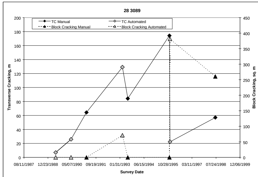
Figure 27. Examples of the difference between the automated and manual surveys for test section 283089.
