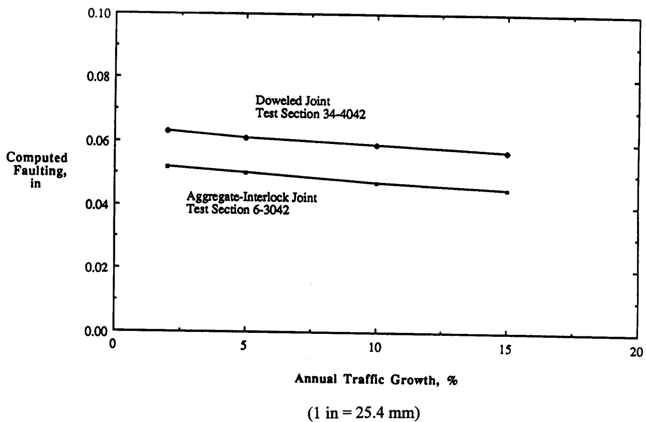
Figure 25. Sensitivity analysis of annual traffic growth rate on computed faulting.
