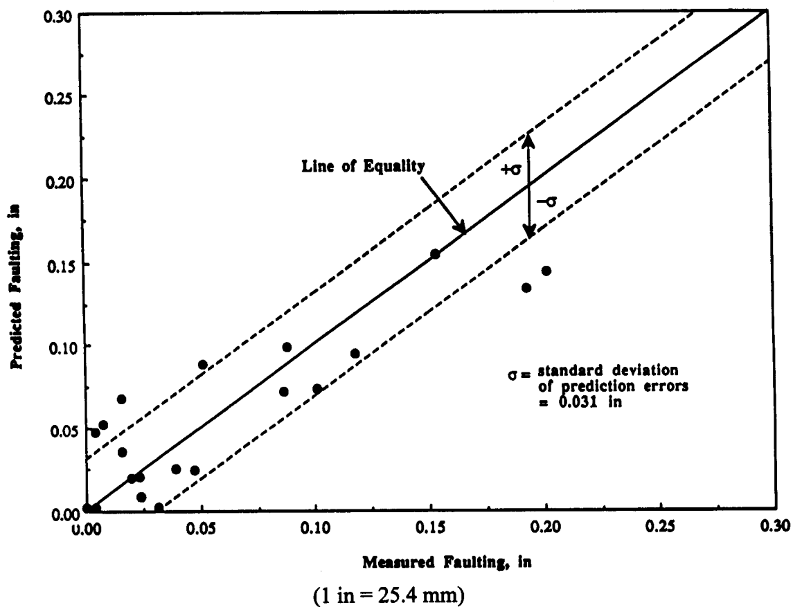
Figure 22. Predicted faulting versus measured faulting for aggregate-interlock joints.
