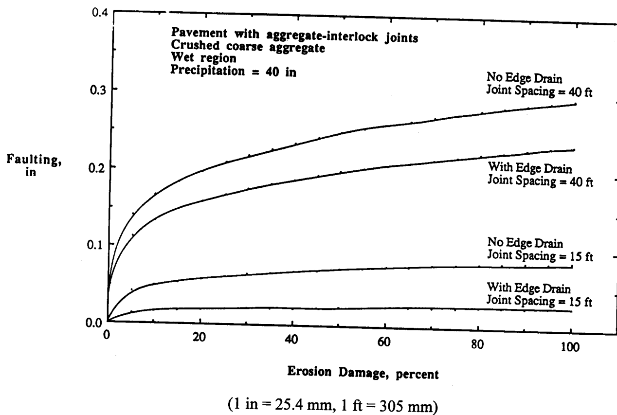
Figure 17. Faulting versus accumulated erosion for aggregate-interlock joints with crushed coarse aggregate in wet region.
