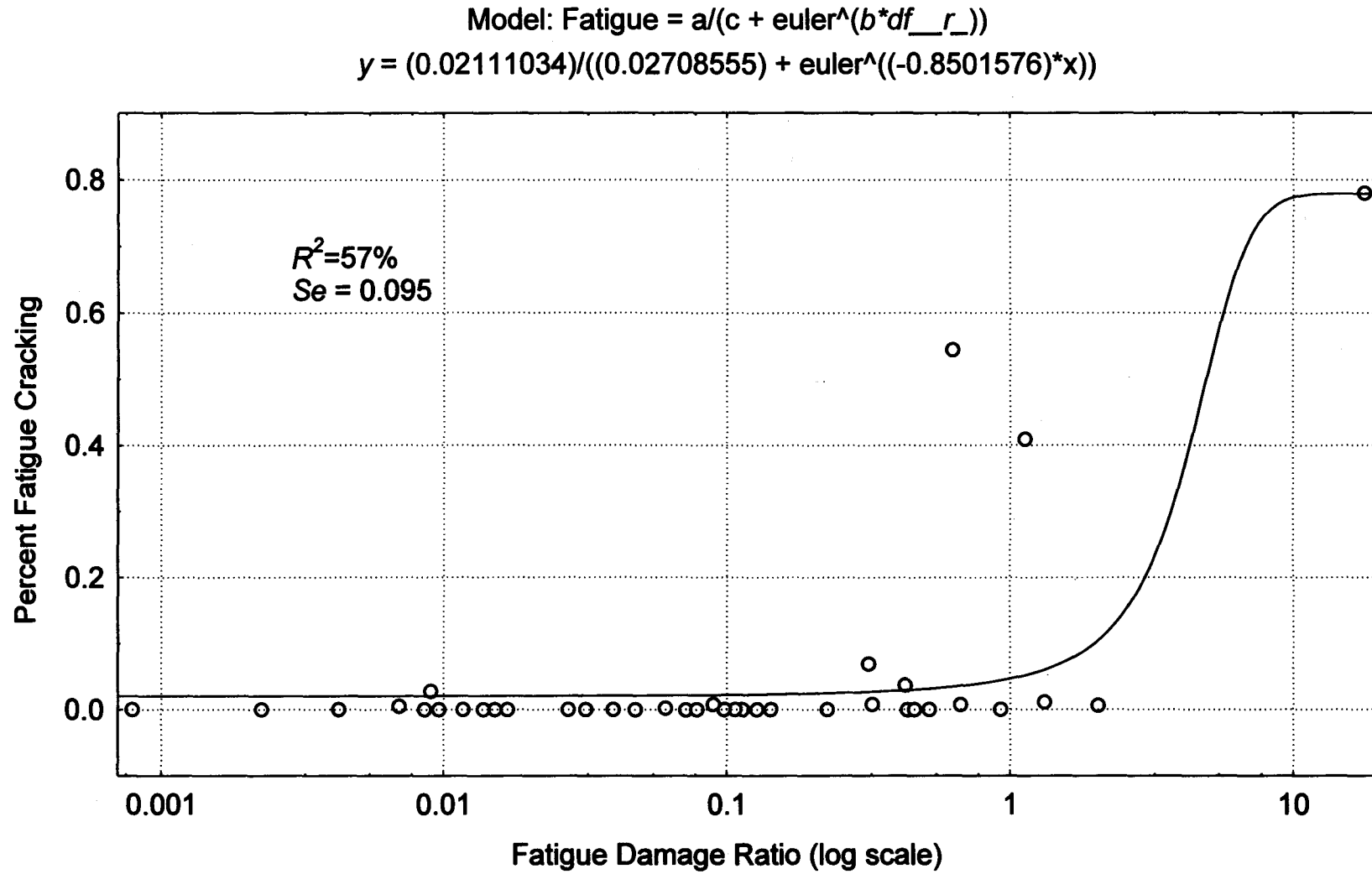
Figure 8. Constrained growth model.
