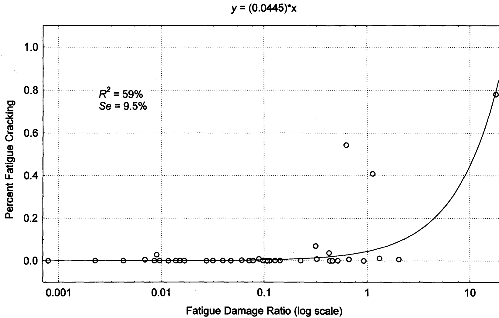
Figure 10. Linear model.
