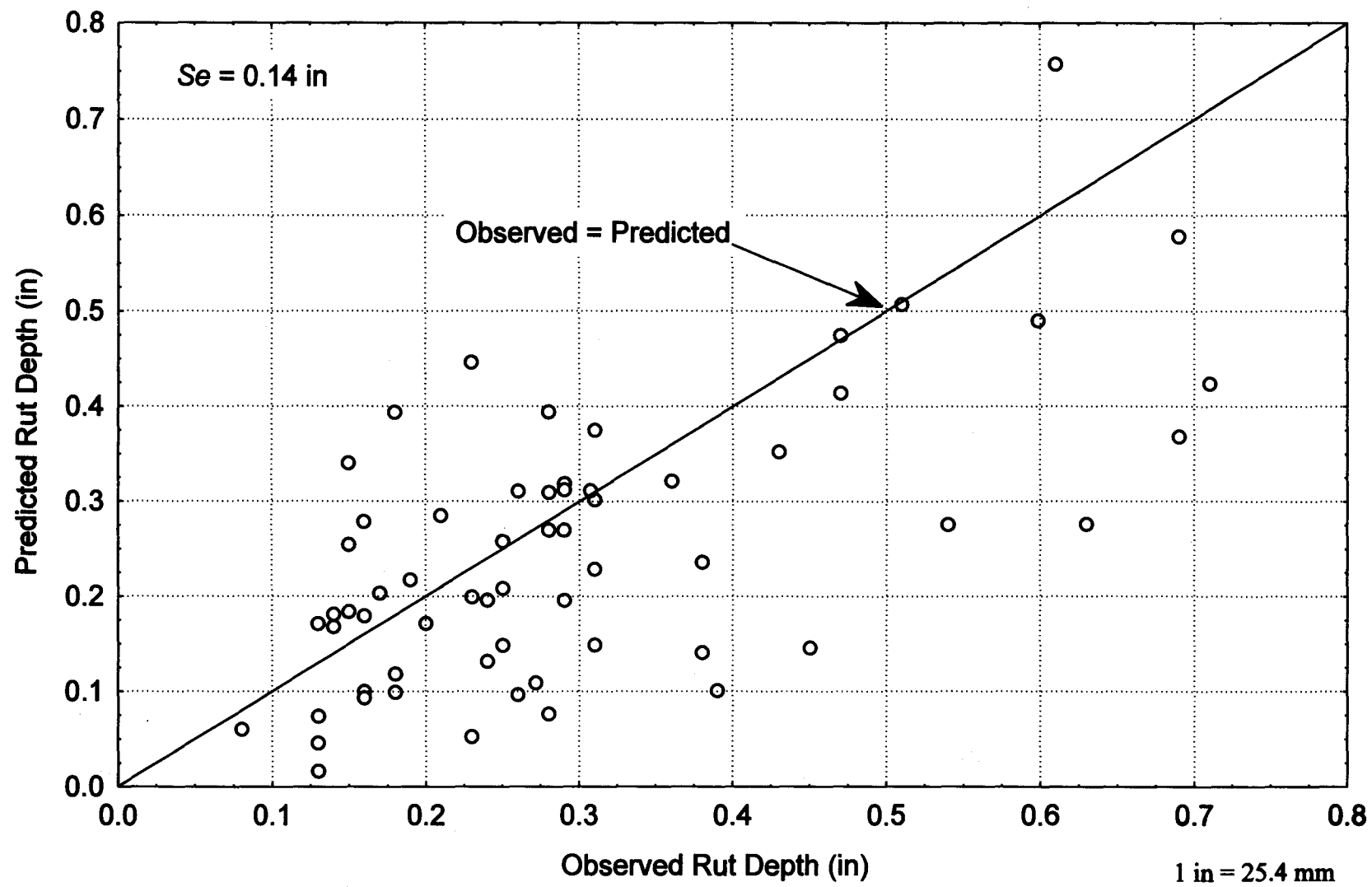
Figure 25. Observed versus predicted rut depth, based on validation data set.
