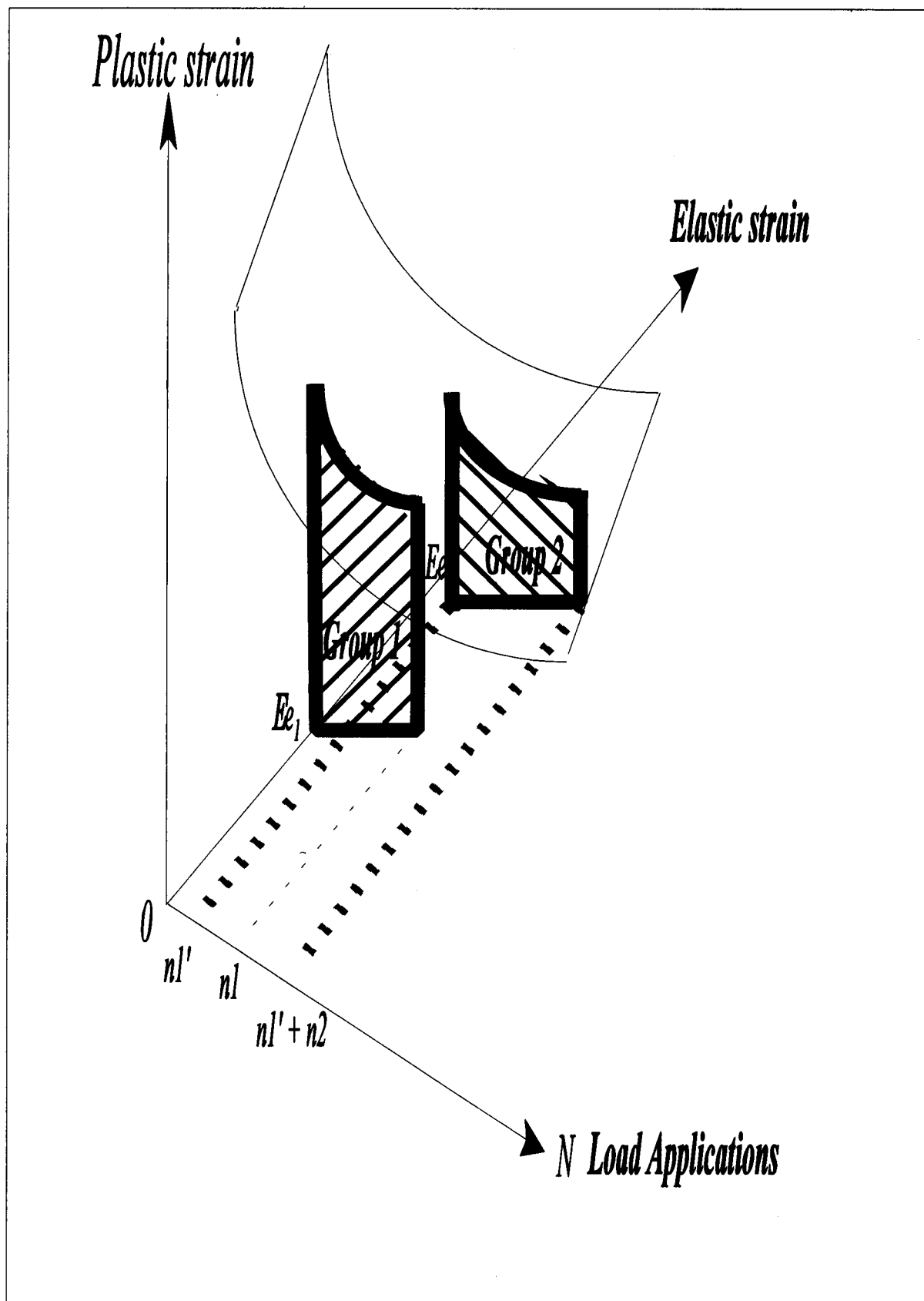
Figure 22. Three-dimensional strain model.
