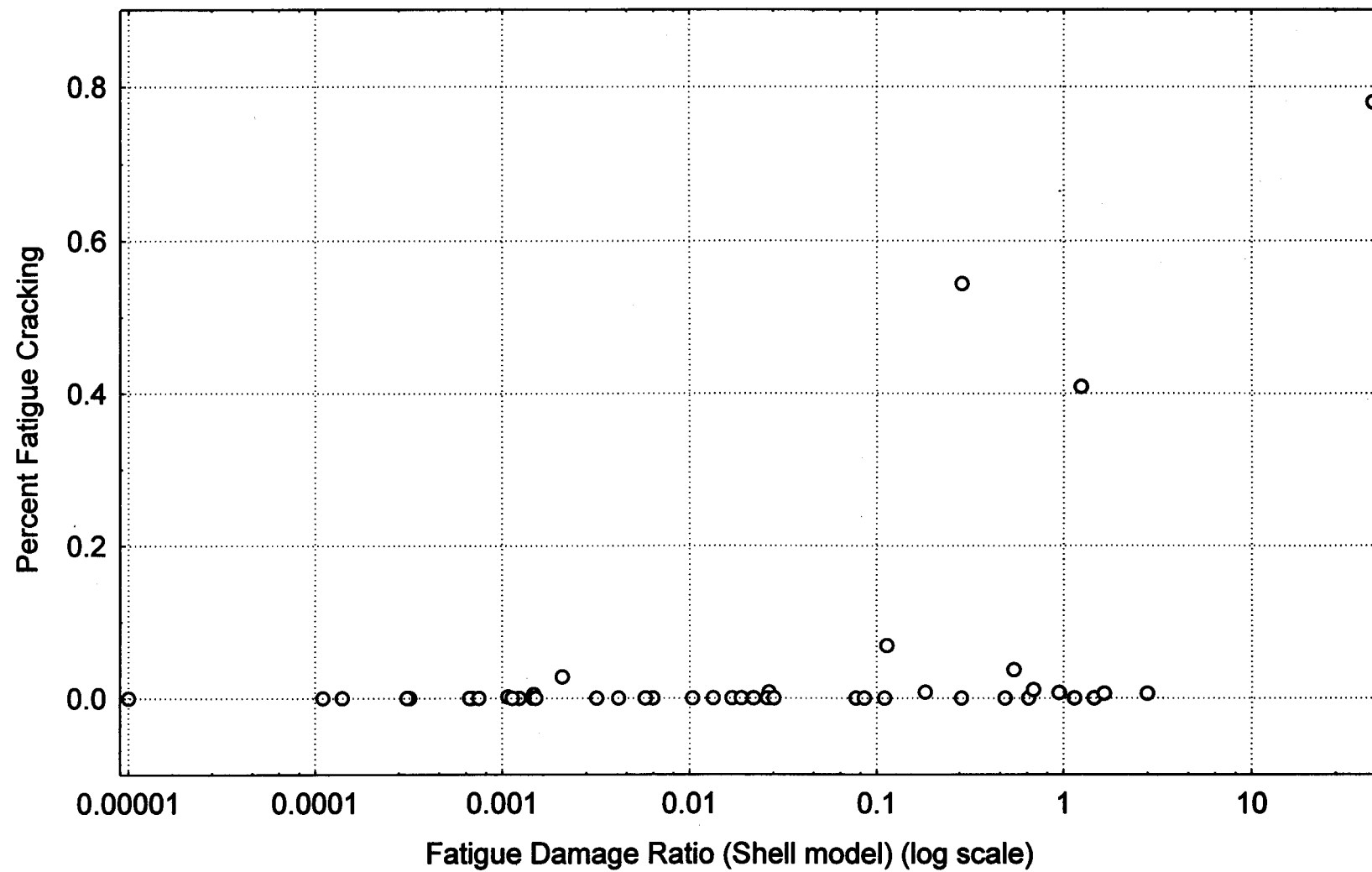
Figure 16. The Shell fatigue model, GPS-1 sections.
