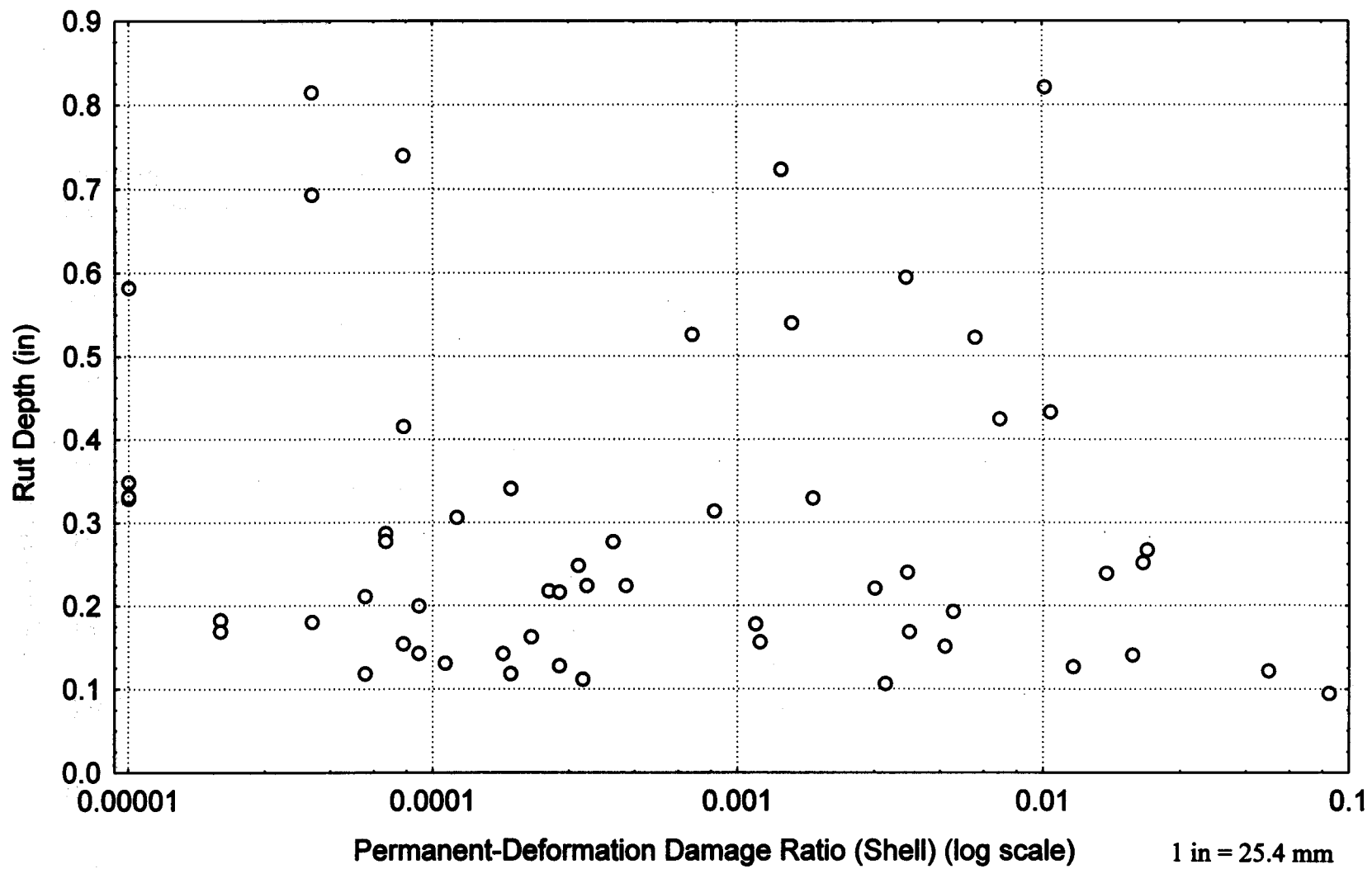
Figure 18. Shell rutting model, GPS-1 sections.
