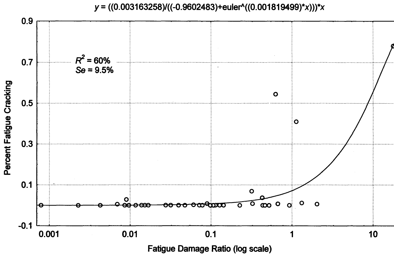
Figure 9. Modified constrained growth model.
