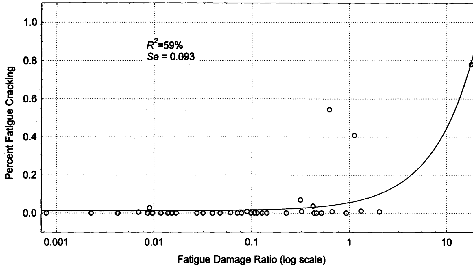
Figure 11. Exponential growth model.
