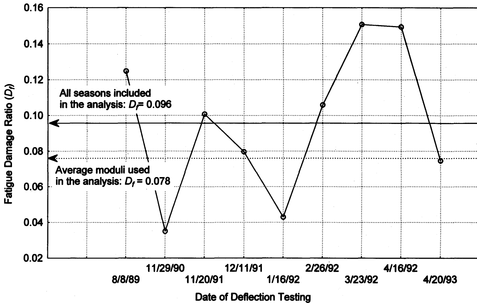
Figure 20. Seasonal variation effects on fatigue damage ratio.
