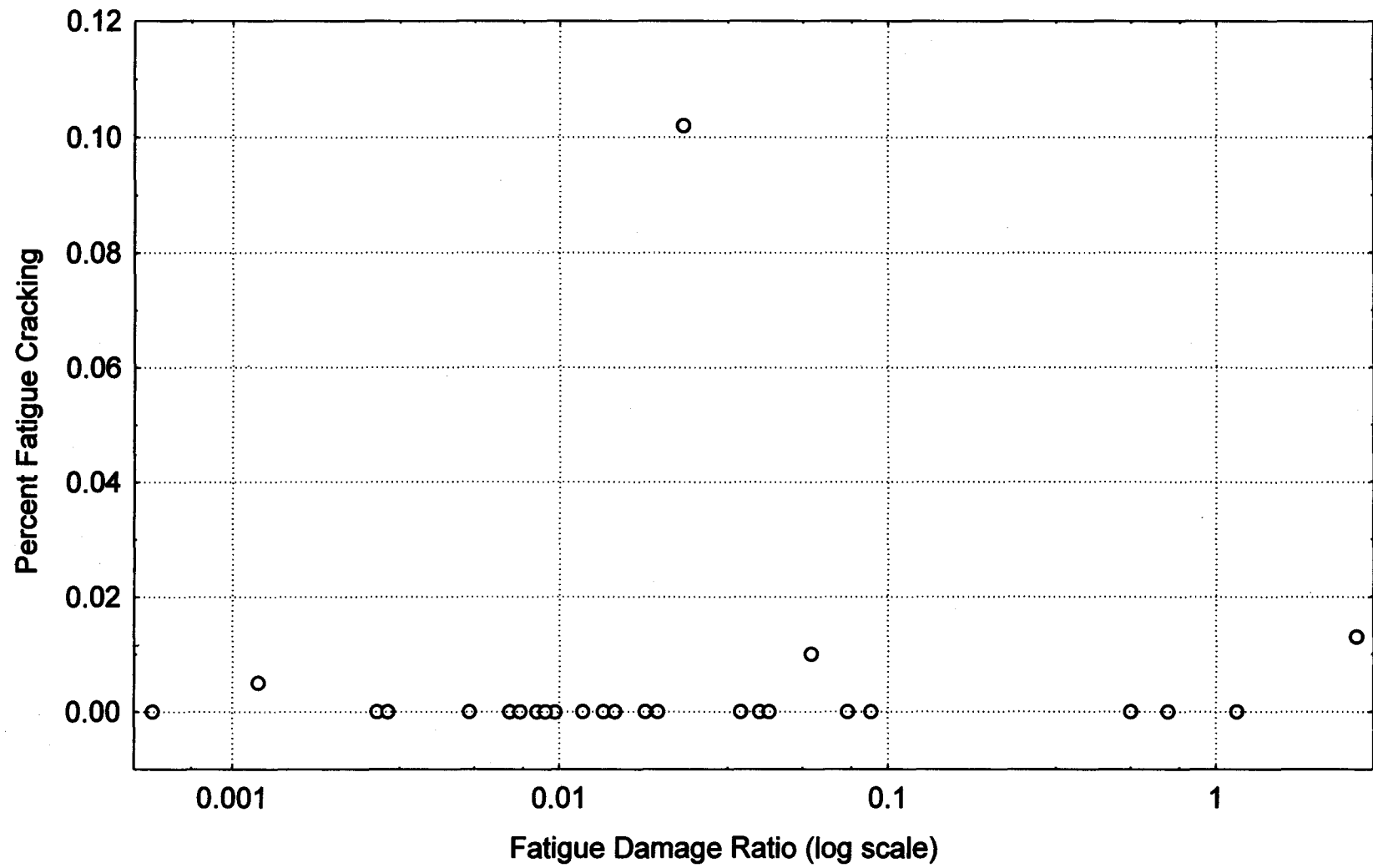
Figure 12. Fatigue damage versus fatigue cracking for GPS-2.
