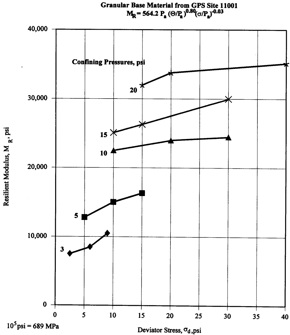
Figure 3. Example of repeated load triaxial resilient modulus test results of a granular base material.
