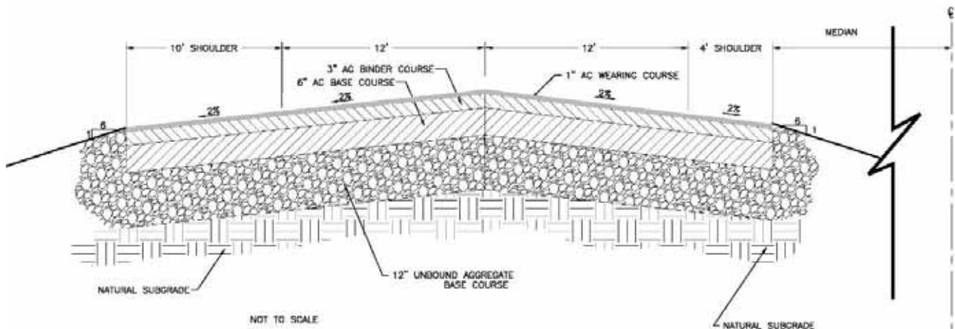
Figure 70. Diagram. Interstate highway, left section.
