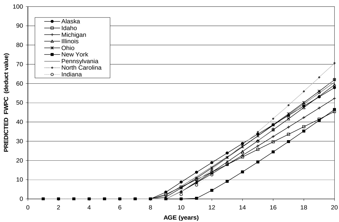
Figure 63. Scatter graph. Flexible pavement FWPC for selected sites in each agency.
