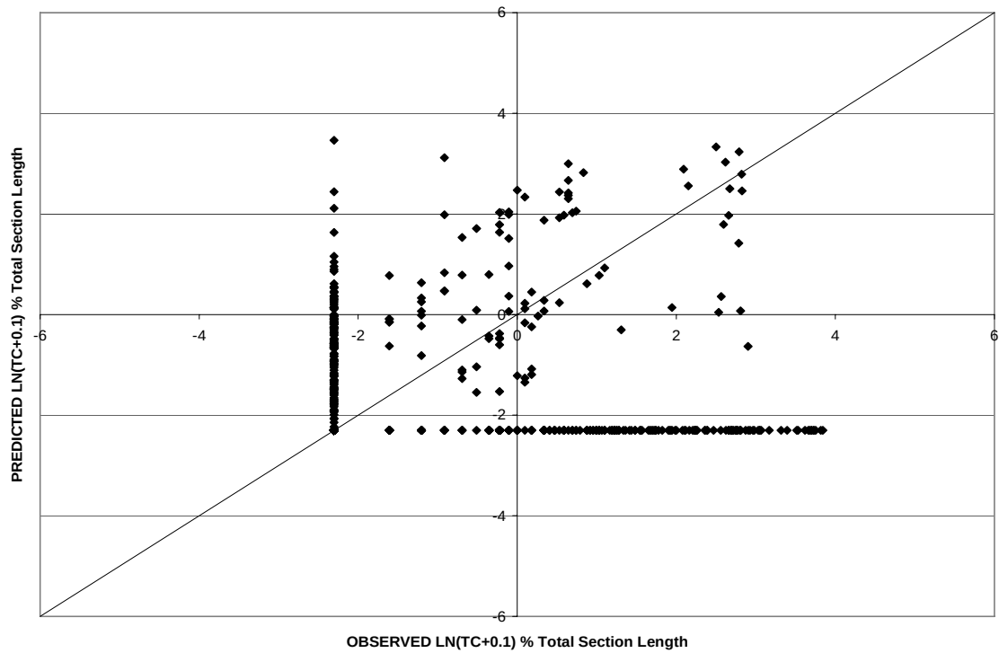
Figure 35. Scatter plot. TC model for rigid pavements with linear TC-age relationship.
