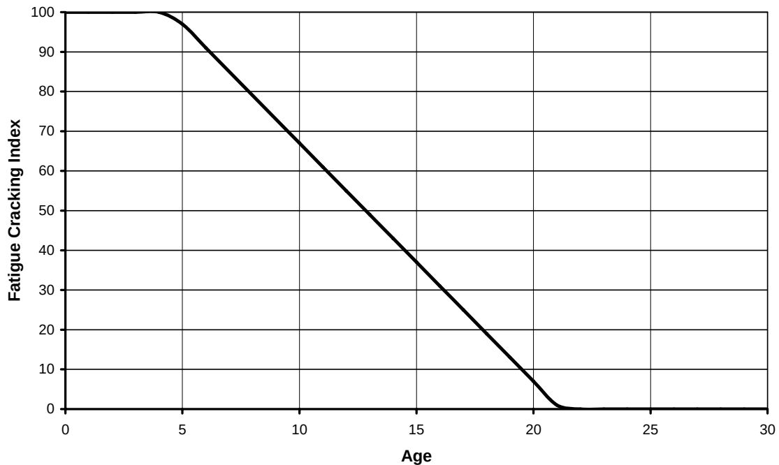
Figure 81. Chart. Fatigue cracking index trend for environmental case wet no-freeze.
