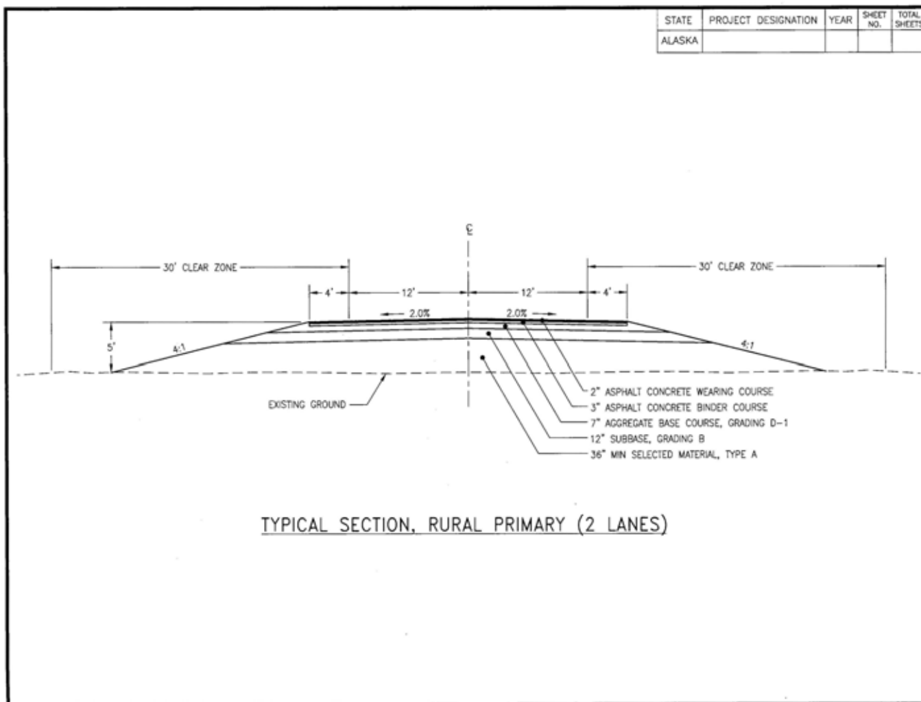
Figure 92. Diagram. Typical section for rural primary (2 lanes) in Alaska.
