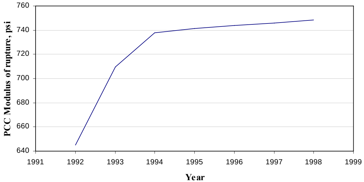
Figure 3. Estimated strength development of GADOT mix.
