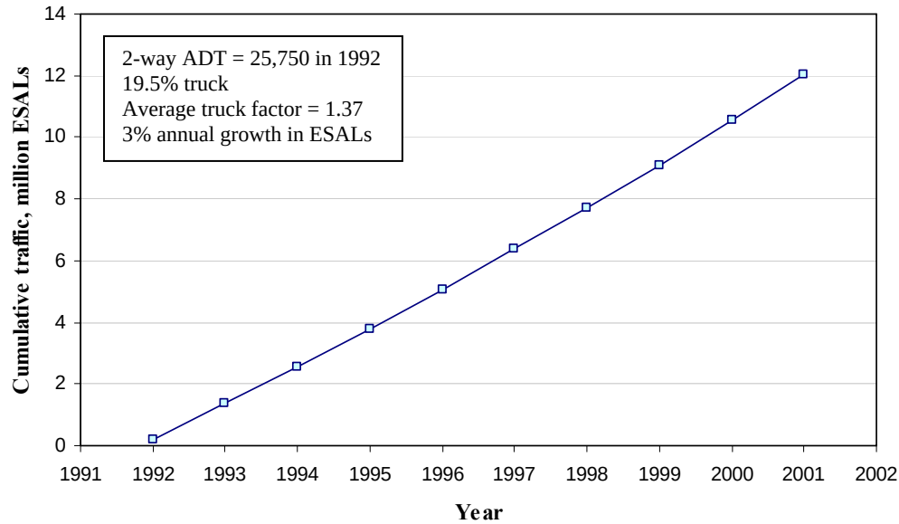
Figure 1. Estimated traffic on Georgia site.
