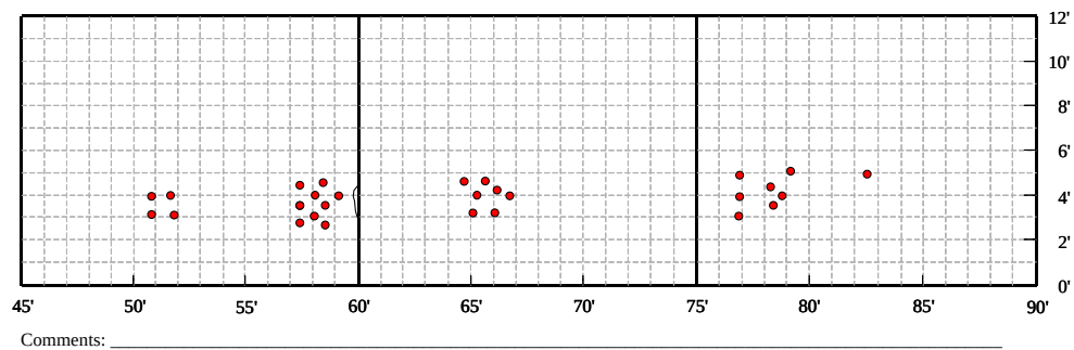
Figure 26. Graph. Distress map for patch NC-1 in North Carolina—1998.
