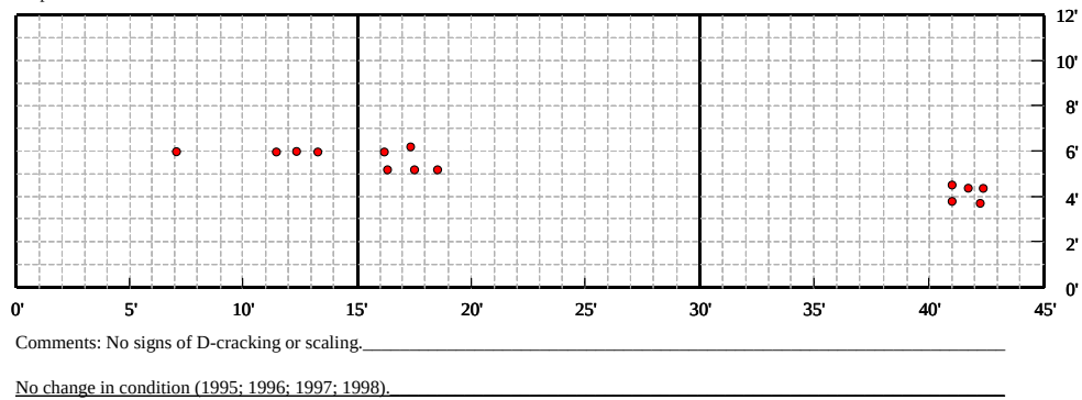
Figure 25. Graph. Distress map for patch NC-1 in North Carolina—1994.
