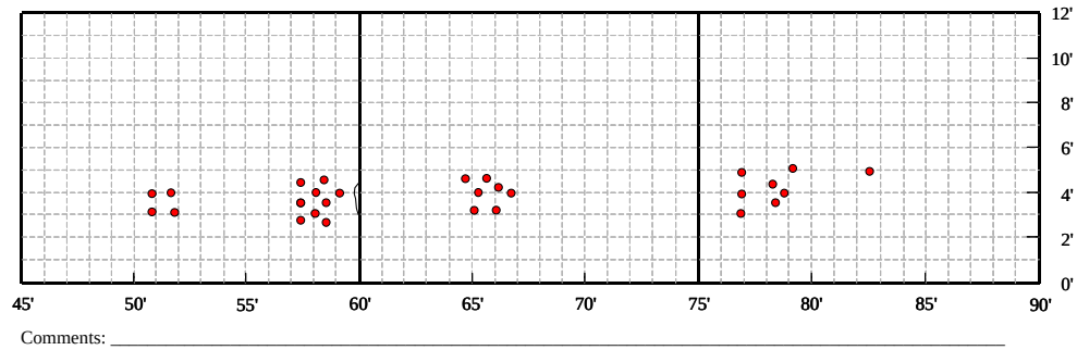
Figure 25. Graph. Distress map for patch NC-1 in North Carolina—1994.
