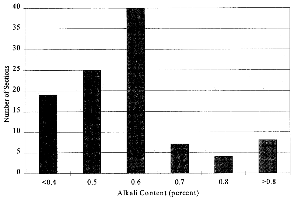
Figure 52. Distribution of PCC alkali content.
