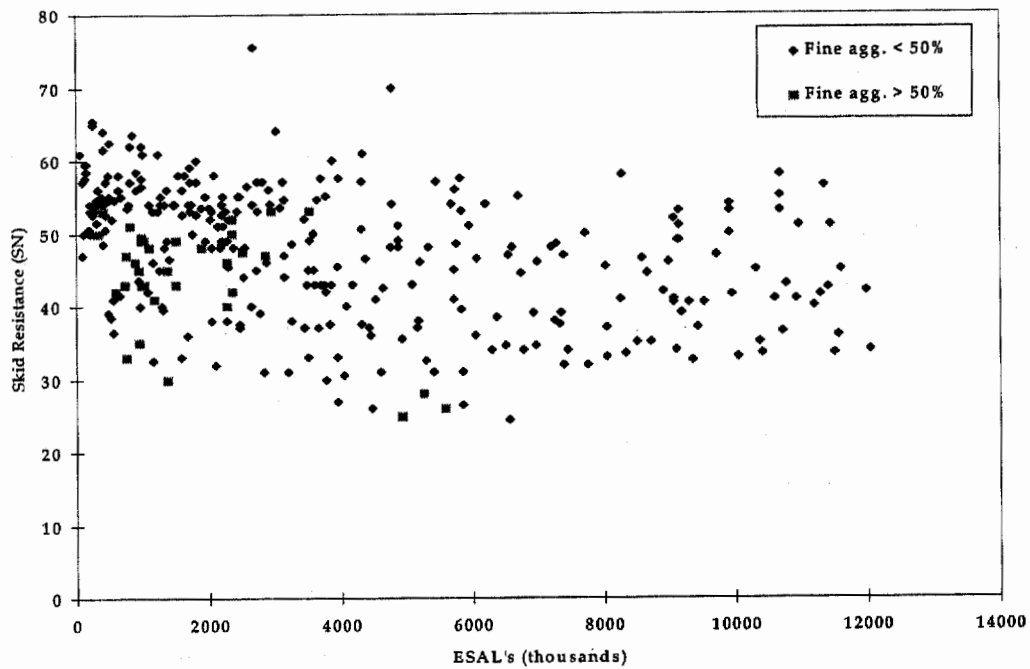
Figure 31. Plot of skid number versus ESAL's showing effect of percentage of fine aggregate.
