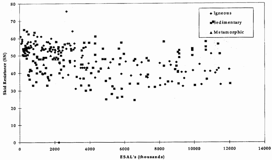
Figure 27. Plot of skid number versus ESAL's for PCC-surfaced pavements showing effect of coarse aggregate geologic classifications.
