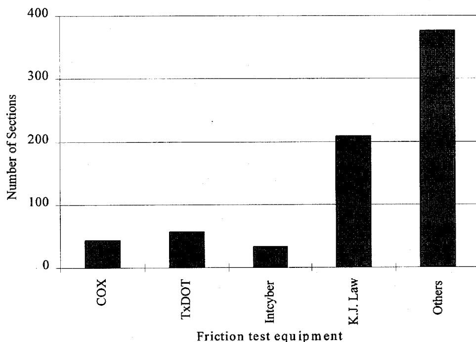
Figure 34. Friction test equipment type used for LTPP data collection.
