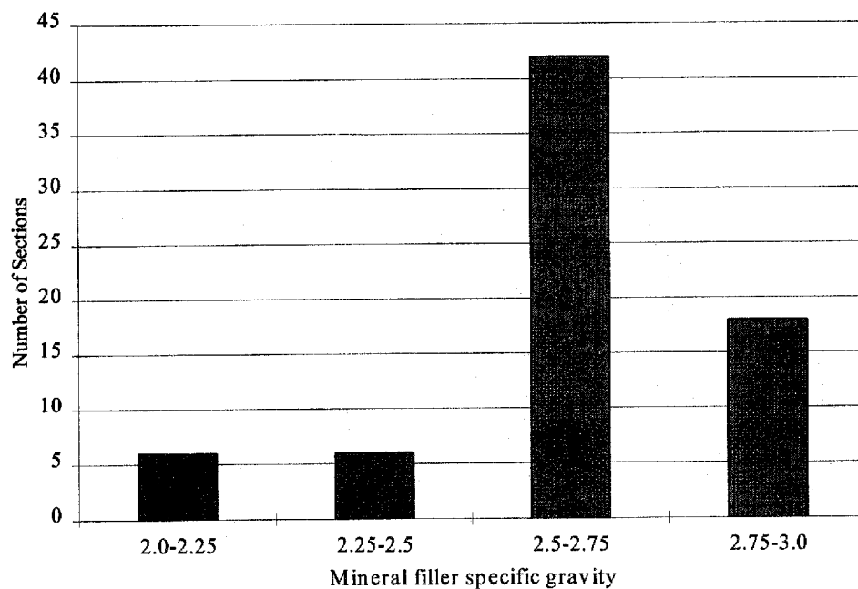
Figure 39. Histogram of mineral filler specific gravity values in AC surface mixture.
