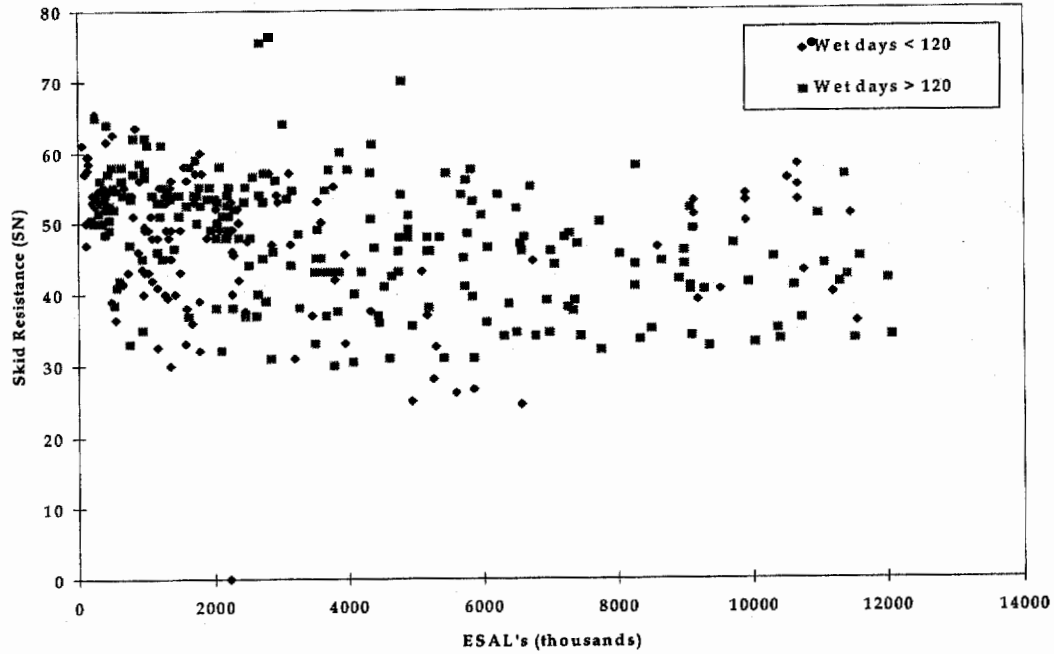
Figure 26. Plot of skid number versus ESAL's for PCC-surfaced pavements showing effect of wet days.
