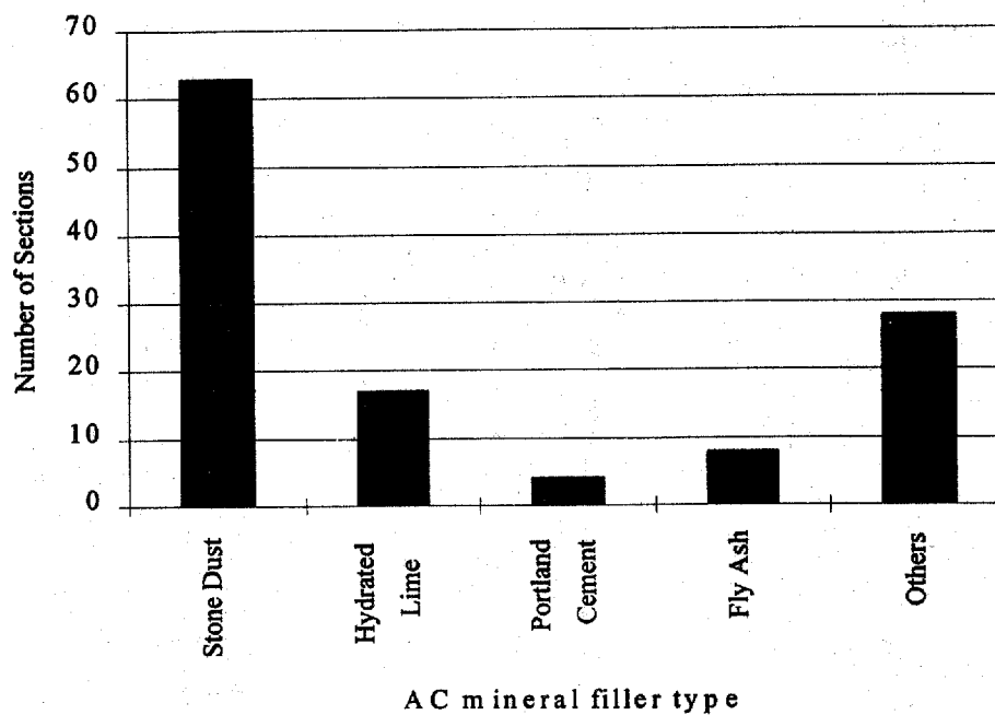
Figure 38. Histogram of mineral filler type used in AC surface mixture.
