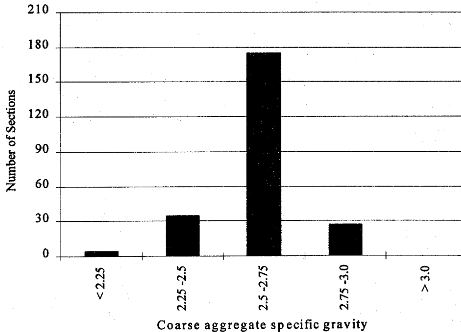
Figure 36. Histogram of available specific gravity values for coarse aggregate used in AC surface mixture.
