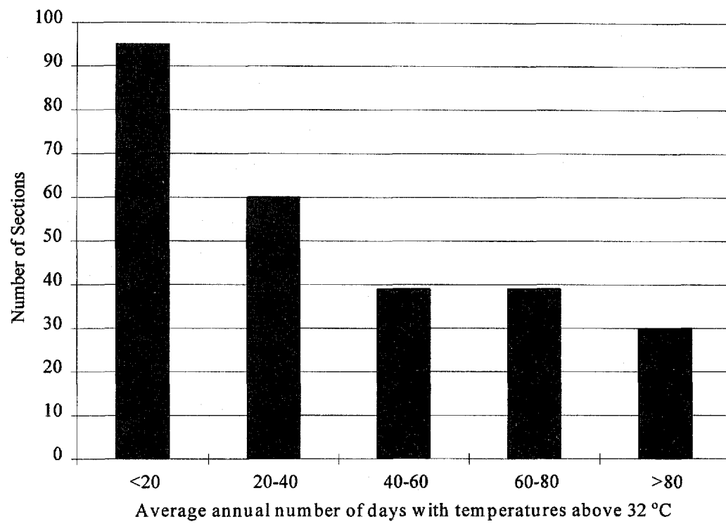
Figure 63. Average annual number of days with temperatures above 32 °C for all PCC-surfaced pavements evaluated.
