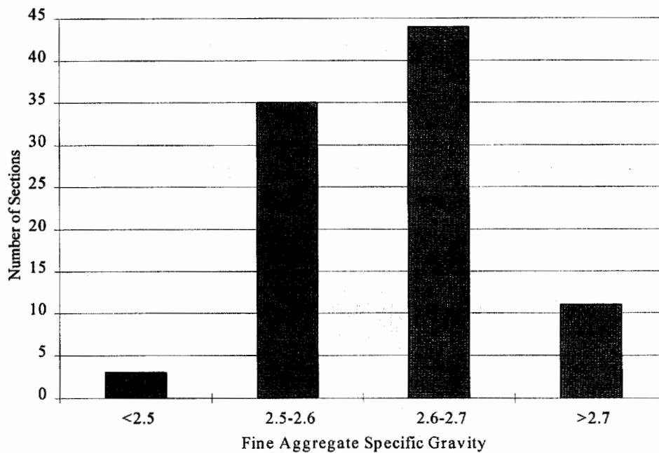
Figure 56. Distribution of PCC fine aggregate specific gravity.
