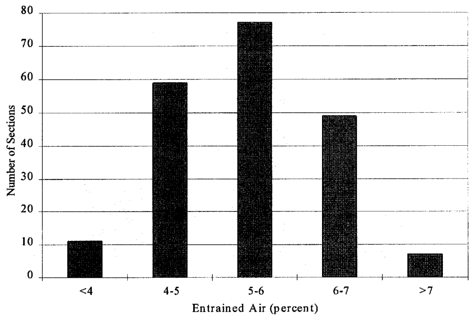
Figure 53. Distribution of PCC entrained air content.
