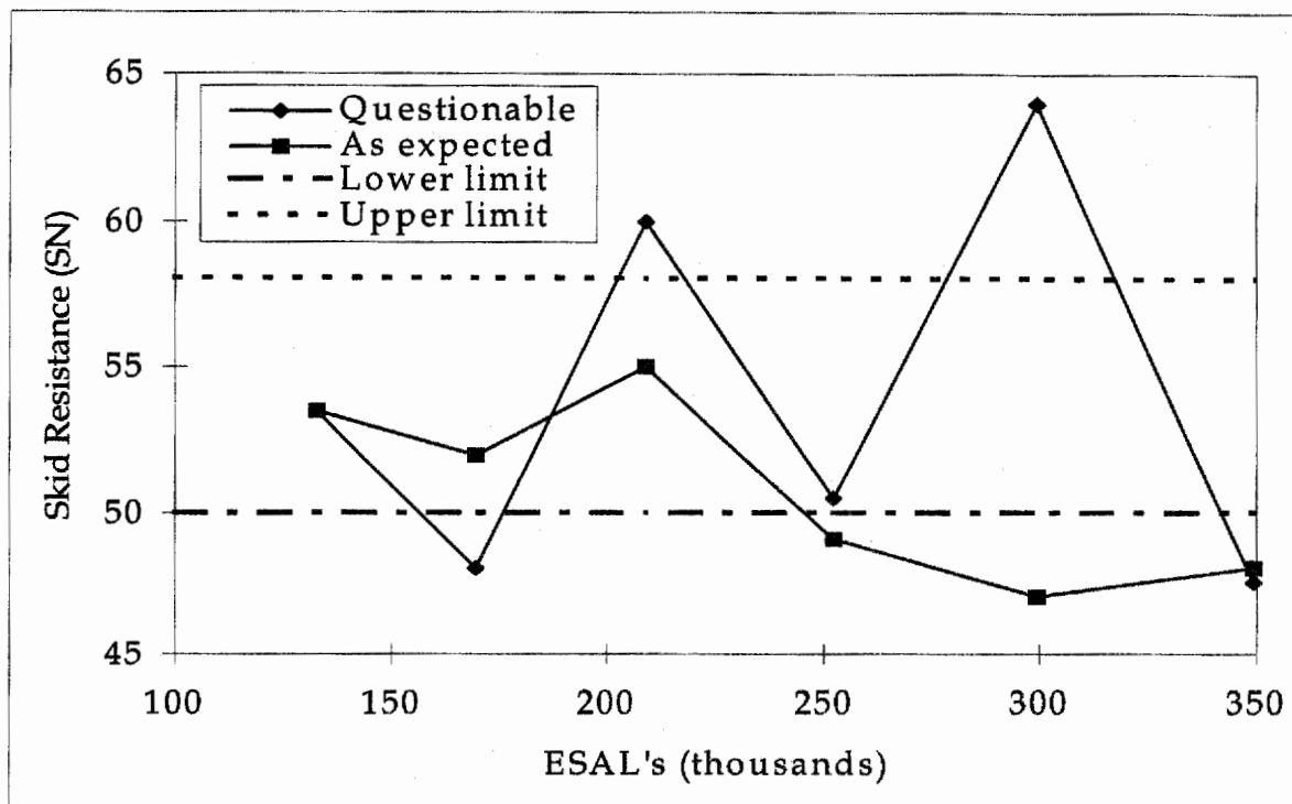
Figure 11. Plot showing time-series friction data with as-expected and not-as-expected data.
