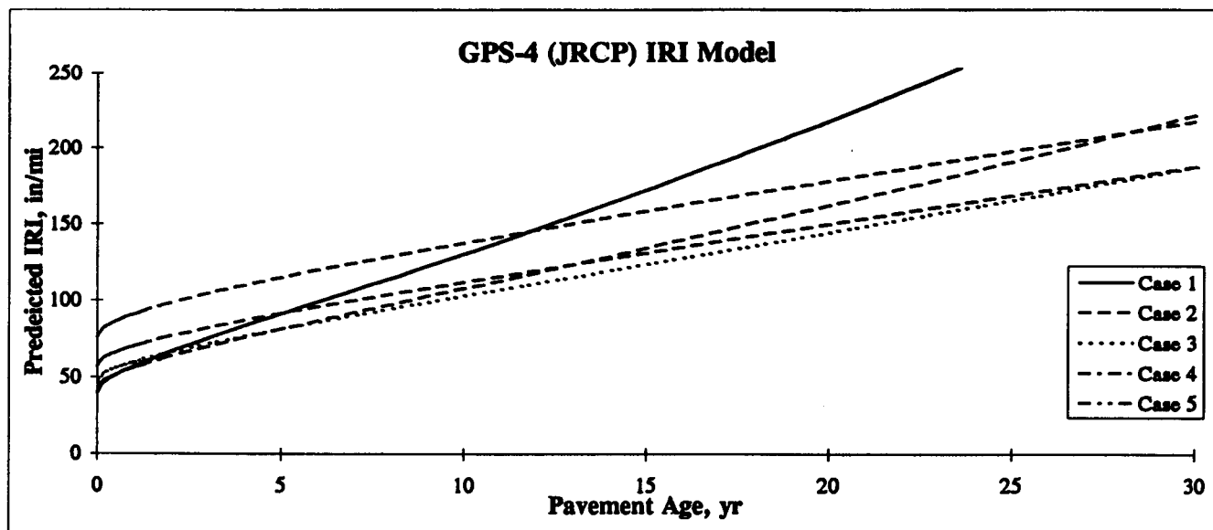
Fig 5.5.3. Sensitivity of GPS-4 IRI model to changes in PCC thickness, holding all other parameters constant.
