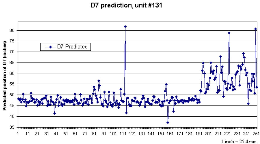
Figure 48. Graph. Predicted position of d7, unit #131, 1994–97.
