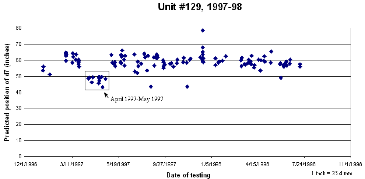
Figure 16. Graph. Predicted position of d7, unit #129, 1997-98.
