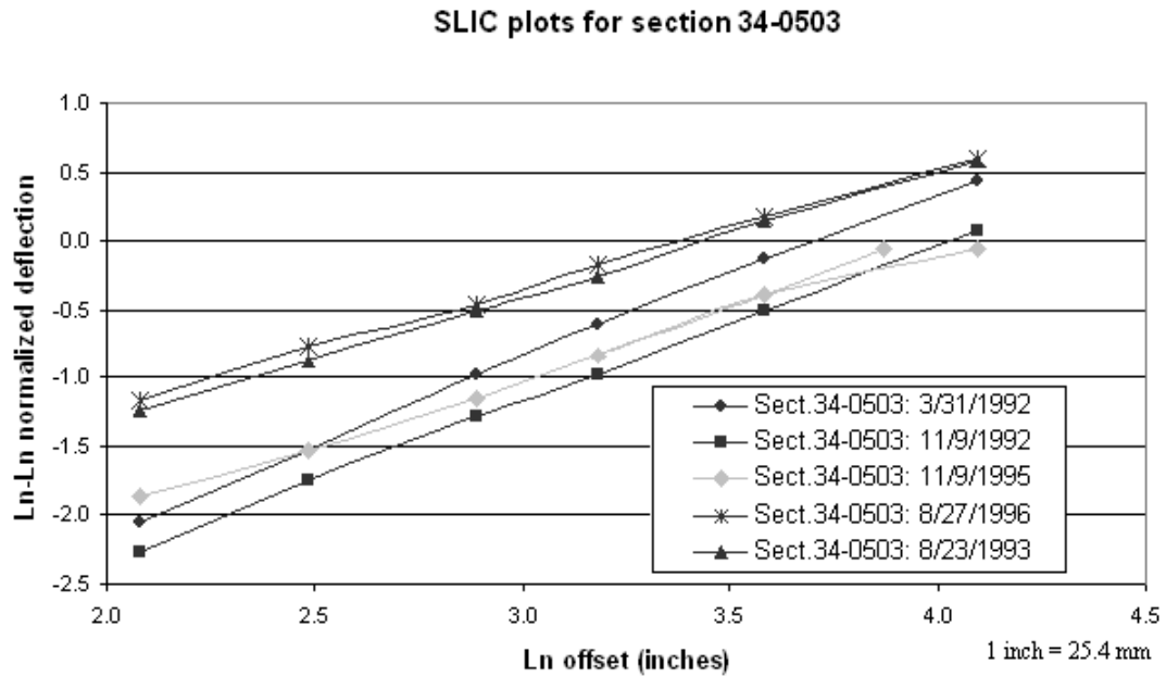
Figure 14. Graph. SLIC plots for section 34-0503 including unit #129, November 1995.
