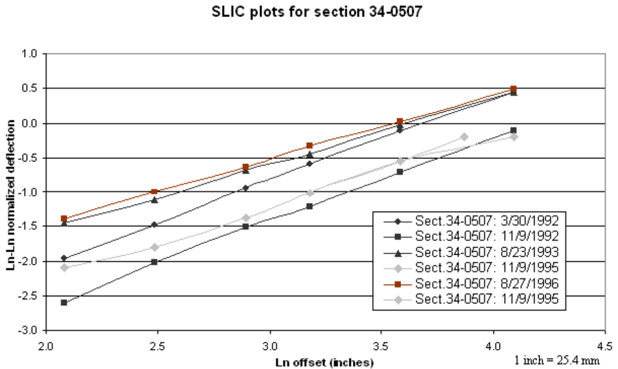
Figure 15. Graph. SLIC plots for section 34-0507 including unit #129, November 1995.
