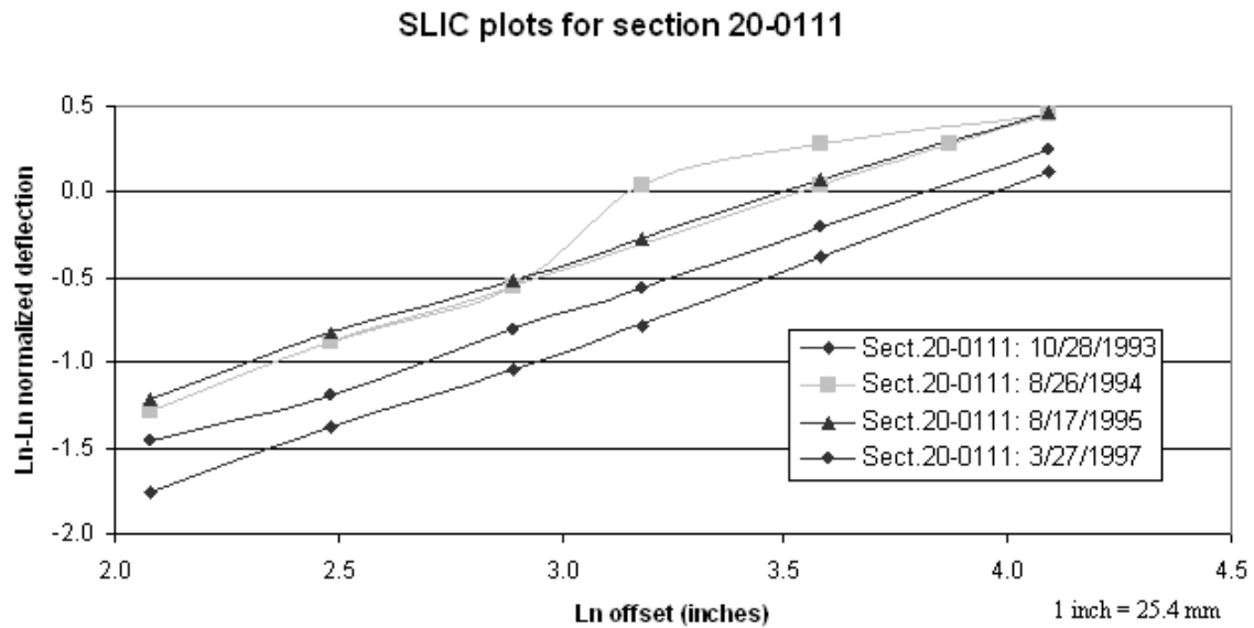
Figure 33. Graph. SLIC plots for section 20–0111 including unit #130, August 1994.
