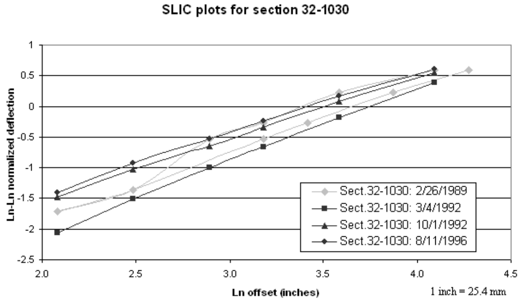
Figure 27. Graph. SLIC plots for section 32–1030 including unit #061, February 1989.
