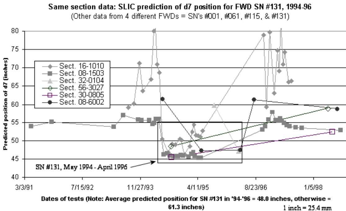
Figure 49. Graph. Same section data for d7 position, four different FWDs.
