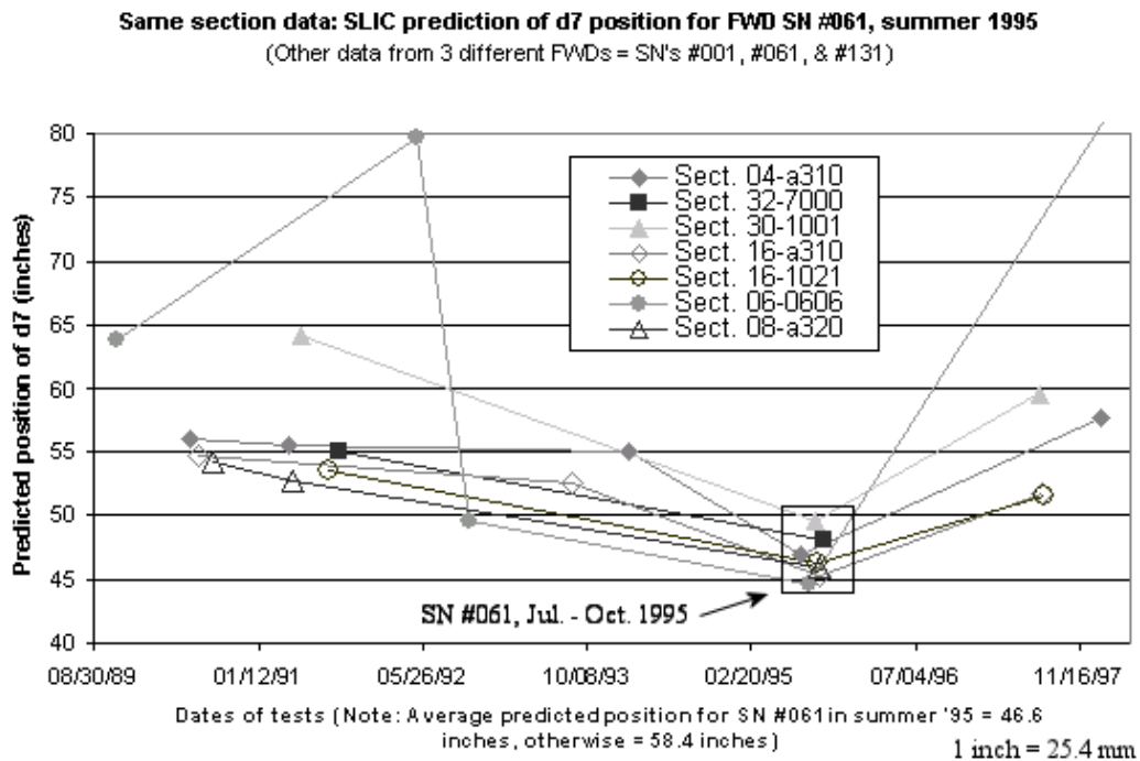
Figure 45. Graph. Same section data for d7 position, three different FWDs.
