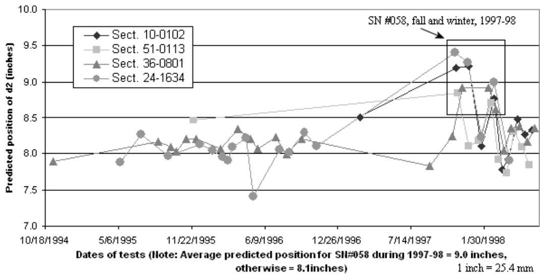
Figure 21. Graph. Same section data for d2 position, two different FWDs.
