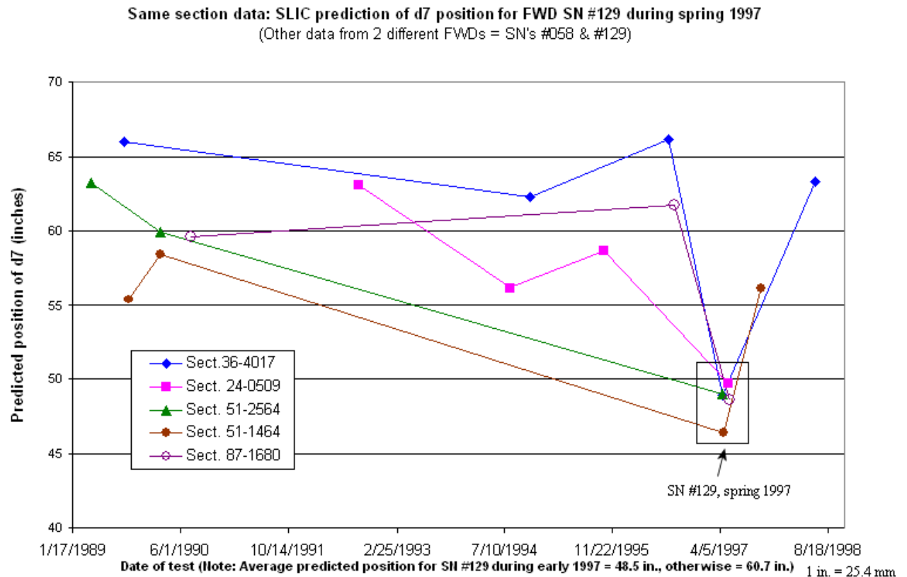
Figure 17. Graph. Same section data for d7 position, two different FWDs.
