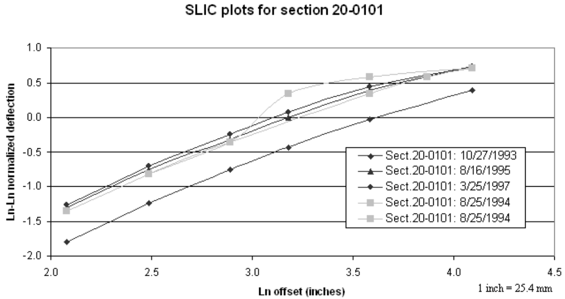
Figure 32. Graph. SLIC plots for section 20–0101 including unit #130, August 1994.
