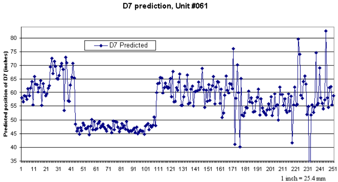
Figure 44. Graph. Predicted position of d7, unit #061, 1994–97.
