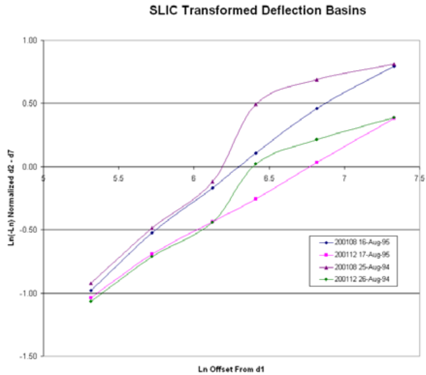
Figure 3. Graph. Sample deflection basins transformed with SLIC (input protocol positions).
