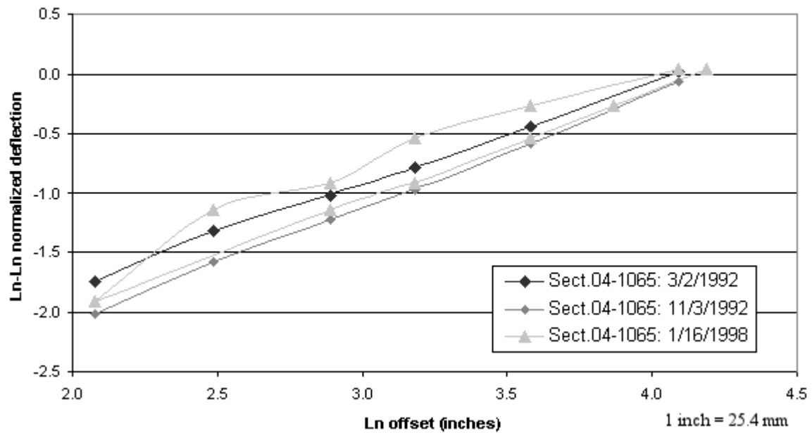
Figure 55. Graph. SLIC plots for section 04-1065 including unit #131, January 1998.
