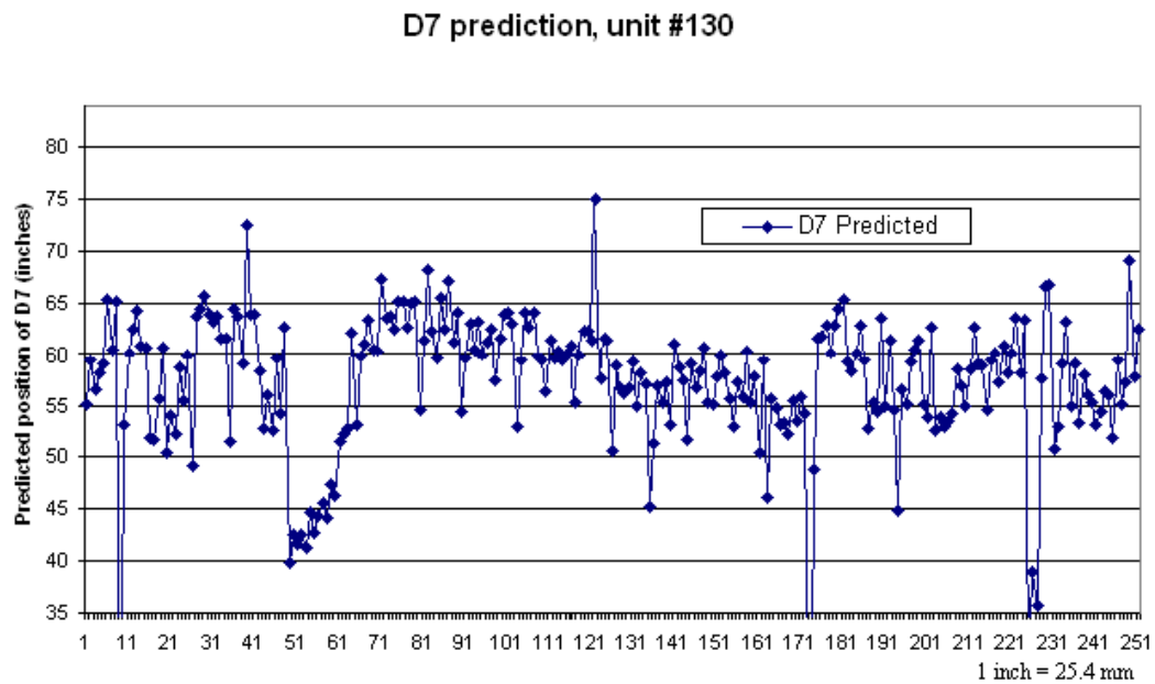
Figure 31. Graph. Predicted position of d7, unit #130, 1994–96.
