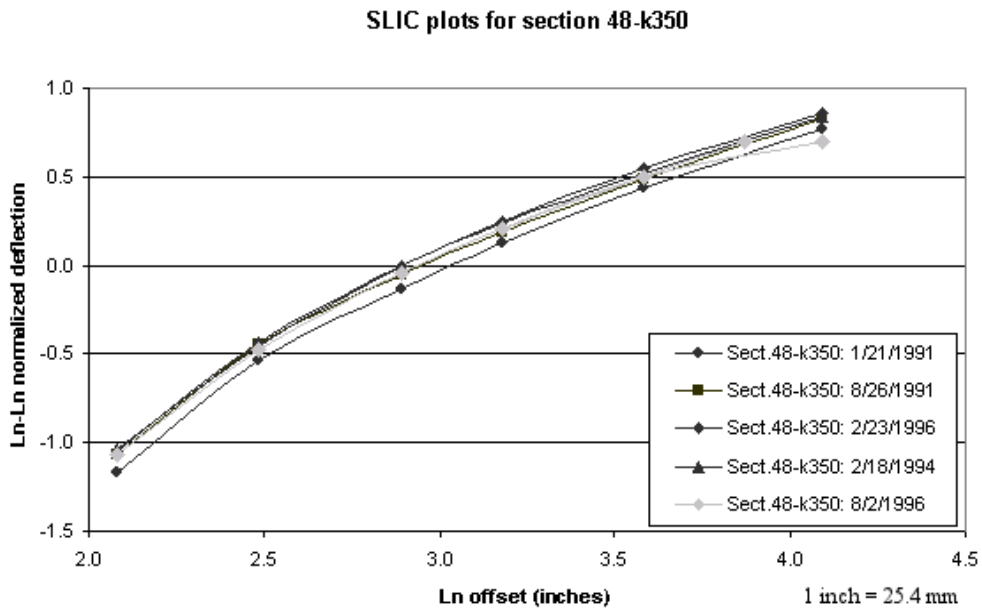
Figure 43. Graph. SLIC plots for section 48-k350 including unit #132, August 1996.
