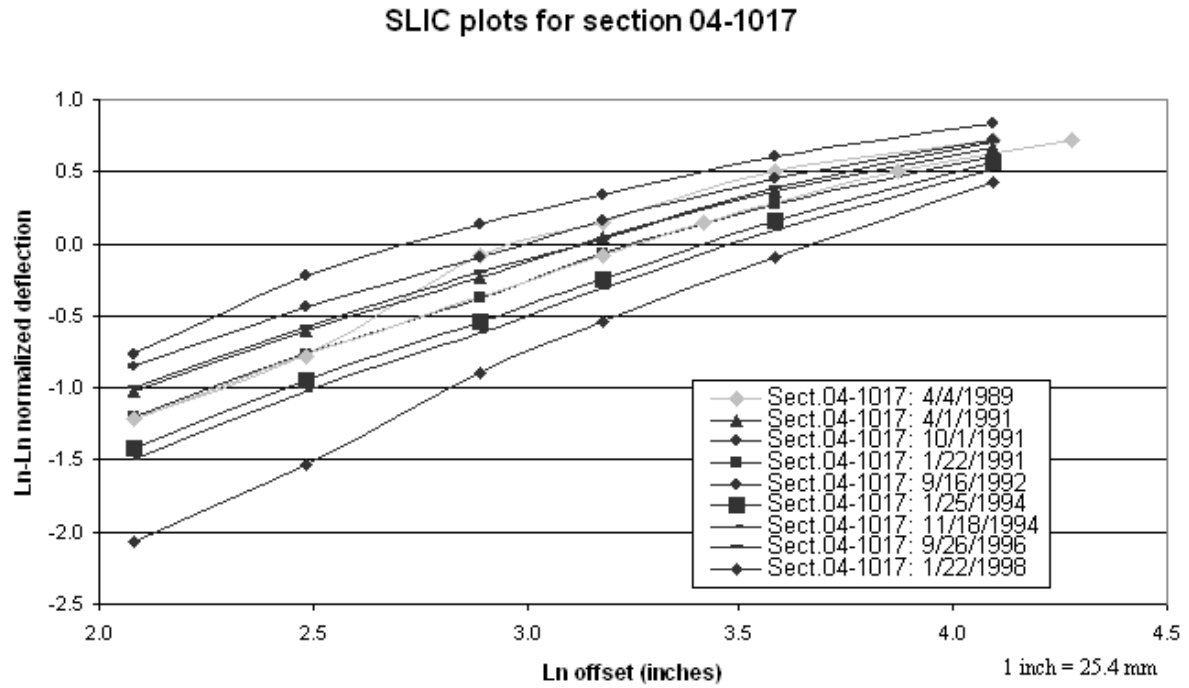
Figure 25. Graph. SLIC plots for section 04–1017 including unit #061, April 1989.
