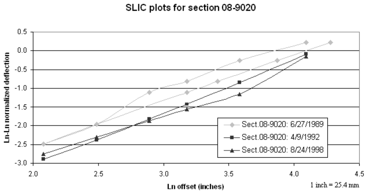
Figure 26. Graph. SLIC plots for section 08–9020 including unit #061, June 1989.
