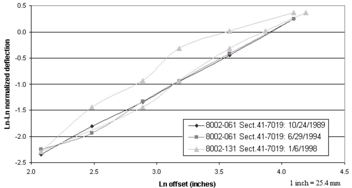
Figure 54. Graph. SLIC plots for section 41-7019 including unit #131, January 1998.
