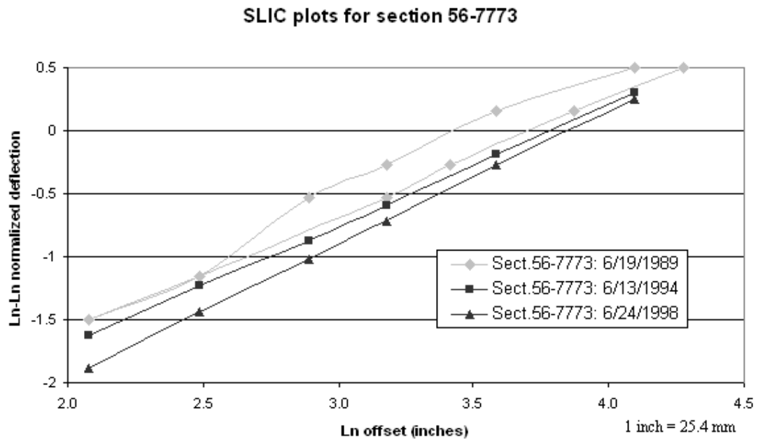
Figure 29. Graph. SLIC plots for section 56–7773 including unit #061, June 1989.
