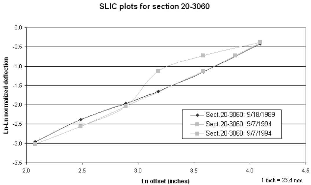
Figure 34. Graph. SLIC plots for section 20–3060 including unit #061, September 1994.
