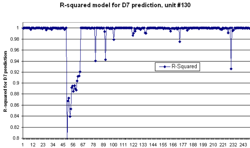
Figure 30. Graph. R^2 model for d7 prediction, unit #130, 1994–96.
