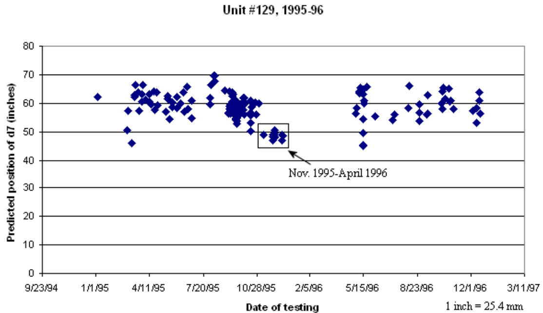
Figure 12. Graph. Predicted position of d7, unit #129, 1995-96.
