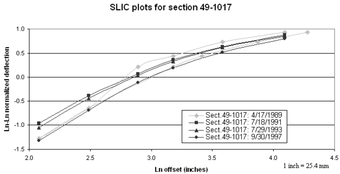
Figure 28. Graph. SLIC plots for section 49–1017 including unit #061, April 1989.
