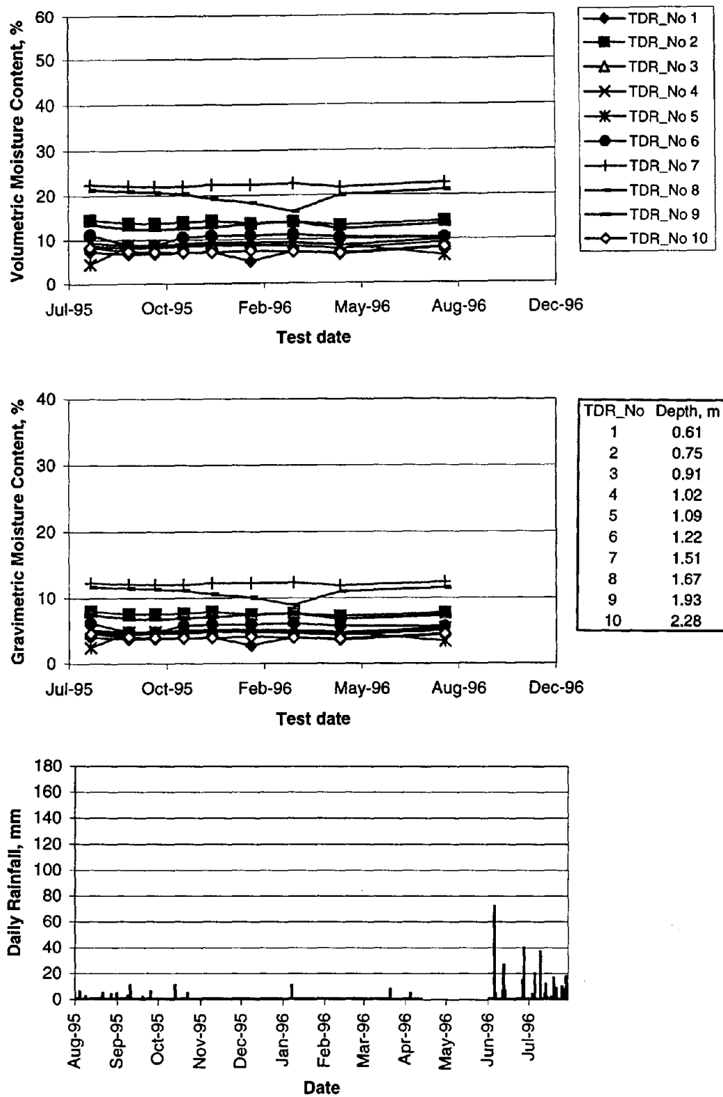
Figure 104. Seasonal variation in volumetric and gravimetric moisture content and daily rainfall for section 313018 in Nebraska.
