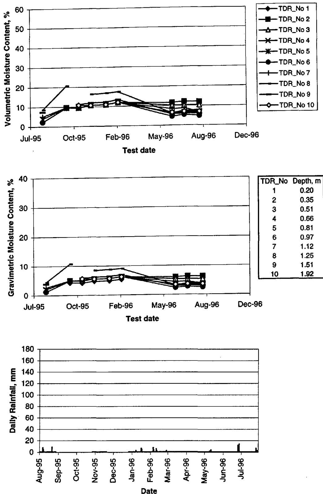
Figure 81. Seasonal variation in volumetric and gravimetric moisture content and daily rainfall for section 040113 in Arizona.
