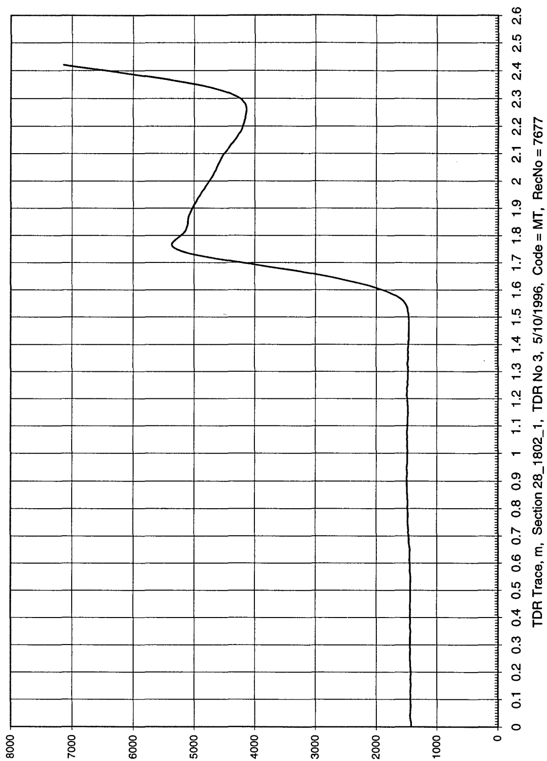
Figure 79. TDR trace 24 for precision and bias study.
