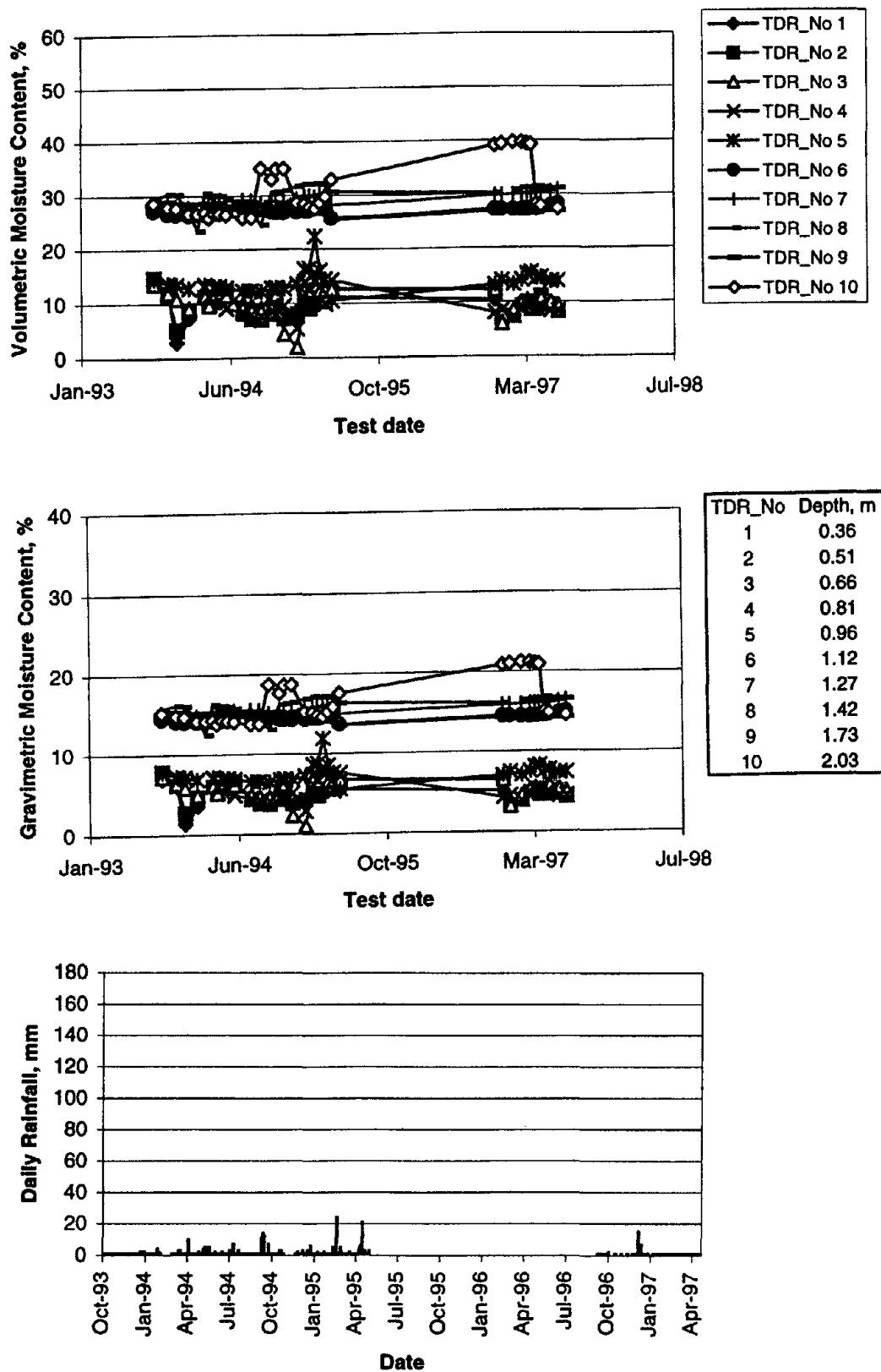
Figure 91. Seasonal variation in volumetric and gravimetric moisture content and daily rainfall for section 161010 in Idaho.
