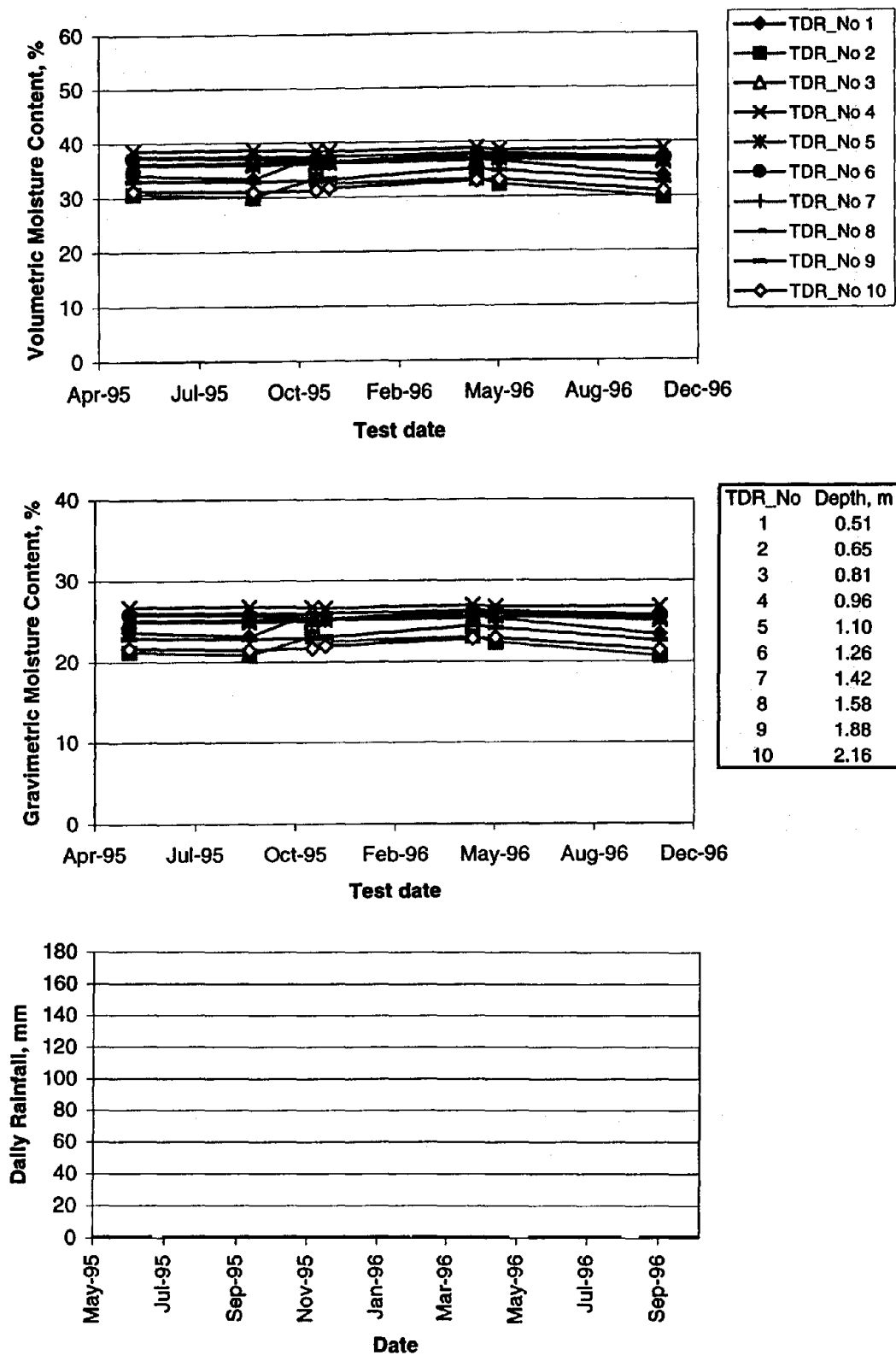
Figure 109. Seasonal variation in volumetric and gravimetric moisture content and daily rainfall for section 370205 in North Carolina.
