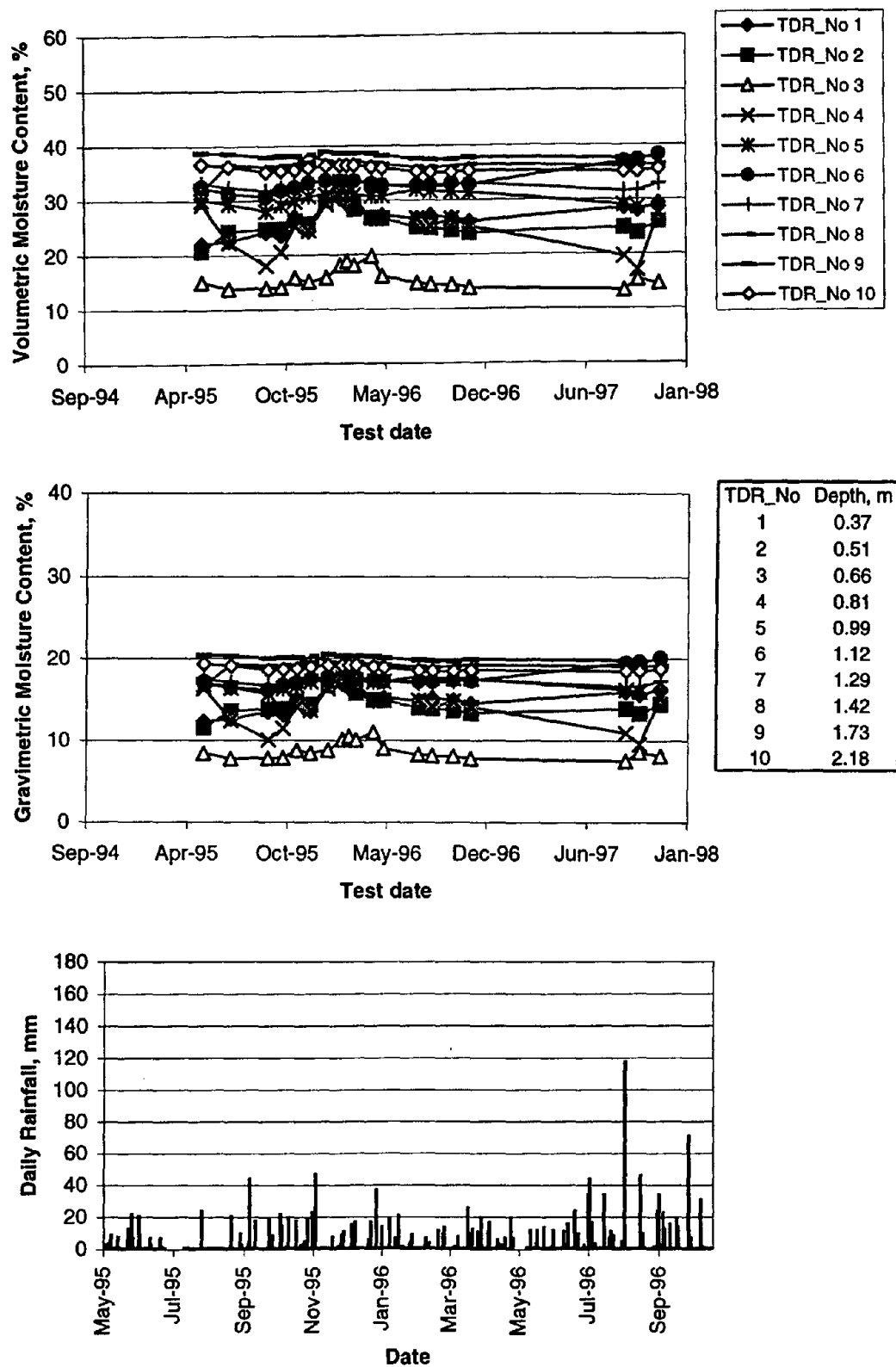
Figure 95. Seasonal variation in volumetric and gravimetric moisture content and daily rainfall for section 241634 in Maryland.
