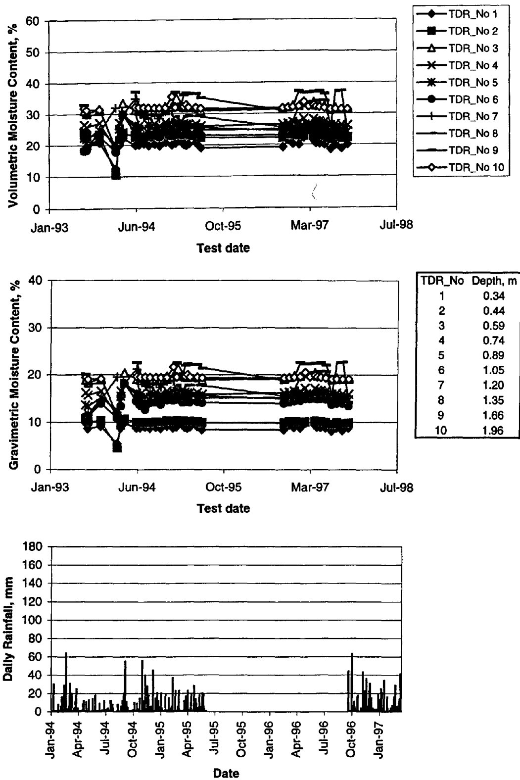
Figure 87. Seasonal variation in volumetric and gravimetric moisture content and daily rainfall for section 091803 in Connecticut.
