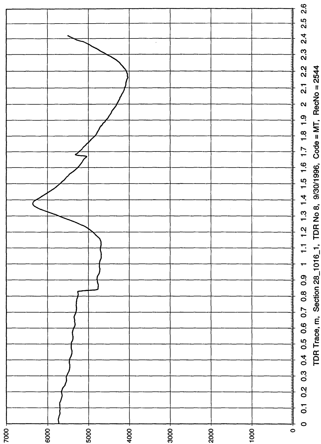
Figure 77. TDR trace 22 for precision and bias study.
