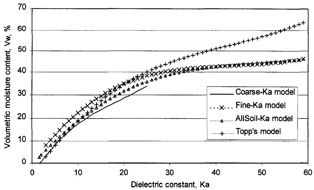
Figure 24. Comparison of various volumetric moisture content models.
