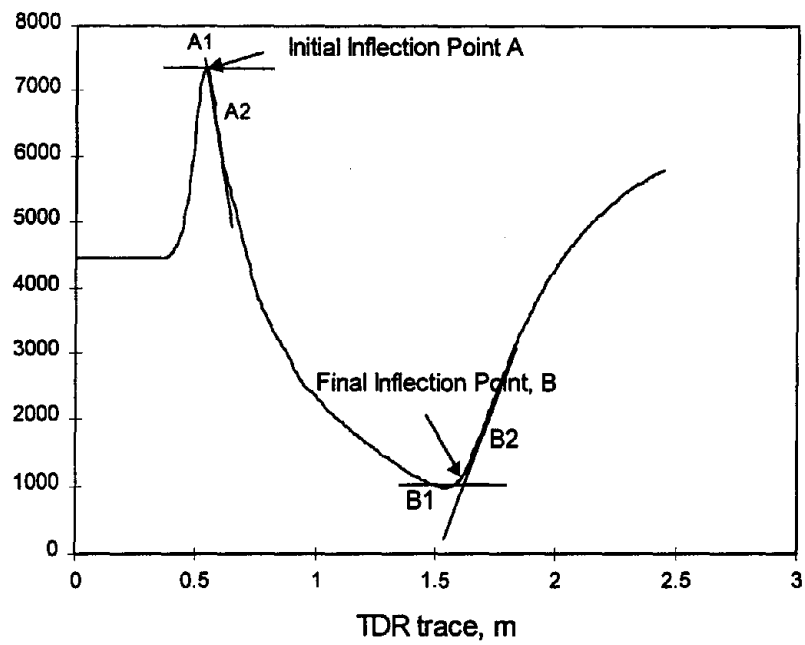
Figure 5. Illustration of the Method of Tangents (section 510113).
