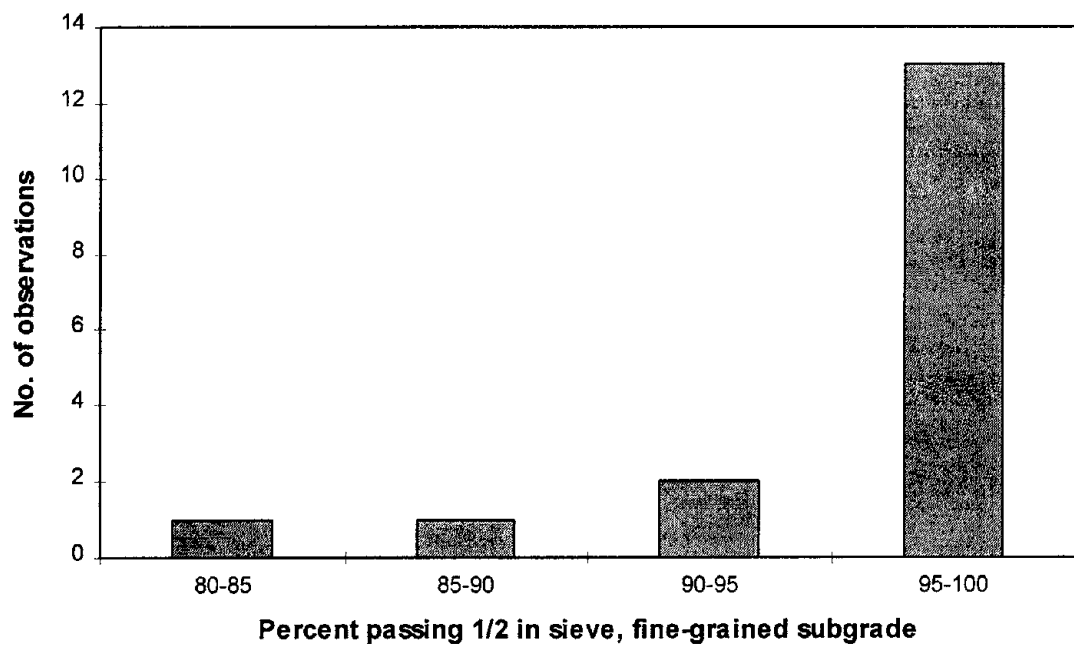
Figure 50. Frequency distribution of percent passing the ½-in sieve for SMP sites, fine-grained soils.
