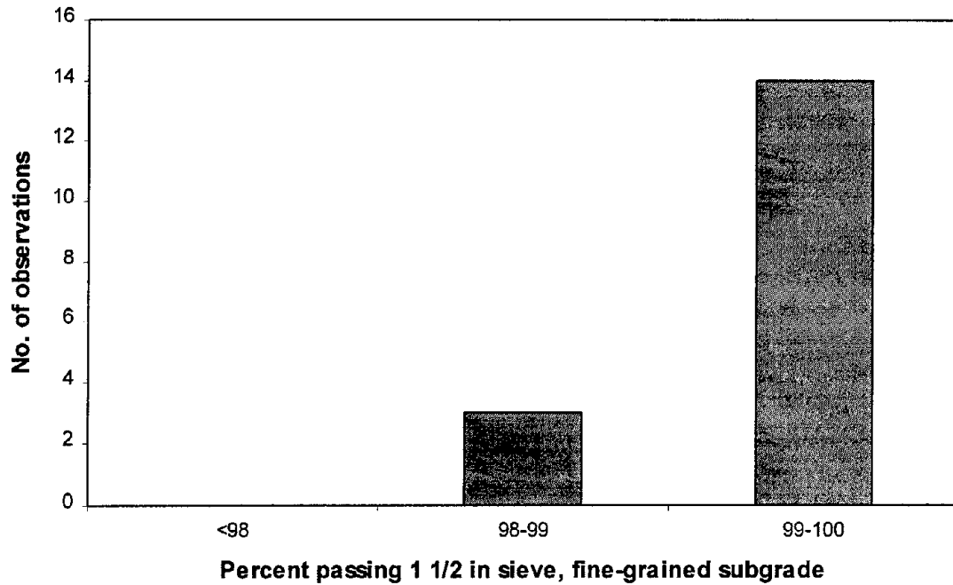
Figure 49. Frequency distribution of percent passing the 1½-in sieve for SMP sites, fine-grained soils.
