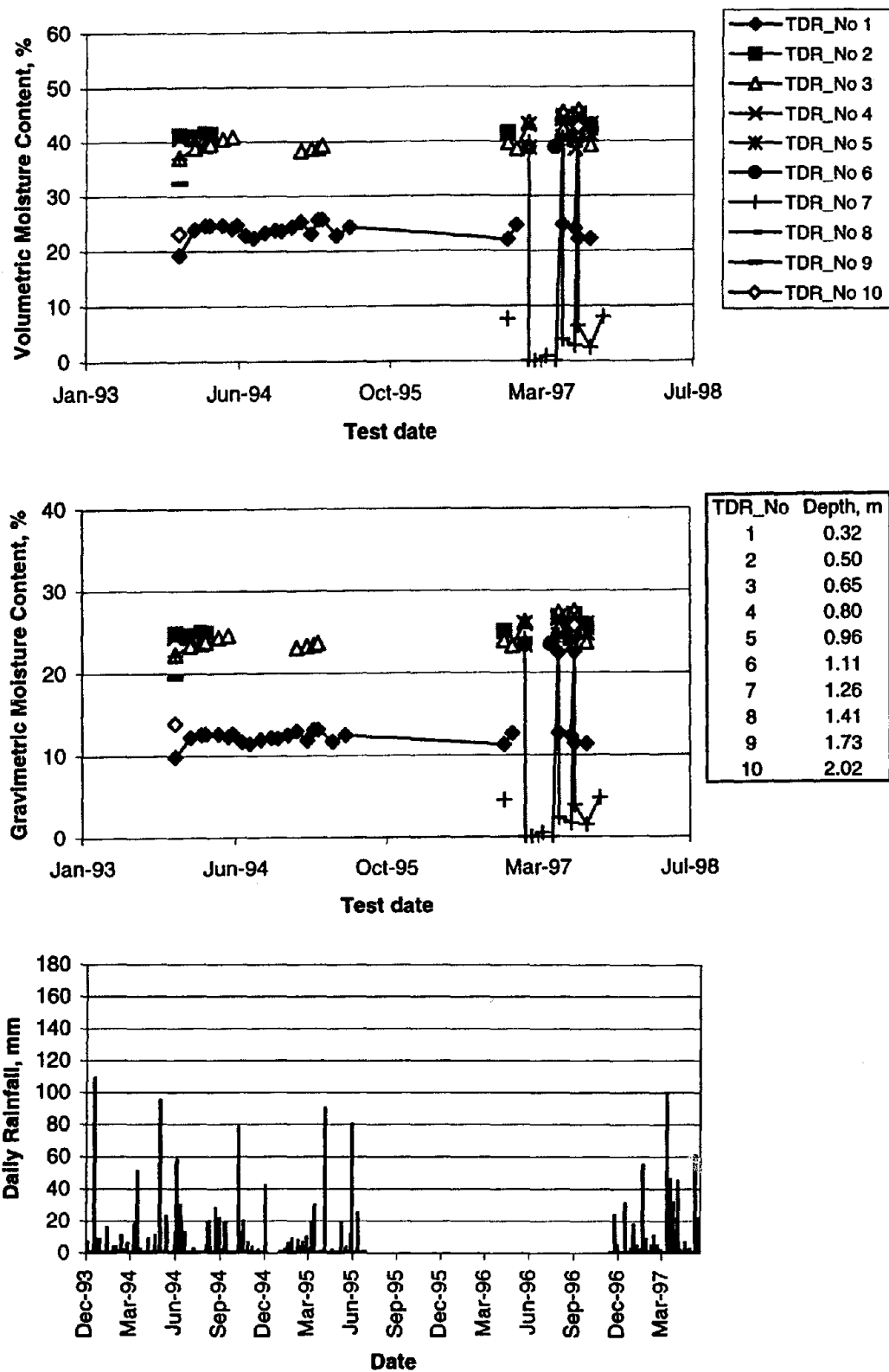
Figure 117. Seasonal variation in volumetric and gravimetric moisture content and daily rainfall for section 481060 in Texas.
