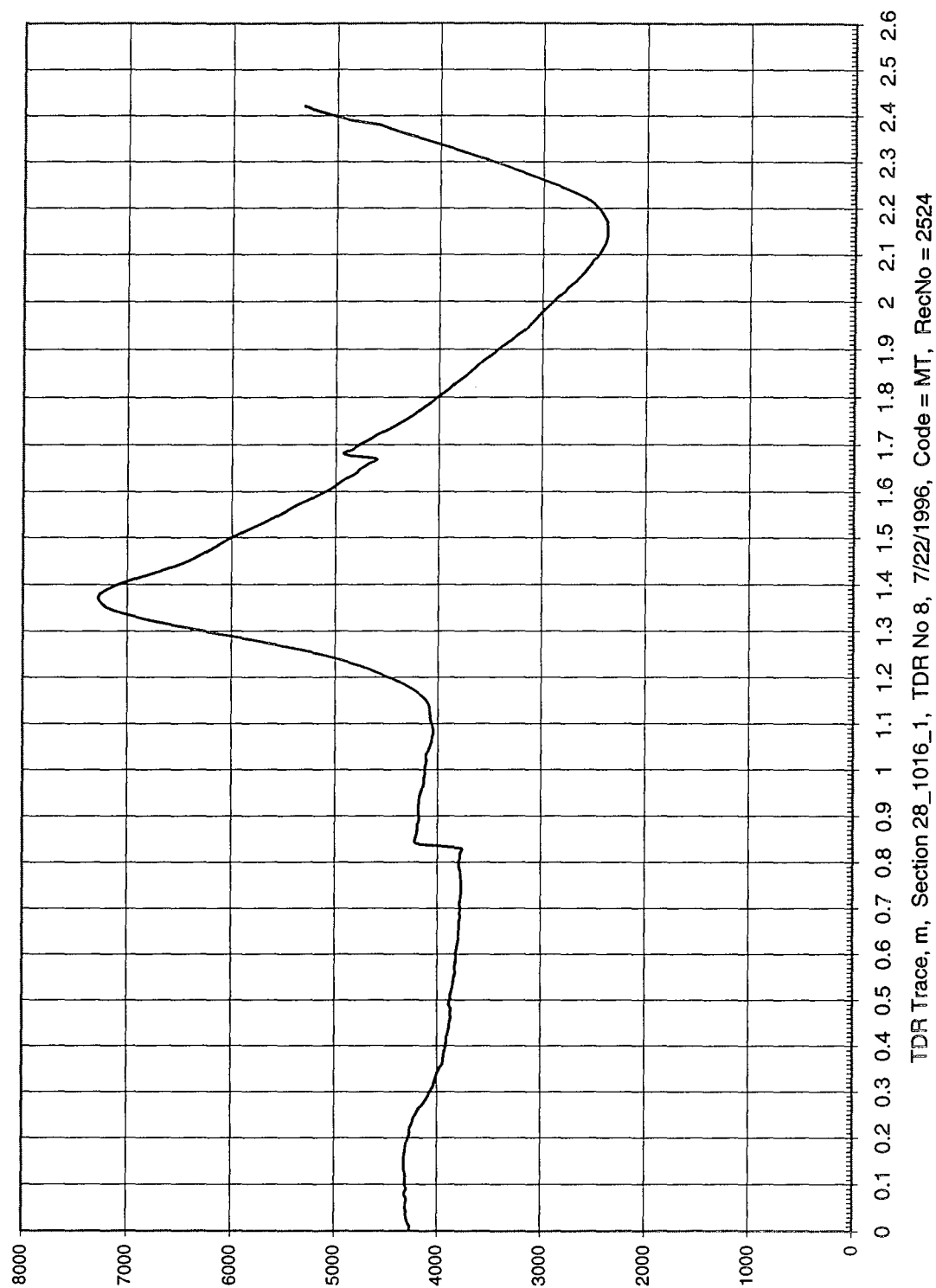
Figure 76. TDR trace 21 for precision and bias study.
