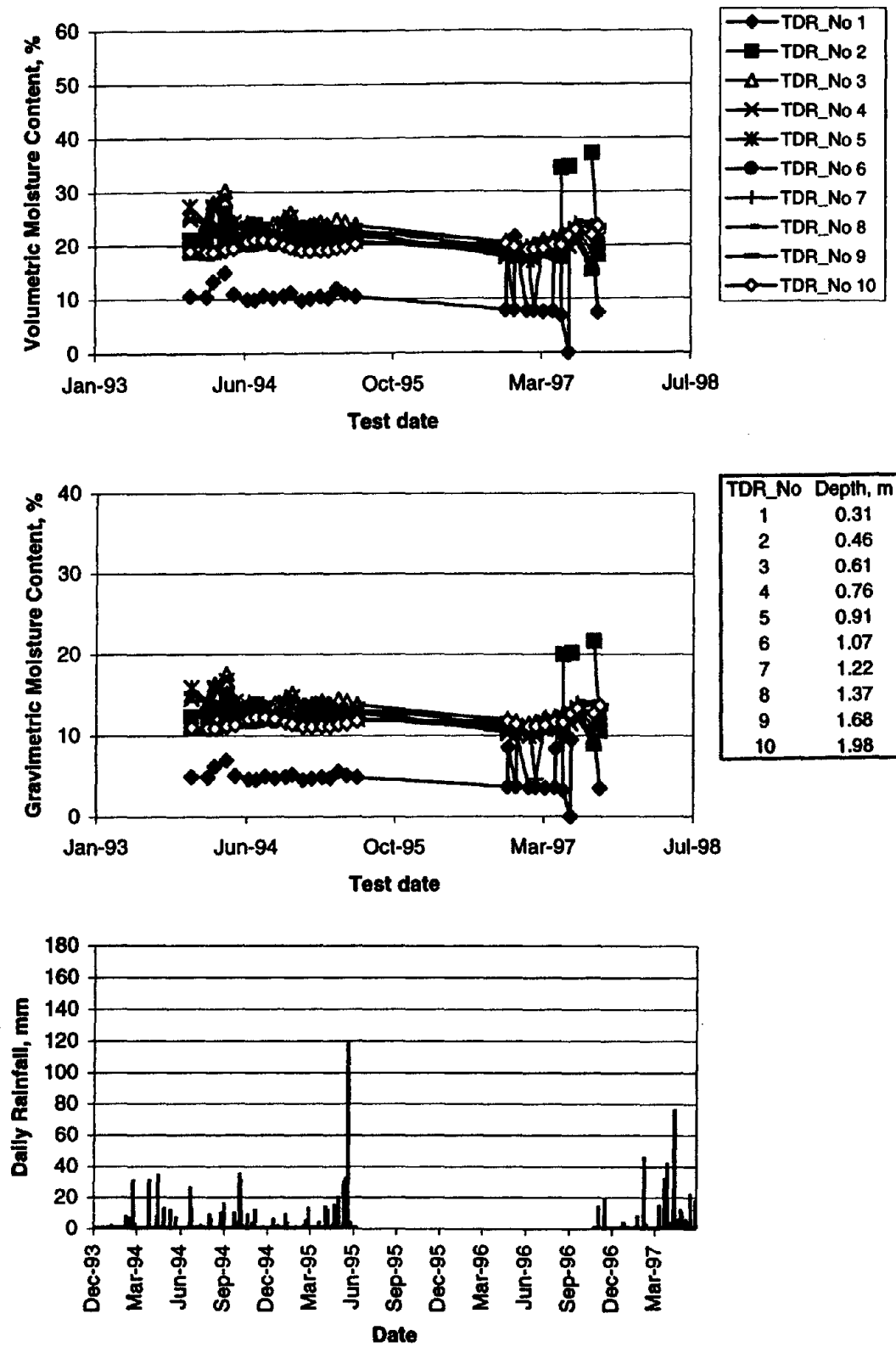
Figure 119. Seasonal variation in volumetric and gravimetric moisture content and daily rainfall for section 481077 in Texas.
