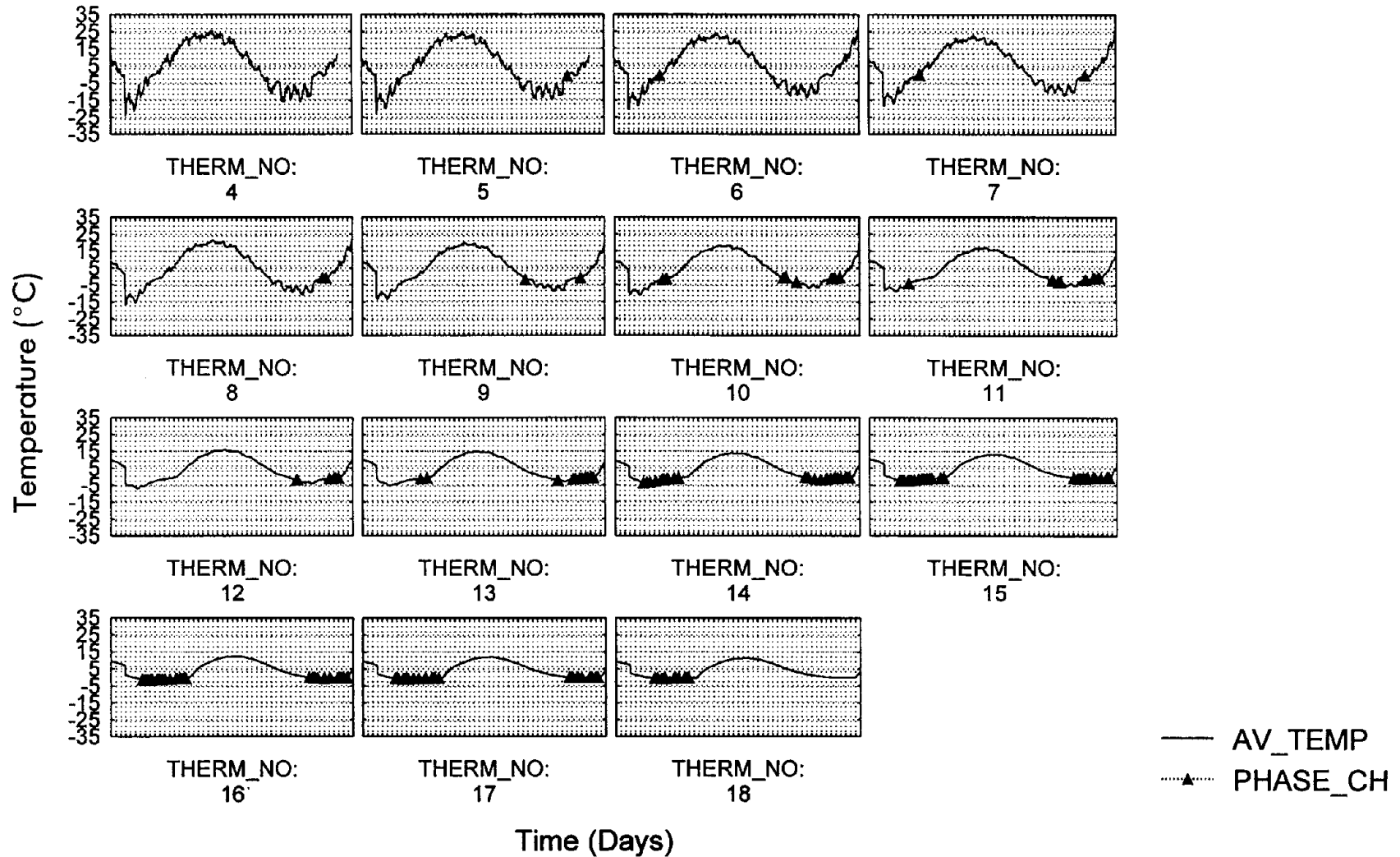
Figure 3. Phase change events using latent heat of fusion.
