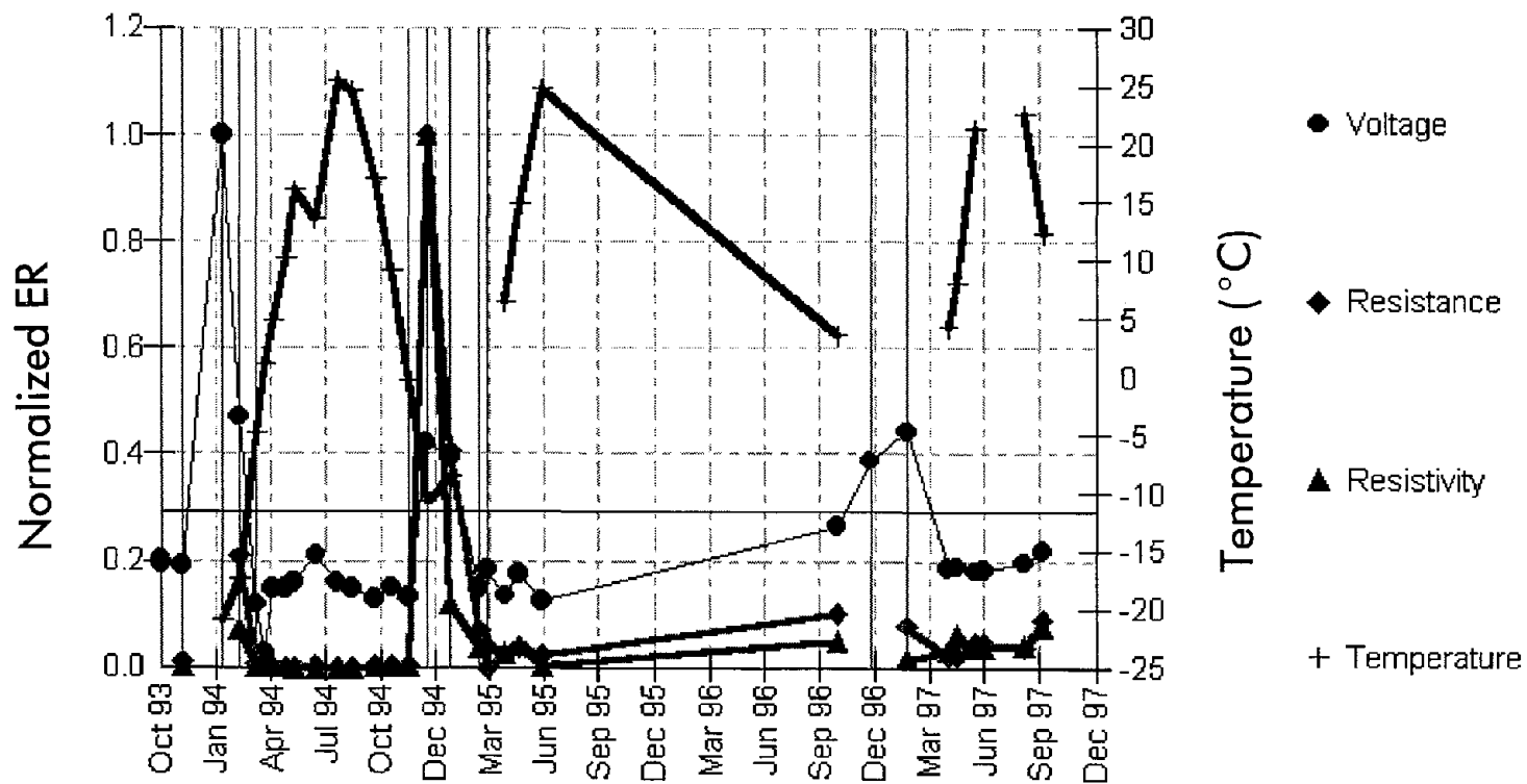
Figure 6. Example ER time-series graph produced by FROST.
