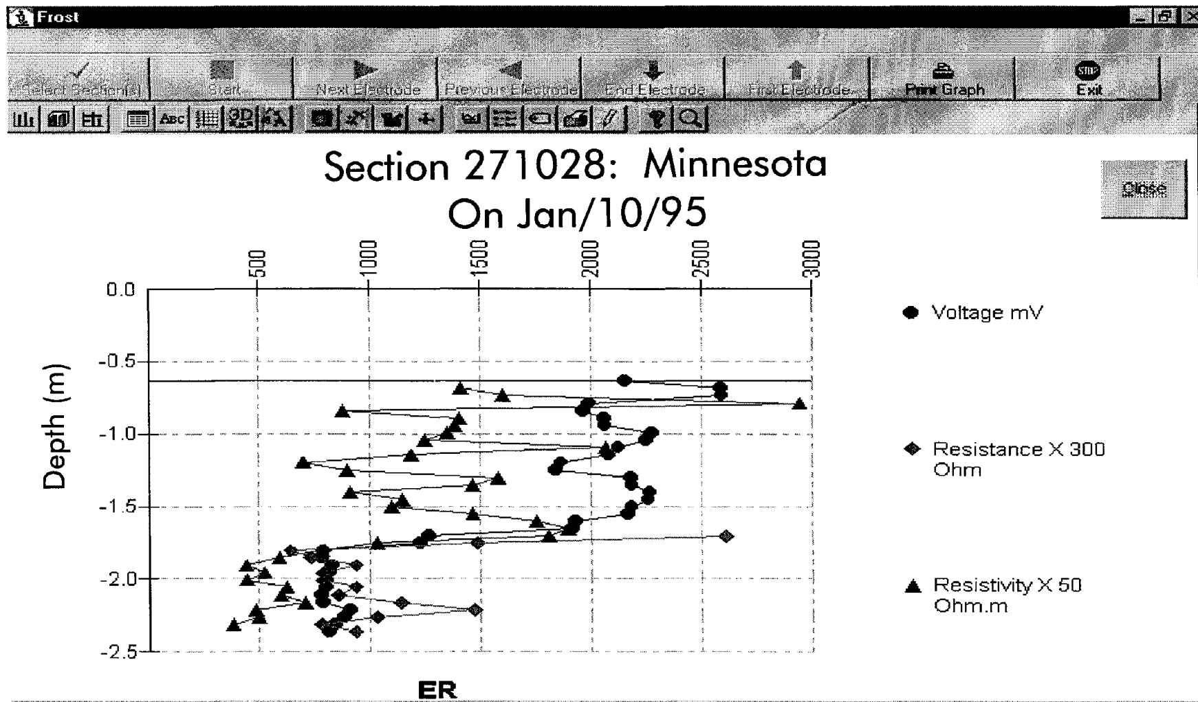
Figure 8. Example ER versus depth plot produced by FROST.
