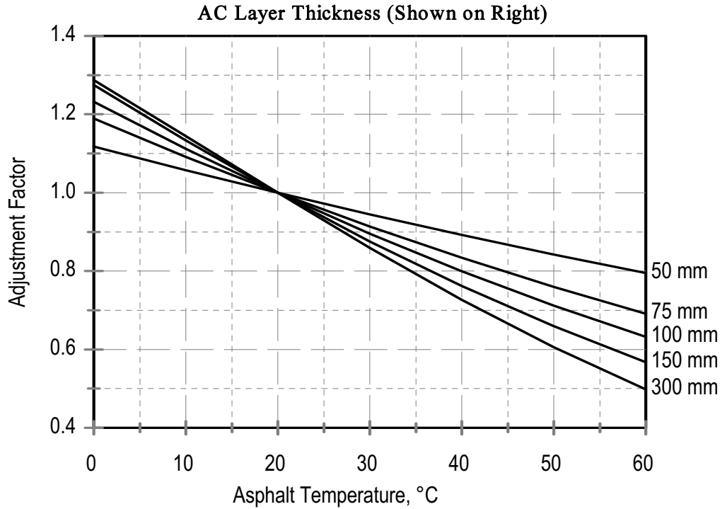
Figure 26. FWD temperature adjustment factors for defl36 = 100 \mu\text{m} and 40° latitude.
