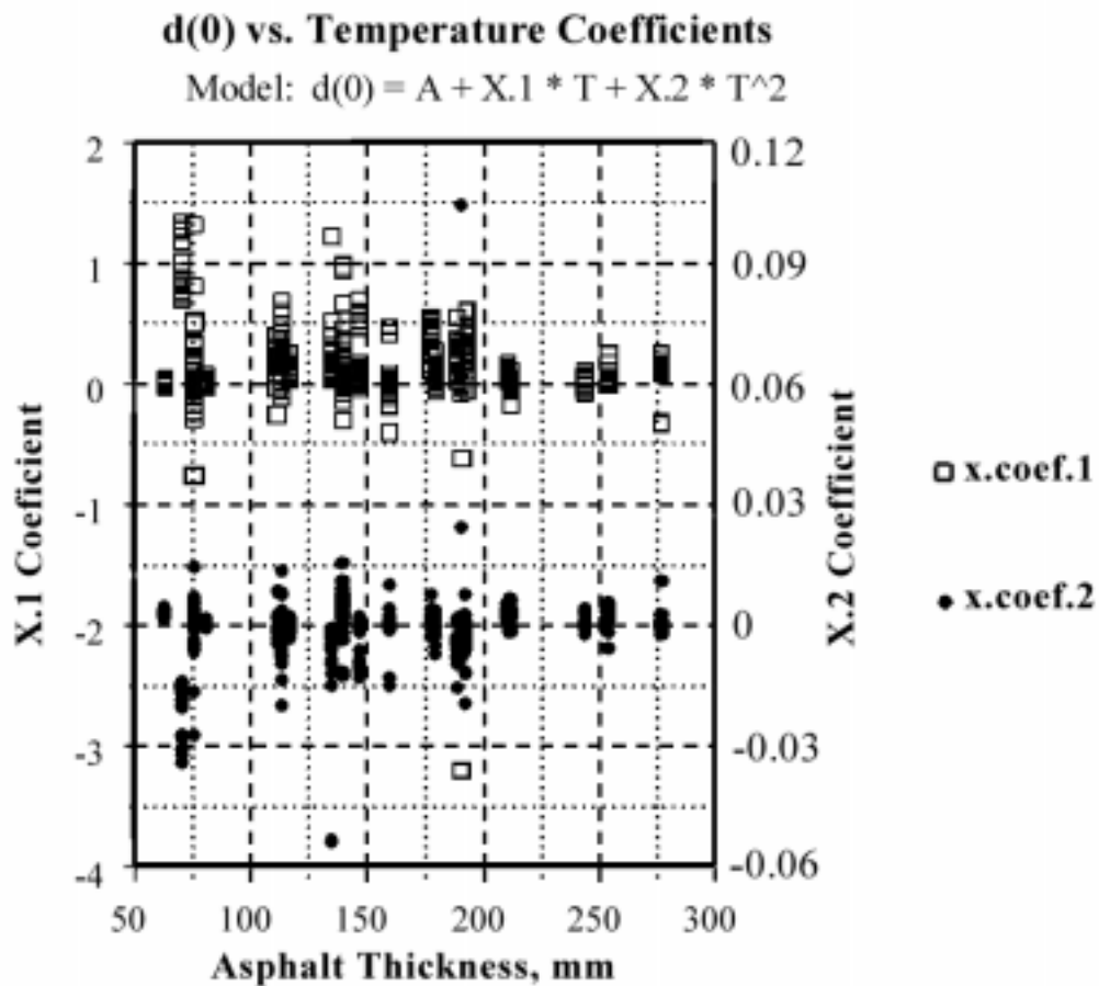
Figure 24. Temperature versus deflection coefficients.
