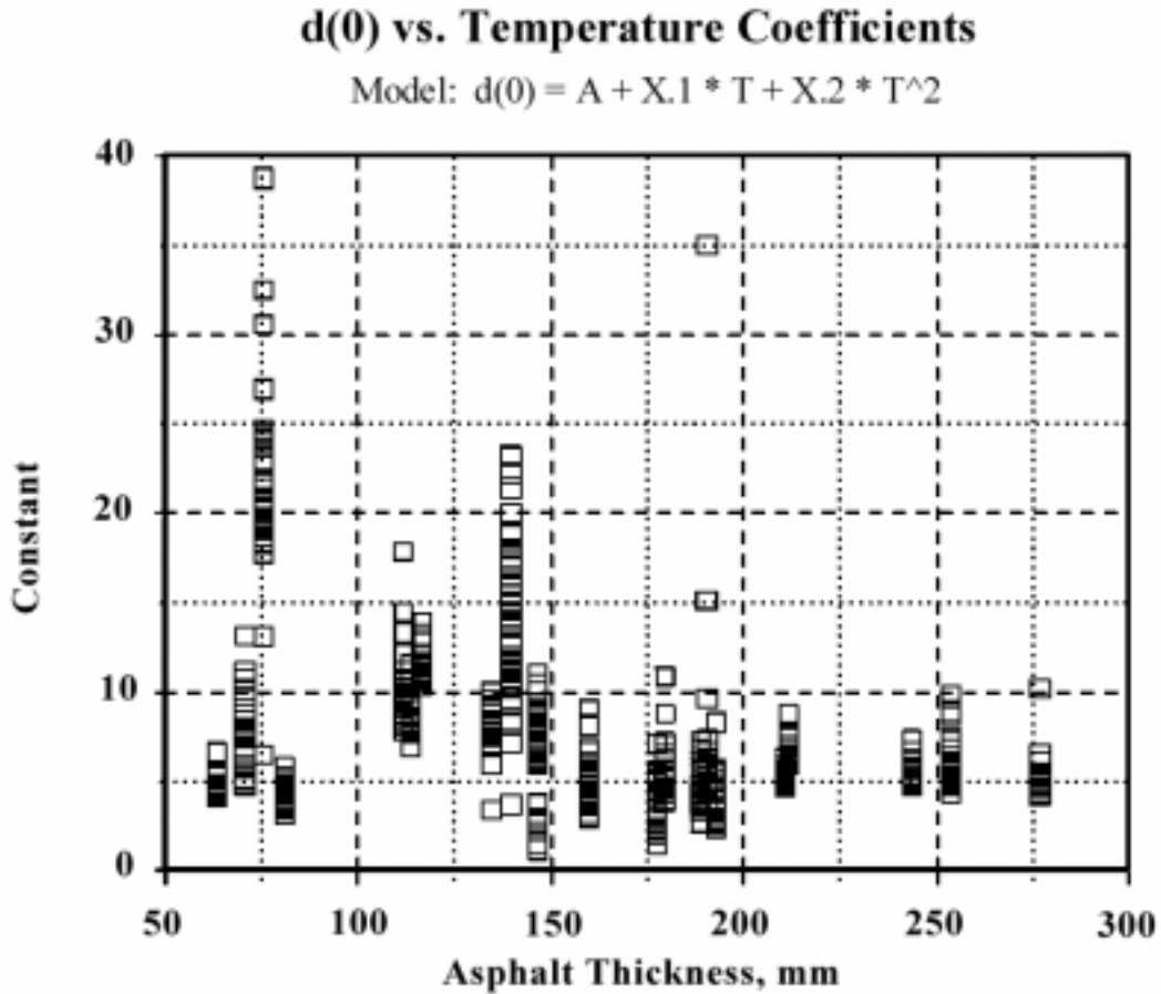
Figure 25. Intercept of temperature versus deflection regressions.
