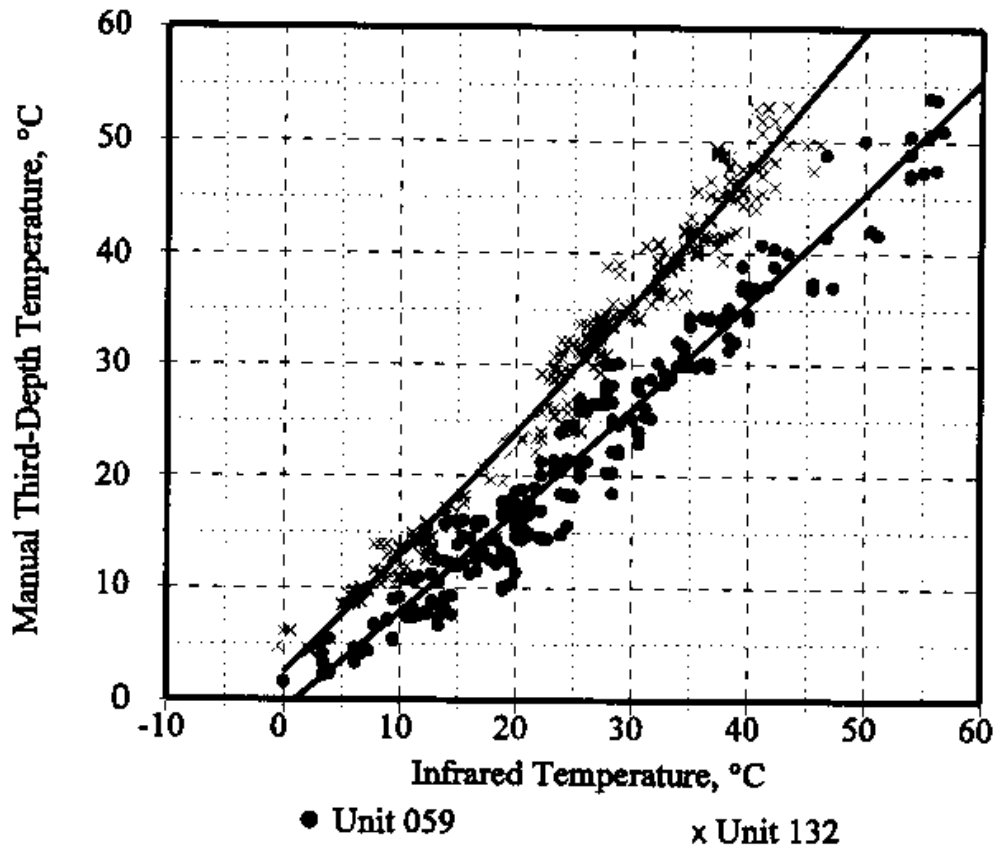
Figure 8. Comparison of two infrared sensors used on the same sites.
