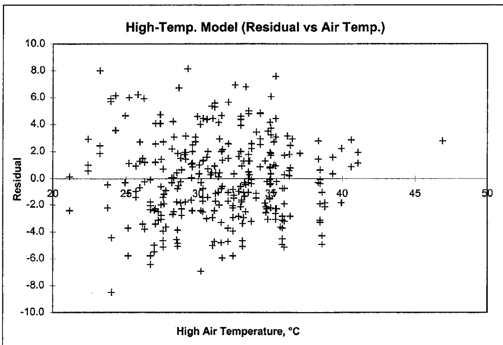
Figure 28 - Residual of High-Temperature Model Versus High Air Temperature.
