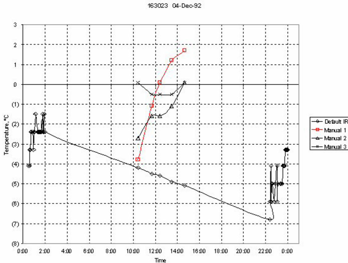
Figure 10. Graph. Time-temperature plot showing 12-hour computer time error.
