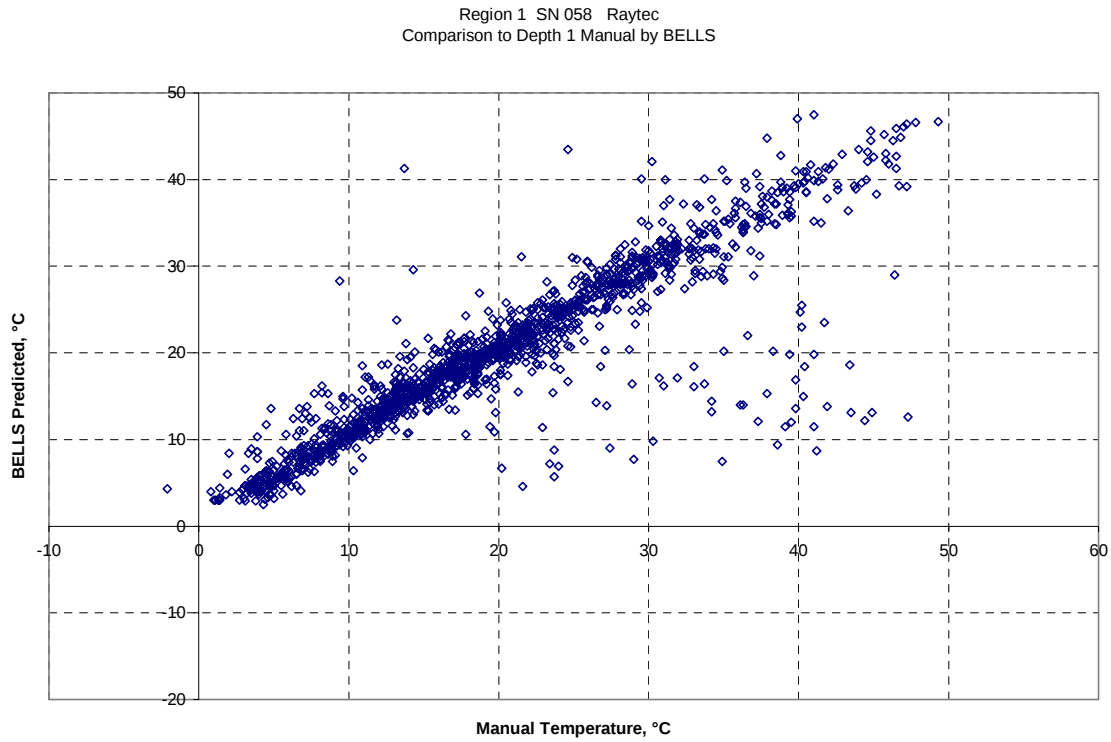
Figure 13. Graph. Manual 1 and BELLS2 compared (before data cleaning; all surfaces).
