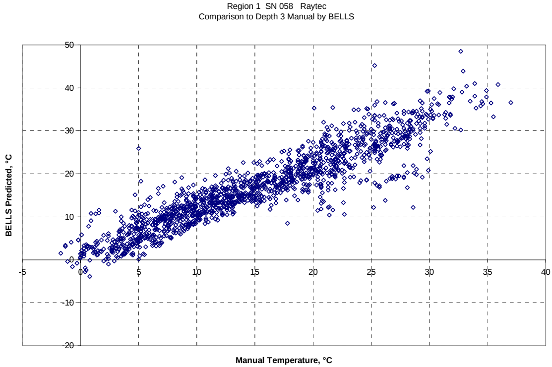
Figure 14. Graph. Manual 3 and BELLS2 compared (before data cleaning; all surfaces).
