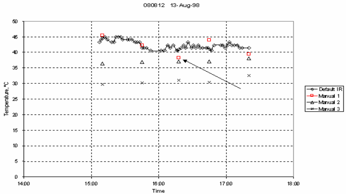
Figure 12. Graph. Minimum detectable error possible by visual scan.
