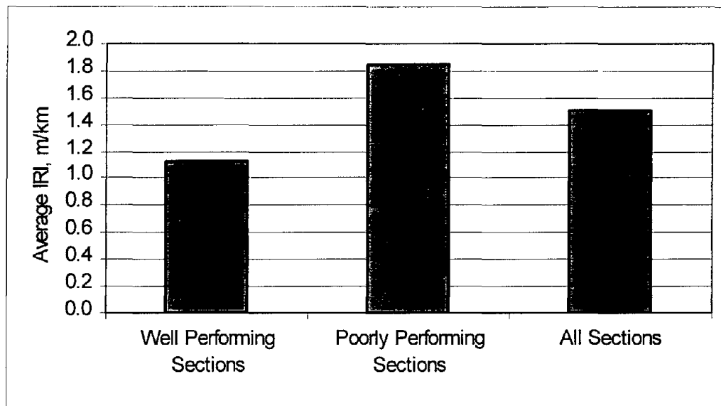
Figure 44. Comparison of IRI values.
