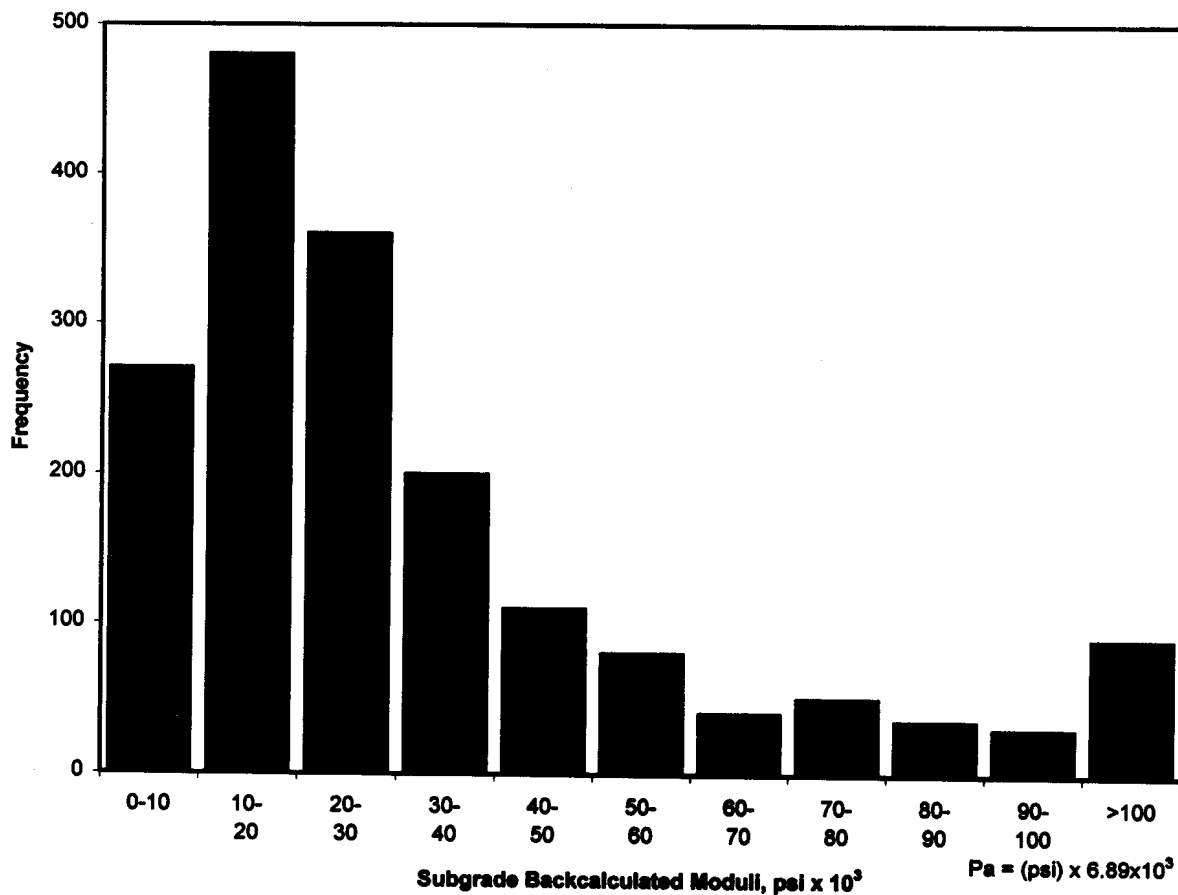
Figure 16. Histogram of backcalculated subgrade layer moduli for the revised results.
