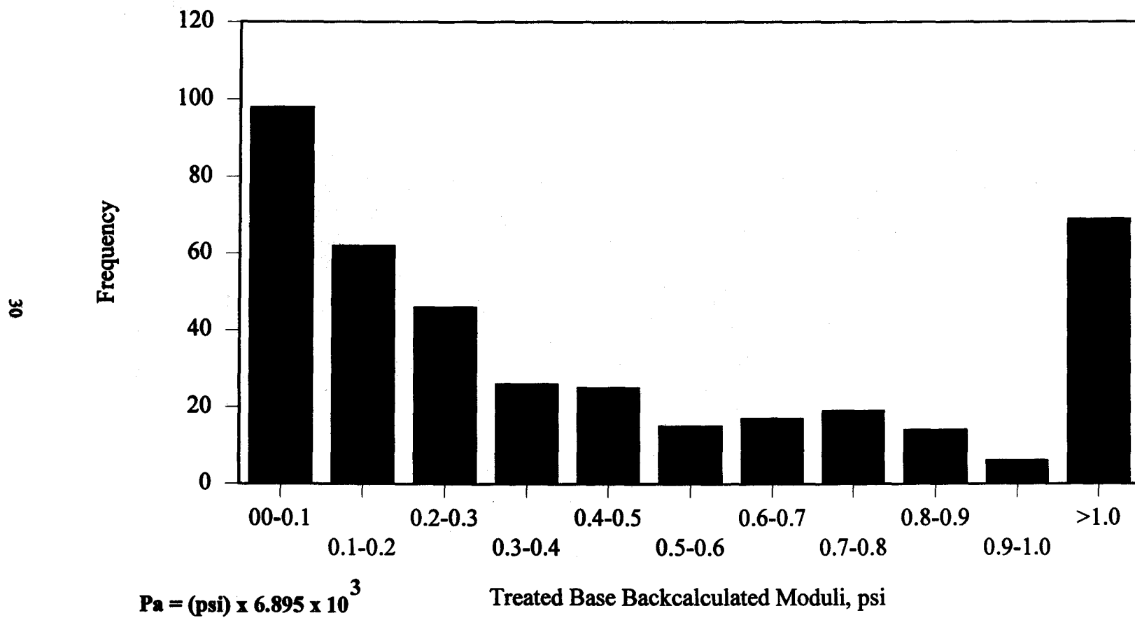
Figure 12. Histogram of backcalculated treated base layer moduli for the revised results.
