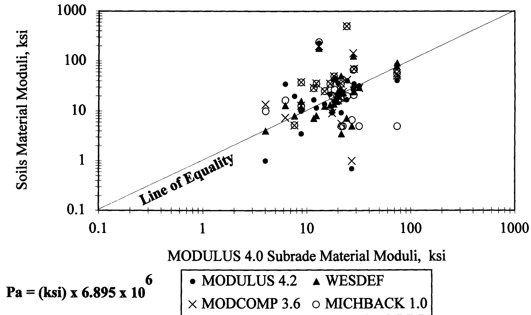
Figure 3. Comparison of calculated layer moduli with different programs to the results from Modulus 4.0 for subgrade soils.
